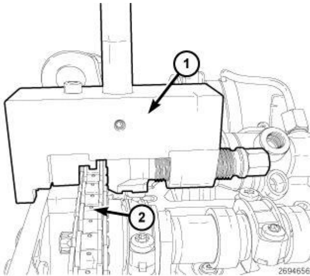
Fig. 586: Installing Rivet Press Tool Onto Timing Chain Courtesy of CHRYSLER LLC
