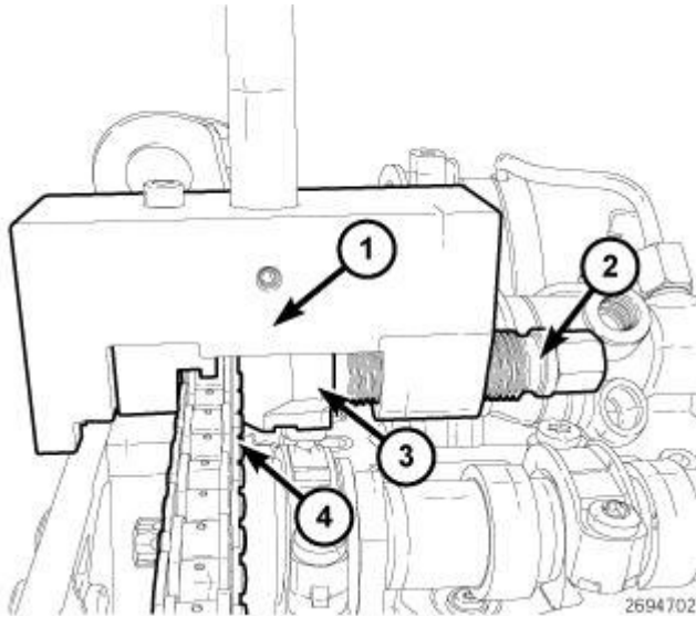
Fig. 588: Riveting Press Tool, Timing Chain Thrust Spindle, Thrust Piece & Timing Chain Courtesy of CHRYSLER LLC
