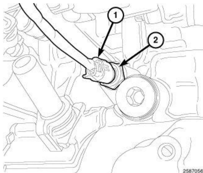
Fig. 349: Oil Temperature Sensor Harness Connector & Sensor
