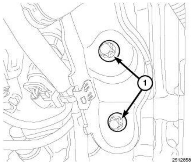
Fig. 614: EGR Support Bracket Bolts Courtesy of CHRYSLER LLC
