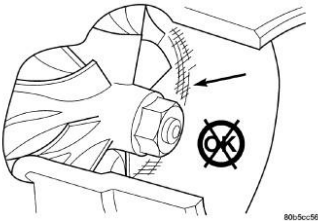
Fig. 573: Inspect Compressor Housing For Impeller Rubbing Condition Courtesy of CHRYSLER LLC
