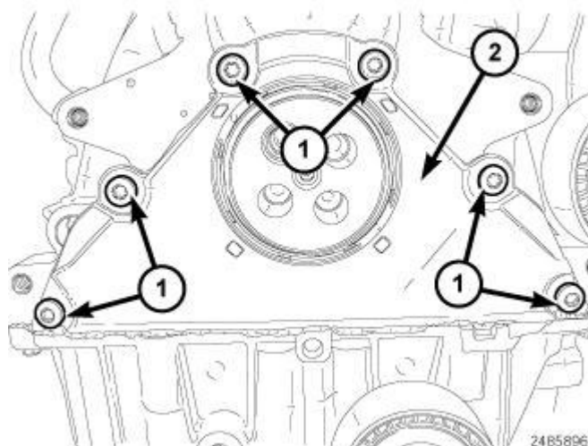
Fig. 238: Front Oil Seal Carrier & Bolts Courtesy of CHRYSLER LLC
