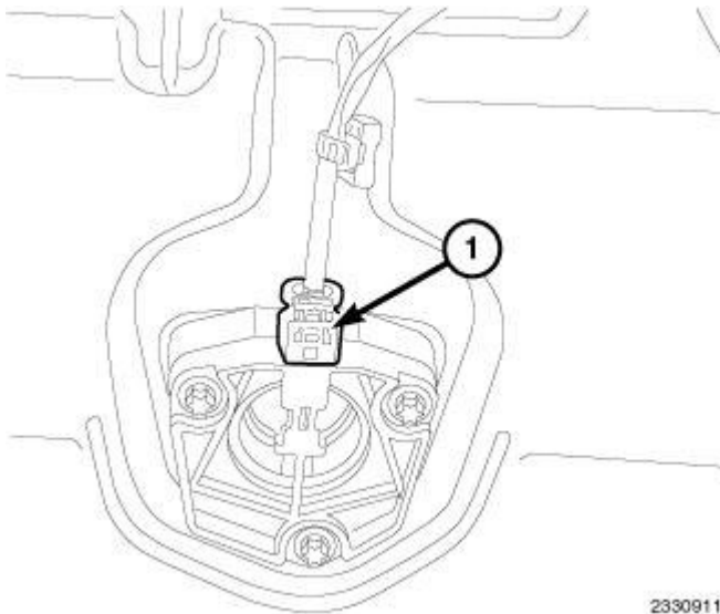
Fig. 60: Oil Life Monitor Harness Connector Courtesy of CHRYSLER LLC
