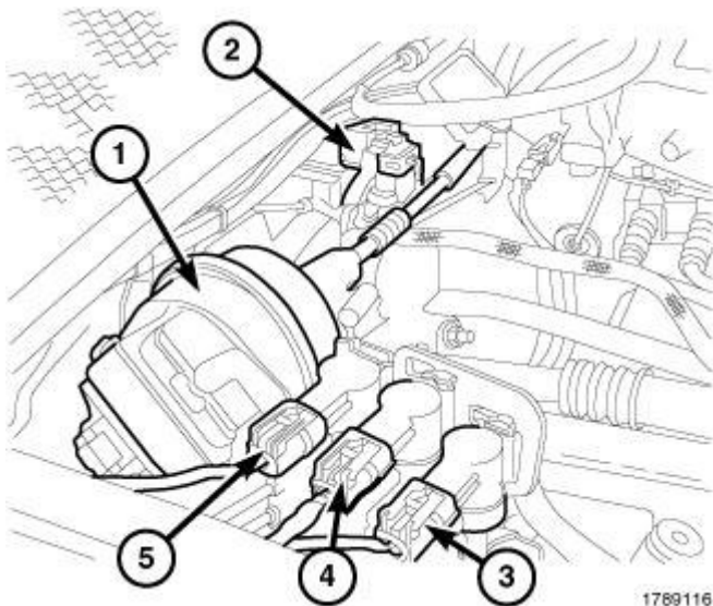
Fig. 557: Wastegate Solenoid & Electrical Connectors Courtesy of CHRYSLER LLC
