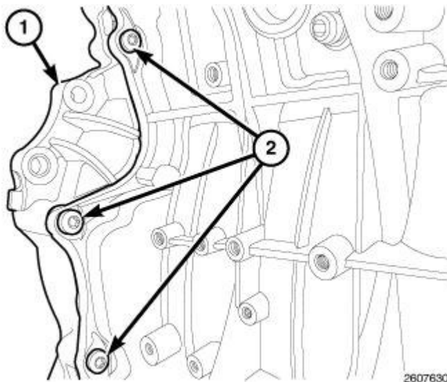
Fig. 606: Locating Bolts At Backside Of Timing Cover Courtesy of CHRYSLER LLC
