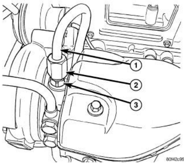
Fig. 550: Oil Supply Line & Fittings Courtesy of CHRYSLER LLC
