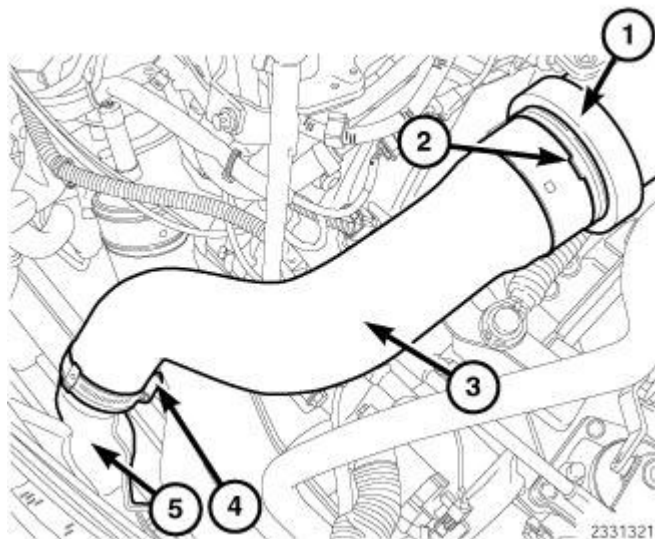
Fig. 82: Upper Charge Air Tube, Lock Ring, Lower Charge Air Tube, Clamp & Charge Air Cooler (CAC) Inlet Courtesy of CHRYSLER LLC
