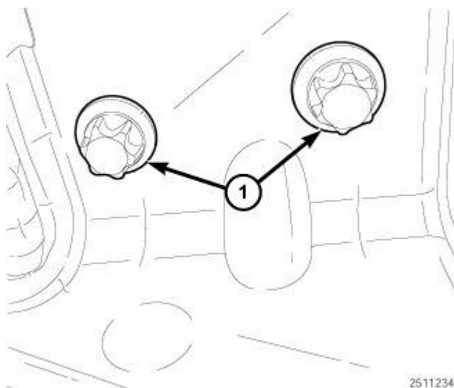
Fig. 648: CAC Tube And Bracket Assembly Bolts Courtesy of CHRYSLER LLC
