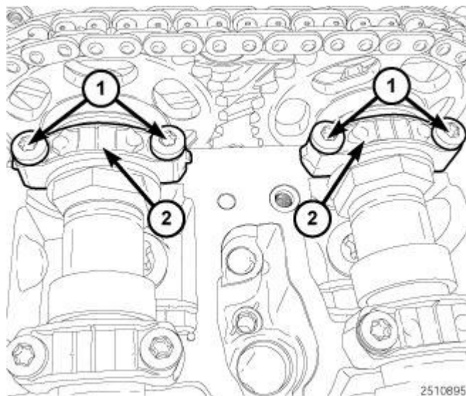
Fig. 654: No. 1 Camshaft Bearing Caps & Bolts Courtesy of CHRYSLER LLC
