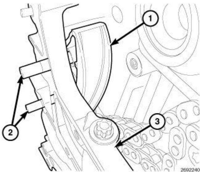
Fig. 641: Timing Chain Guide, Guide Pins & Cylinder Head Courtesy of CHRYSLER LLC
