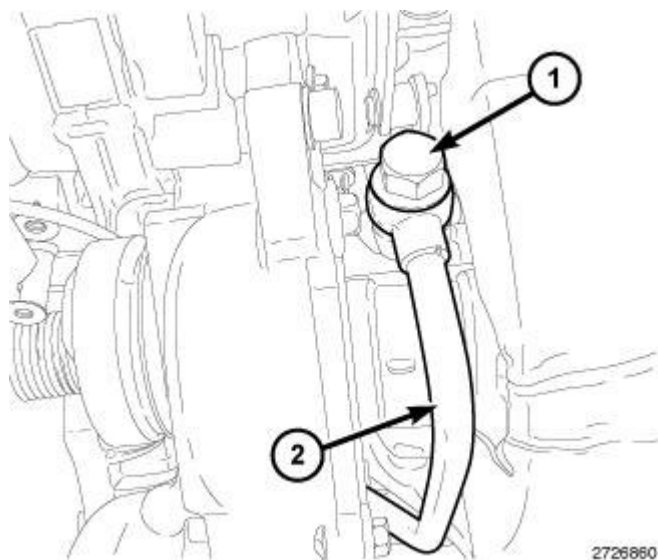
Fig. 570: Oil Supply Line & Banjo Bolt At Turbocharger Courtesy of CHRYSLER LLC
