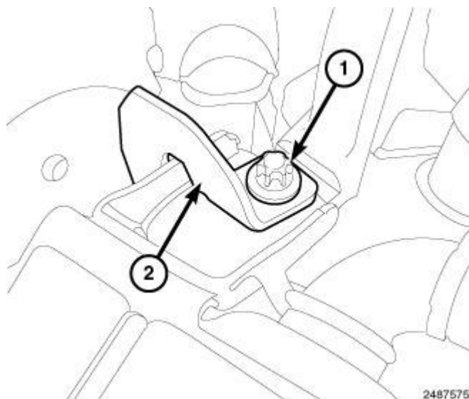
Fig. 616: Upper EGR Cooler Bolt & Bracket Courtesy of CHRYSLER LLC
