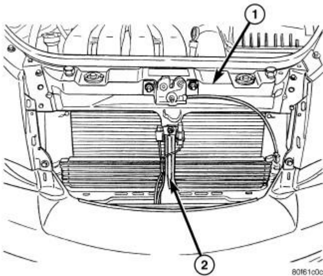
Fig. 538: Upper Radiator Closure Panel & Center Brace Courtesy of CHRYSLER LLC
