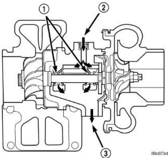
Fig. 565: Turbocharger Bearings, Oil Supply & Drain Courtesy of CHRYSLER LLC
