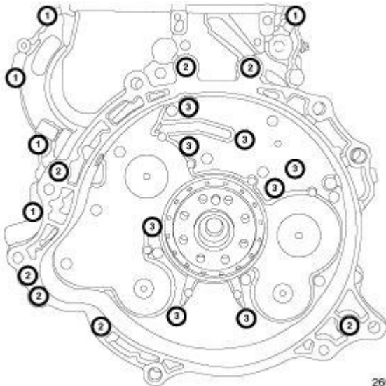
Fig. 630: Timing Chain Cover At Engine Bolts Courtesy of CHRYSLER LLC
