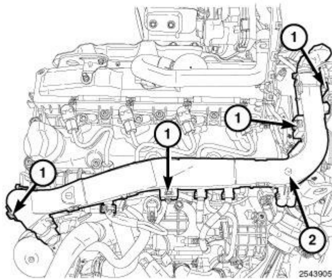
Fig. 176: Lock Tabs & Engine Wire Harness Courtesy of CHRYSLER LLC
