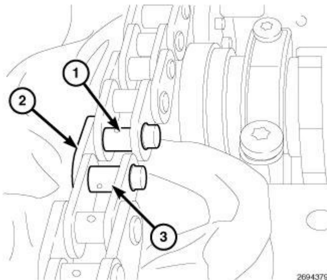
Fig. 583: Connecting New Timing Chain With Old Timing Chain With Assembly Link Courtesy of CHRYSLER LLC
