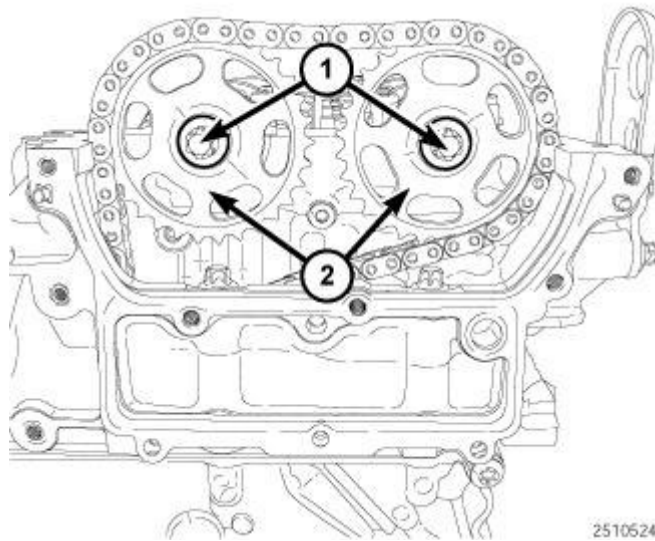
Fig. 638: Camshaft Sprockets & Bolts Courtesy of CHRYSLER LLC
