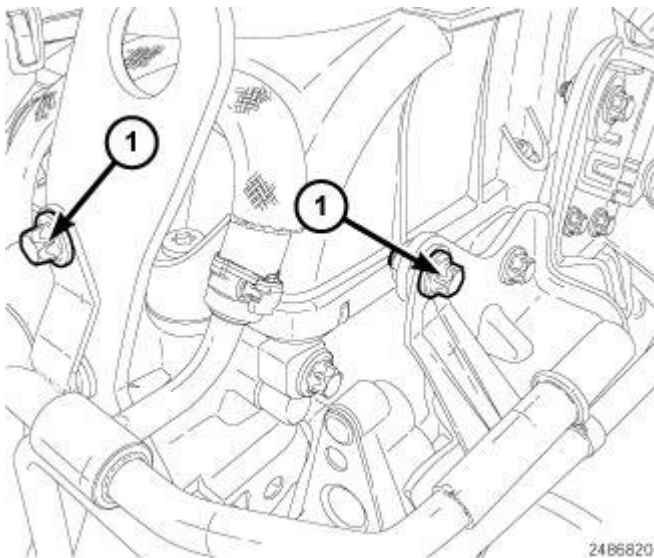
Fig. 590: Upper Fuel Line Bracket Bolts Courtesy of CHRYSLER LLC
