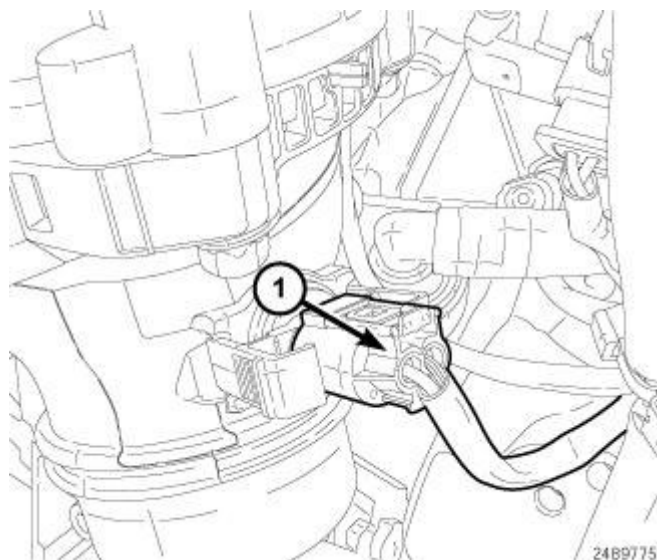
Fig. 512: Charge Air Inlet Temperature Sensor Harness Connector Courtesy of CHRYSLER LLC
