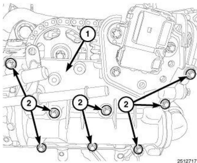
Fig. 611: Timing Chain Upper Cover & Bolts Courtesy of CHRYSLER LLC
