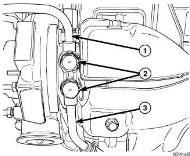
Fig. 545: Coolant Lines & Banjo Fittings Courtesy of CHRYSLER LLC
