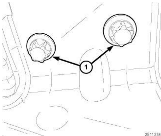
Fig. 665: CAC Tube And Bracket Assembly Bolts Courtesy of CHRYSLER LLC
