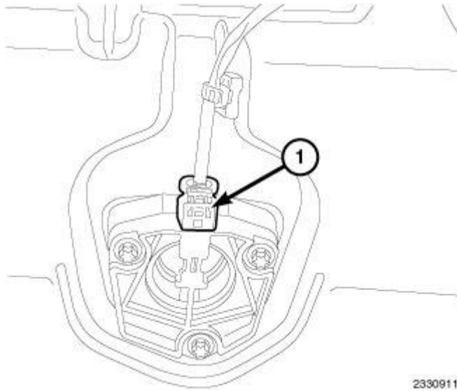
Fig. 48: Oil Life Monitor Harness Connector Courtesy of CHRYSLER LLC
