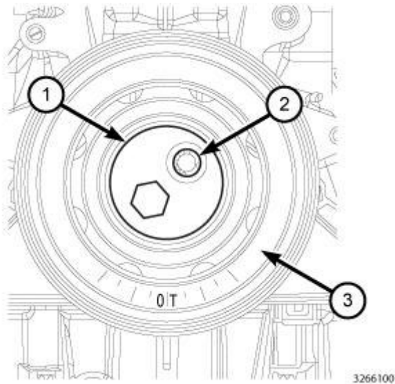
Fig. 651: Vibration Damper Holder Tool, Vibration Damper & Bolts Courtesy of CHRYSLER LLC
