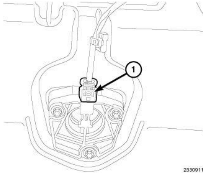
Fig. 326: Oil Life Monitor Harness Connector Courtesy of CHRYSLER LLC
