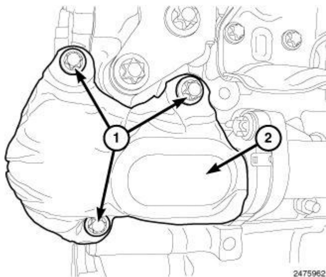
Fig. 594: EGR Pipe Heat Shield & Bolts Courtesy of CHRYSLER LLC
