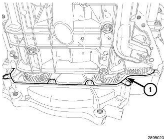
Fig. 323: Applying A 2-mm Bead Of Loctite® Onto Timing Cover Mating Surface Courtesy of CHRYSLER LLC
