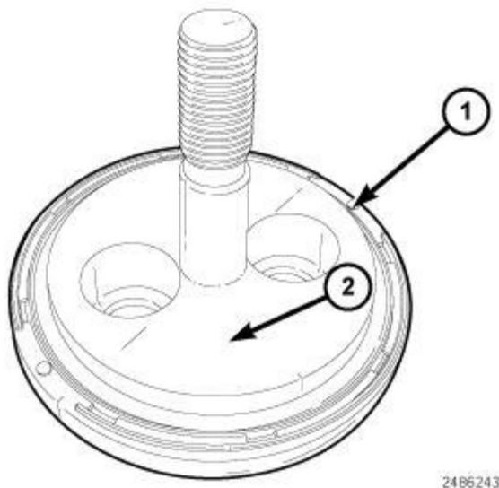
Fig. 243: Front Crankshaft Oil Seal & Front Crankshaft Seal Adapter Courtesy of CHRYSLER LLC
