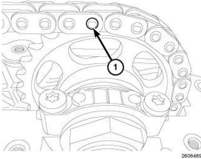
Fig. 581: Timing Chain Pin At Chain Link Courtesy of CHRYSLER LLC
