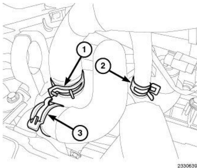
Fig. 31: Heater Hoses At Engine Courtesy of CHRYSLER LLC
