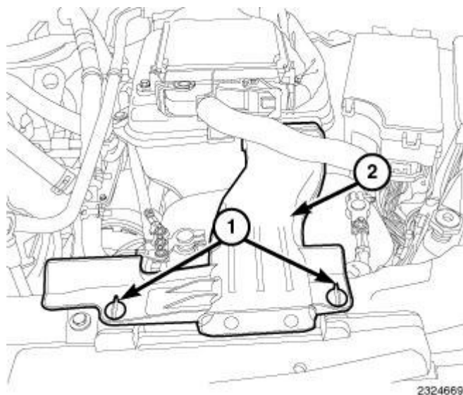
Fig. 91: Quarter Turn Lock Tabs & Air Inlet Duct Courtesy of CHRYSLER LLC
