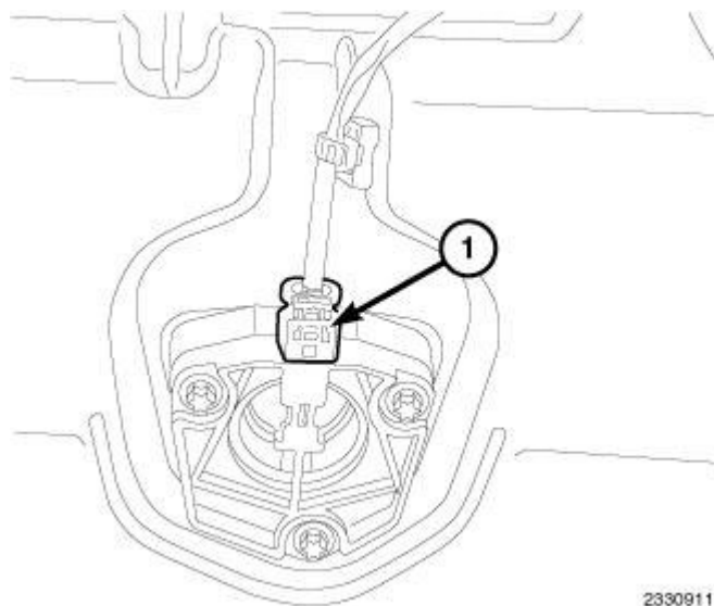
Fig. 223: Oil Life Monitor Harness Connector Courtesy of CHRYSLER LLC
