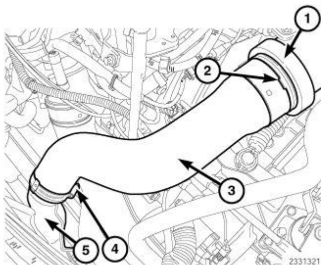
Fig. 566: Upper Charge Air Tube, Lock Ring, Lower Charge Air Tube, Clamp & Charge Air Cooler (CAC) Inlet
