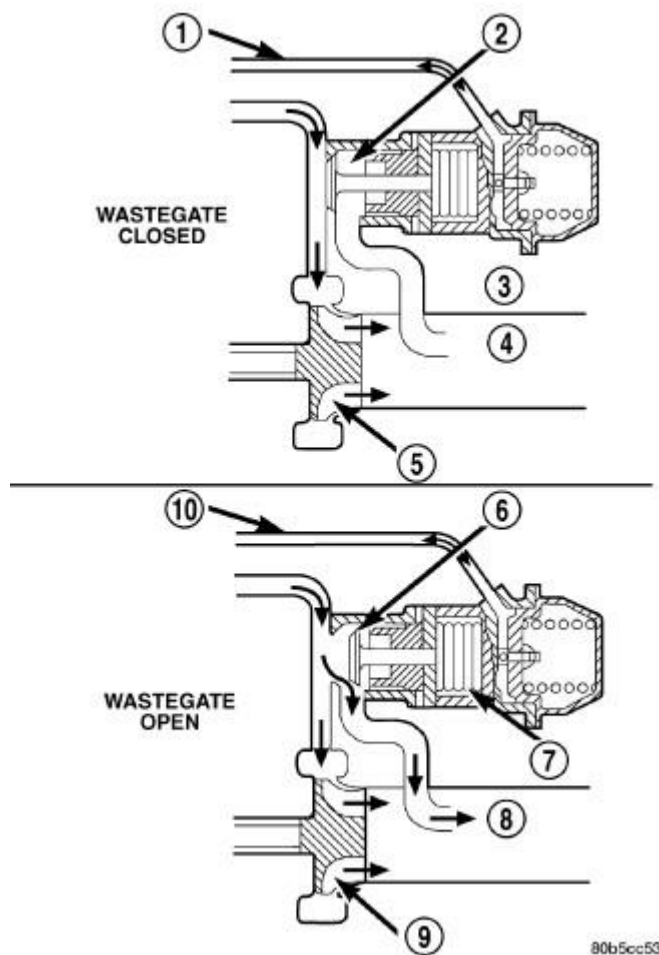
Fig. 564: Wastegate Operation Courtesy of CHRYSLER LLC
