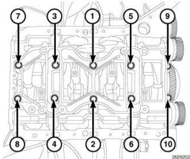
Fig. 219: Crankshaft Main Bearing Cap Bolts Torque Sequence Courtesy of CHRYSLER LLC
