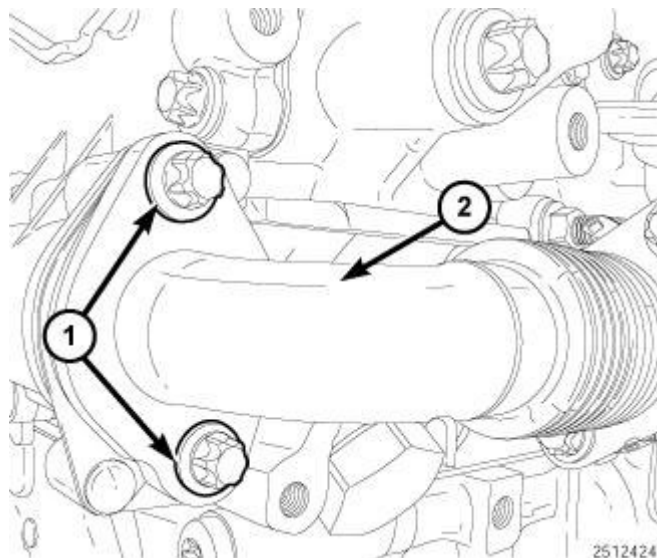
Fig. 623: EGR Pipe & Bolt Courtesy of CHRYSLER LLC
