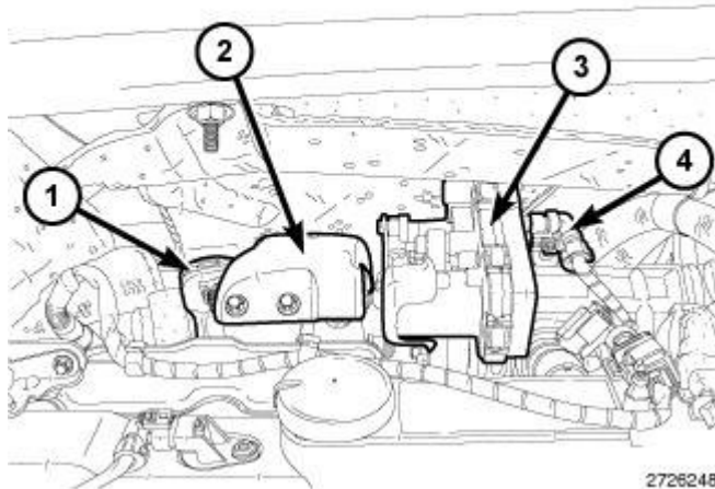
Fig. 567: Catalytic Converter, Turbocharger Heat Shield, Catalytic Converter Band Clamp & Upstream Temperature Sensor Courtesy of CHRYSLER LLC
