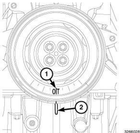
Fig. 652: Crankshaft Alignment Timing Marks Courtesy of CHRYSLER LLC
