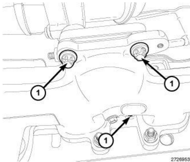
Fig. 572: Turbocharger-To-Exhaust Manifold Mounting Bolts Courtesy of CHRYSLER LLC
