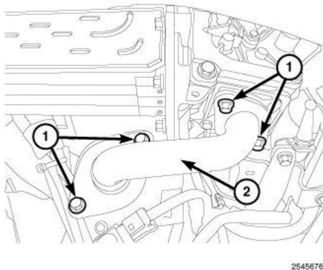
Fig. 596: EGR Tube & Bolts Courtesy of CHRYSLER LLC
