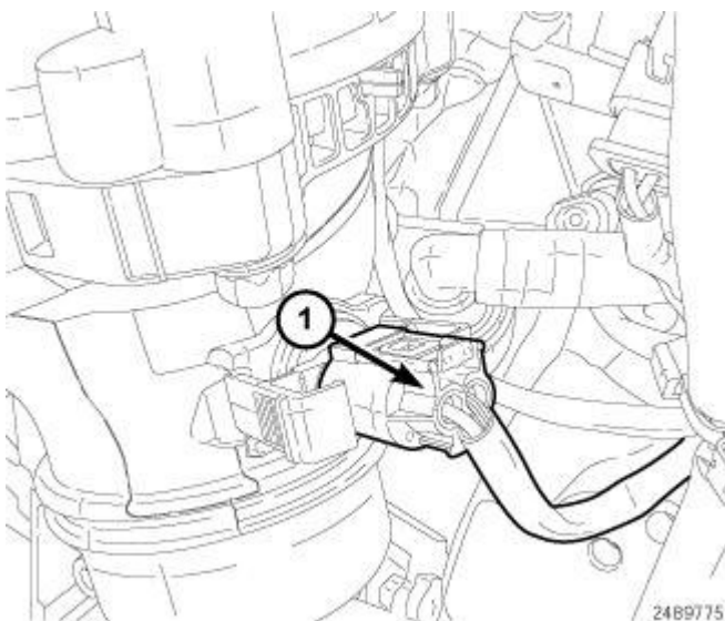
Fig. 451: Charge Air Inlet Temperature Sensor Harness Connector Courtesy of CHRYSLER LLC
