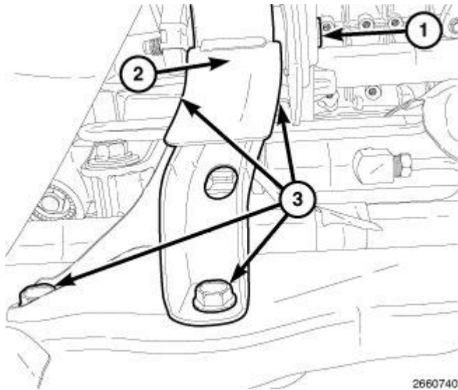
Fig. 67: Rear Roll Mount & Bolts Courtesy of CHRYSLER LLC
