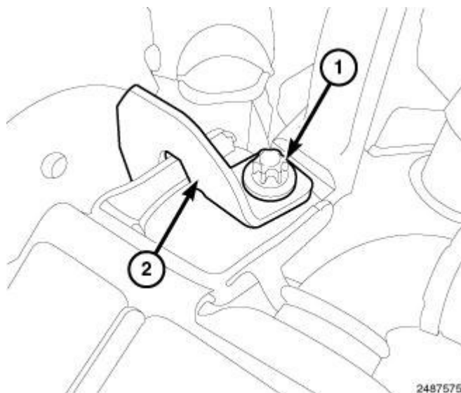
Fig. 600: Upper EGR Cooler Bolt & Bracket Courtesy of CHRYSLER LLC
