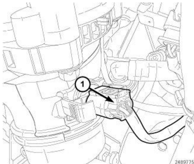
Fig. 352: Charge Air Inlet Temperature Sensor Harness Connector Courtesy of CHRYSLER LLC
