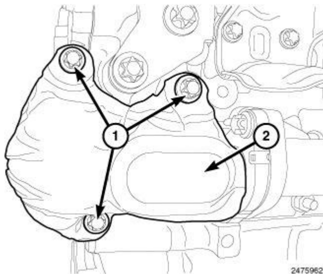
Fig. 624: EGR Pipe Heat Shield & Bolts Courtesy of CHRYSLER LLC
