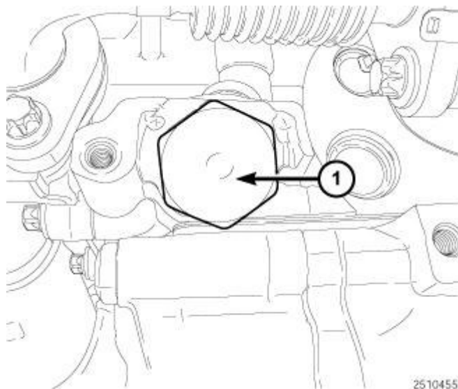
Fig. 659: Timing Chain Tensioner Courtesy of CHRYSLER LLC
