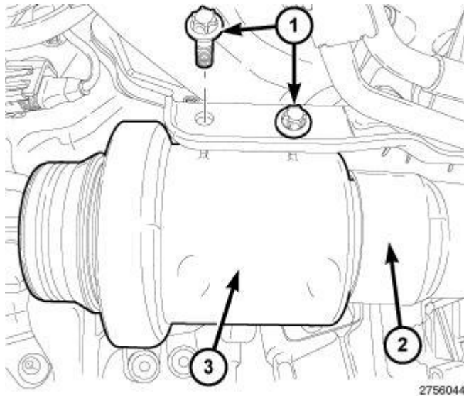
Fig. 536: Air Charge Resonator, Rear Air Charge Tube & Mounting Bolts Courtesy of CHRYSLER LLC
