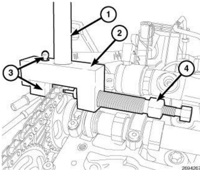
Fig. 582: Chain Link Tool, Handle, Insert & Thrust Screw/Pin Courtesy of CHRYSLER LLC
