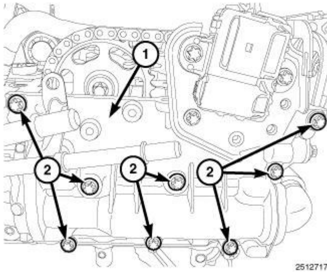
Fig. 605: Timing Chain Upper Cover & Bolts Courtesy of CHRYSLER LLC
