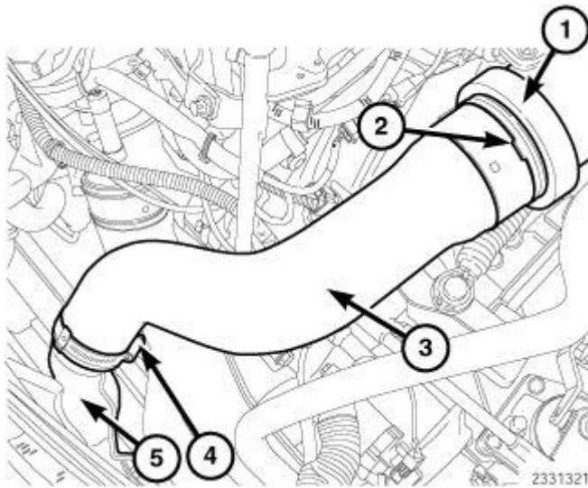
Fig. 580: Upper Charge Air Tube, Lock Ring, Lower Charge Air Tube, Clamp & Charge Air Cooler (CAC) Inlet
