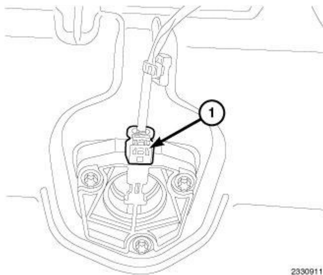
Fig. 364: Oil Life Monitor Harness Connector Courtesy of CHRYSLER LLC
