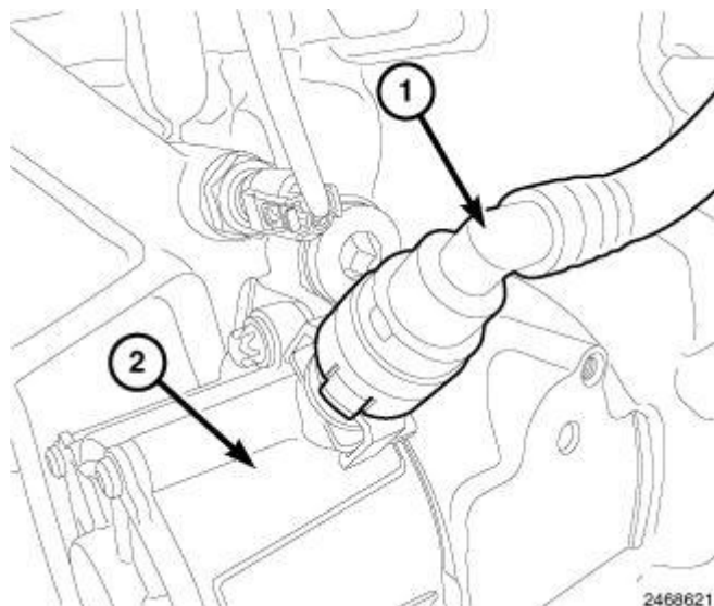
Fig. 348: Vacuum Hose At Vacuum Pump
