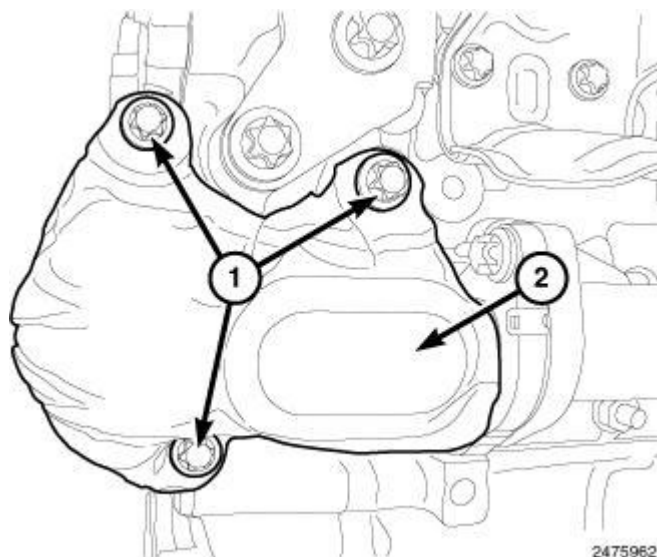
Fig. 660: EGR Pipe Heat Shield & Bolts Courtesy of CHRYSLER LLC
