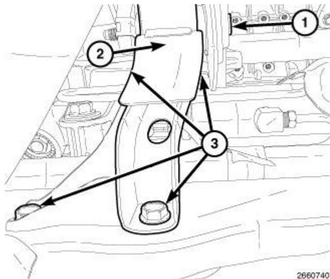
Fig. 40: Rear Roll Mount & Bolts Courtesy of CHRYSLER LLC
