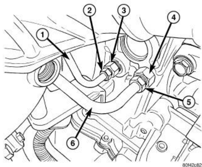
Fig. 549: Oil Supply Line, Oil Cooler Coolant Line & Fittings Courtesy of CHRYSLER LLC
