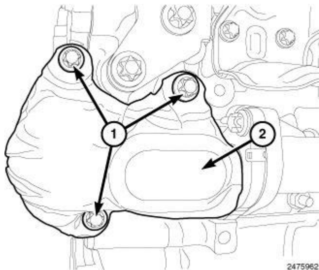
Fig. 656: EGR Pipe Heat Shield & Bolts Courtesy of CHRYSLER LLC
