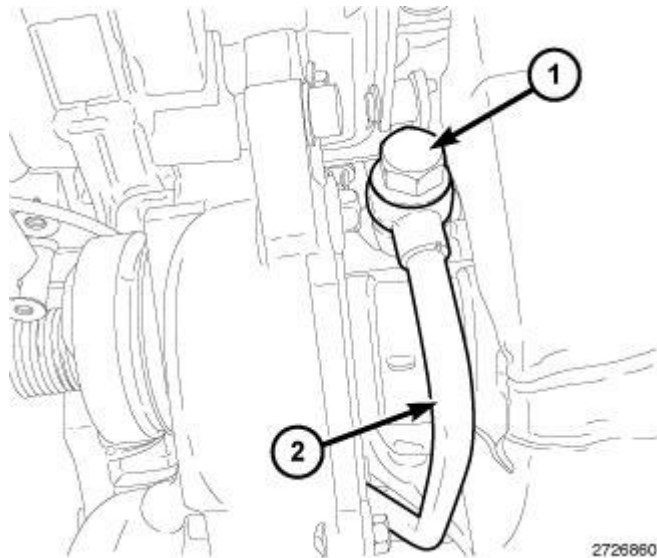
Fig. 576: Oil Supply Line & Banjo Bolt At Turbocharger Courtesy of CHRYSLER LLC
