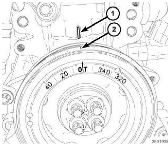
Fig. 633: Positioning Cylinder No. 1 Piston To Ignition TDC Courtesy of CHRYSLER LLC
