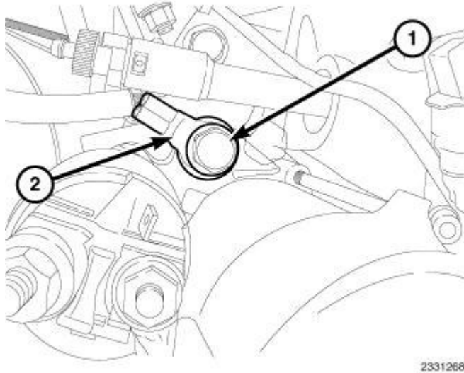
Fig. 73: Battery Ground Cable & Bolt At Engine Block Courtesy of CHRYSLER LLC
