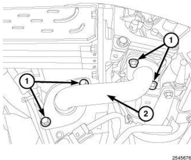
Fig. 622: EGR Tube & Bolts Courtesy of CHRYSLER LLC
