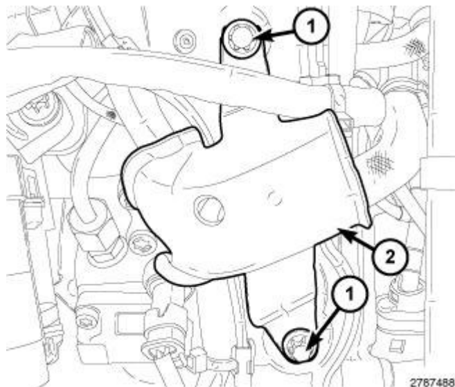
Fig. 599: Bolts & Heat Shield Courtesy of CHRYSLER LLC
