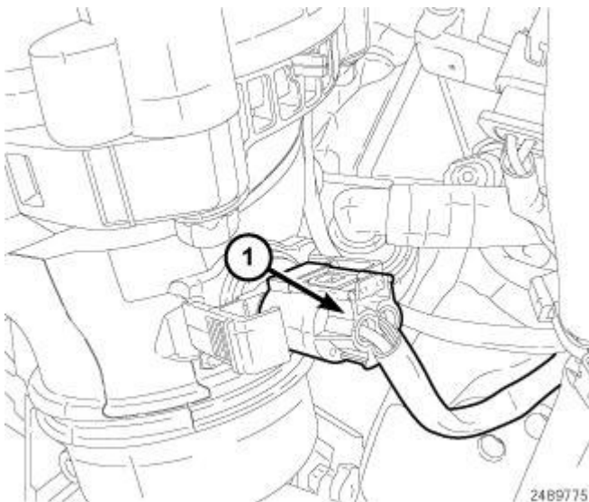
Fig. 429: Charge Air Inlet Temperature Sensor Harness Connector Courtesy of CHRYSLER LLC
