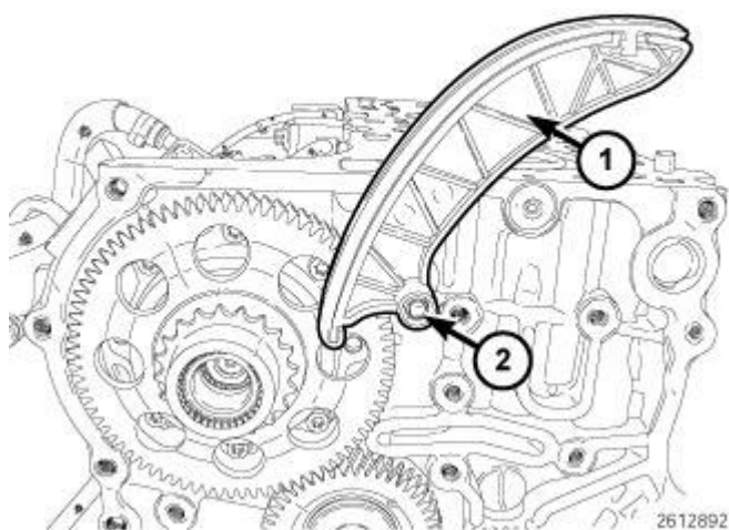
Fig. 647: Tensioning Rail & Pin Courtesy of CHRYSLER LLC
