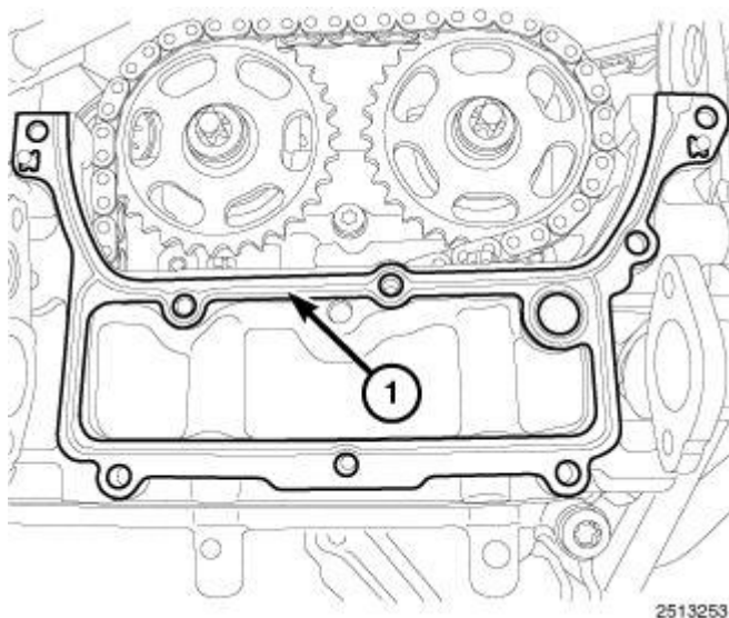
Fig. 608: Upper Timing Cover Gasket Courtesy of CHRYSLER LLC
