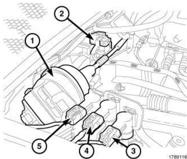
Fig. 562: Wastegate Solenoid & Electrical Connectors Courtesy of CHRYSLER LLC
