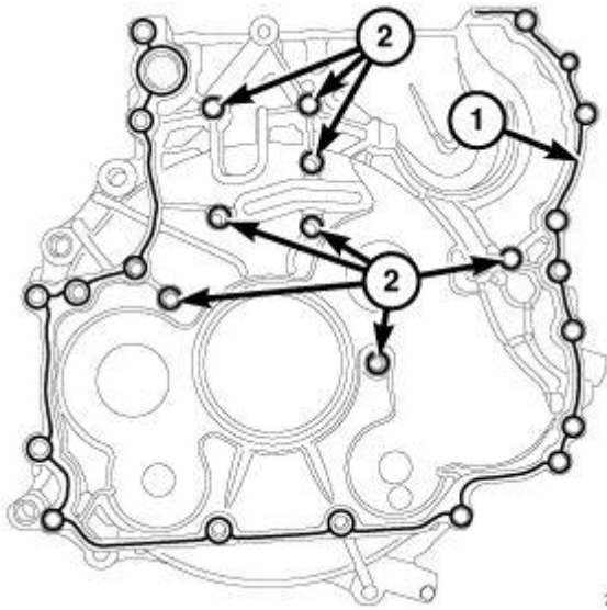
Fig. 629: Applying Sealant To Lower Timing Chain Cover Mating Surfaces Courtesy of CHRYSLER LLC
