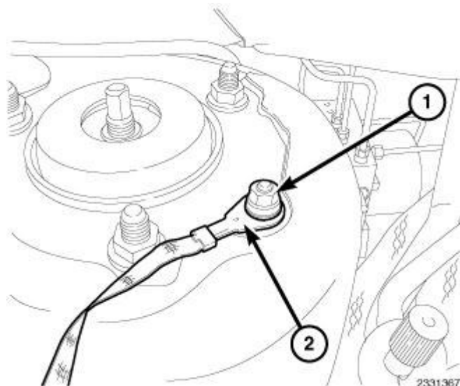
Fig. 28: Engine Ground Strap & Retaining Nut Courtesy of CHRYSLER LLC
