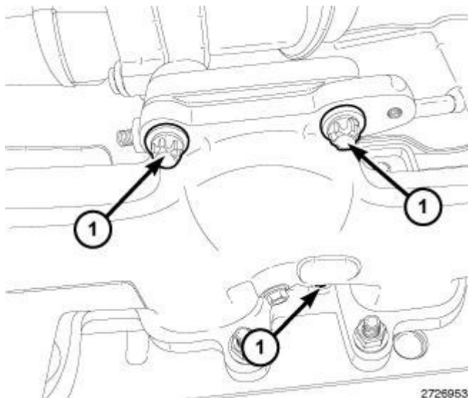
Fig. 574: Turbocharger-To-Exhaust Manifold Mounting Bolts Courtesy of CHRYSLER LLC
