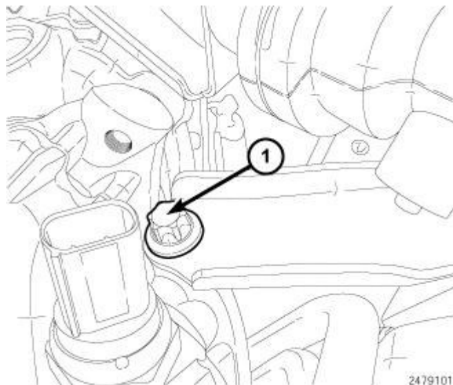
Fig. 603: Support Bracket Bolt Courtesy of CHRYSLER LLC
