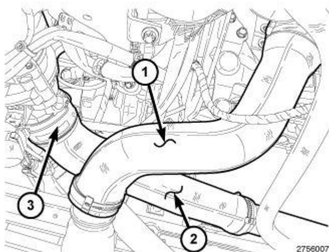
Fig. 535: Front Upper, Lower Air Charge Hose & Clamp Courtesy of CHRYSLER LLC
