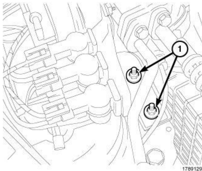
Fig. 558: Nuts Securing Solenoid Mounting Bracket Courtesy of CHRYSLER LLC
