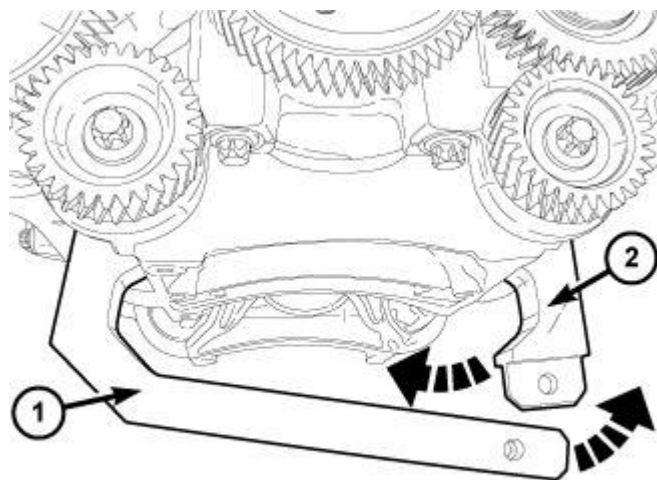
Fig. 328: Installing Balance Shaft Lock Tool Halves & Rotating Into Locked Position Courtesy of CHRYSLER LLC
