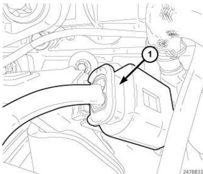
Fig. 445: Fuel Quality Control Valve Harness Connector Courtesy of CHRYSLER LLC
