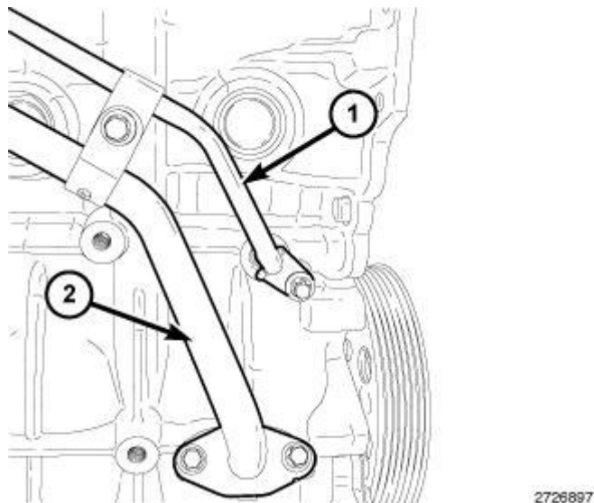
Fig. 571: Oil Supply & Return Lines Courtesy of CHRYSLER LLC
