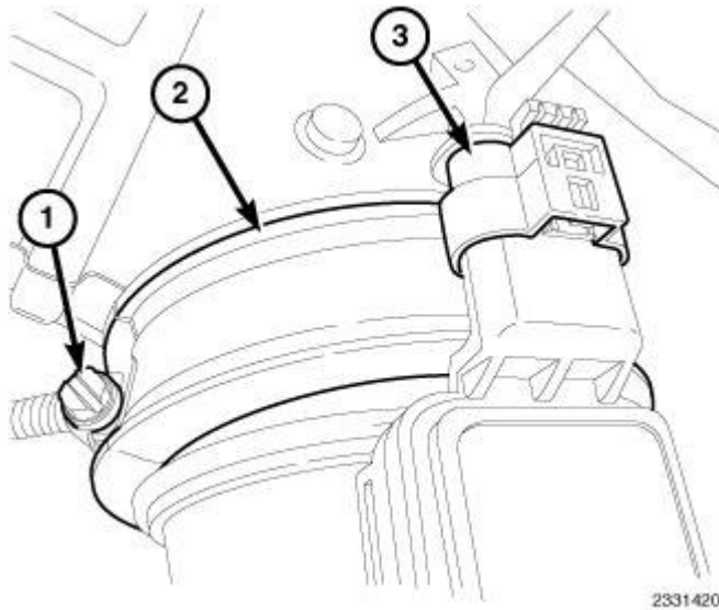
Fig. 90: Mass Air Flow Sensor Harness Connector, Air Cleaner-To-Turbocharger Inlet Tube & Clamp Courtesy of CHRYSLER LLC
