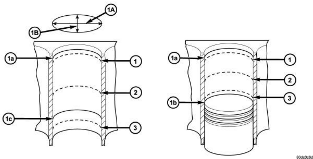
Fig. 198: Measuring Cylinder Bores Courtesy of CHRYSLER LLC
