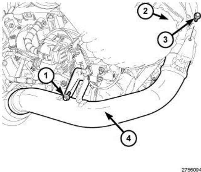
Fig. 537: Rear Air Charge Tube & Bolts Courtesy of CHRYSLER LLC
