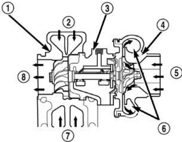
Fig. 563: Turbocharger Description
