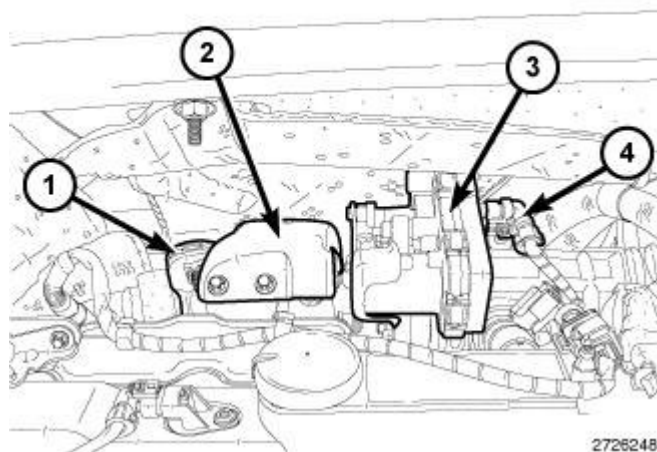
Fig. 579: Catalytic Converter, Turbocharger Heat Shield, Catalytic Converter Band Clamp & Upstream Temperature Sensor Courtesy of CHRYSLER LLC
