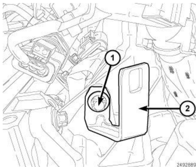
Fig. 298: Wire Harness Support Bracket & Bolts Courtesy of CHRYSLER LLC
