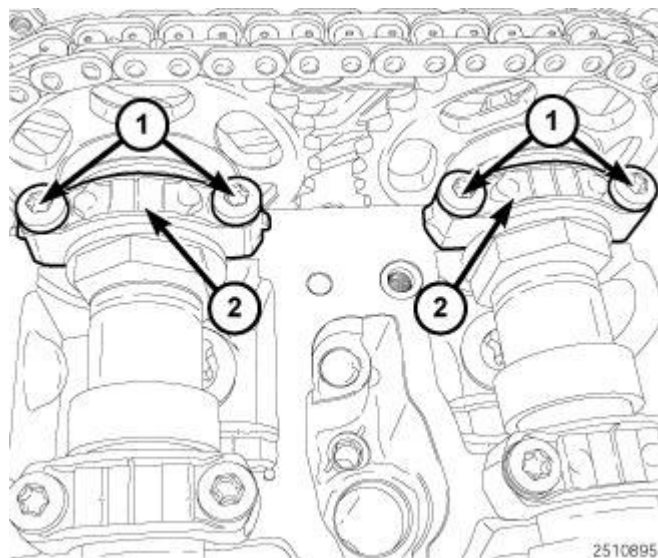
Fig. 662: No. 1 Camshaft Bearing Caps & Bolts Courtesy of CHRYSLER LLC
