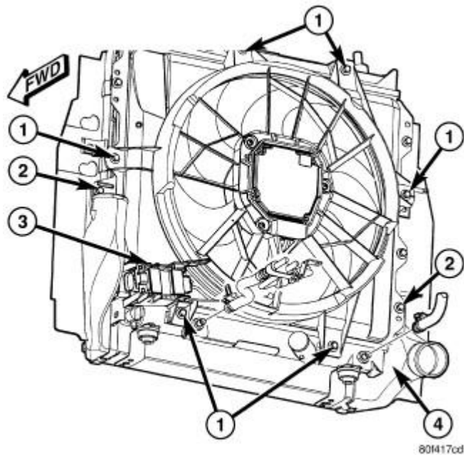
Fig. 539: Cooling Module - 2.4L Turbo Courtesy of CHRYSLER LLC
