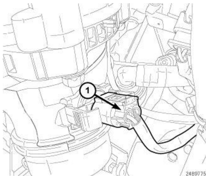
Fig. 347: Charge Air Inlet Temperature Sensor Harness Connector Courtesy of CHRYSLER LLC
