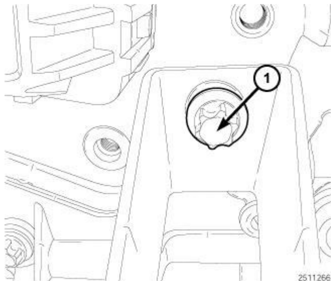
Fig. 663: Bolt Securing CAC Tube To Glow Plug Module Courtesy of CHRYSLER LLC
