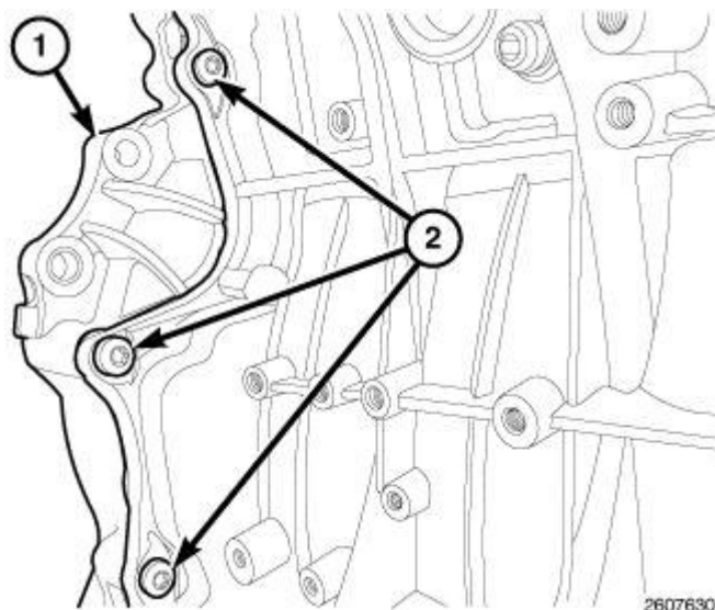
Fig. 631: Locating Bolts At Backside Of Timing Cover Courtesy of CHRYSLER LLC
