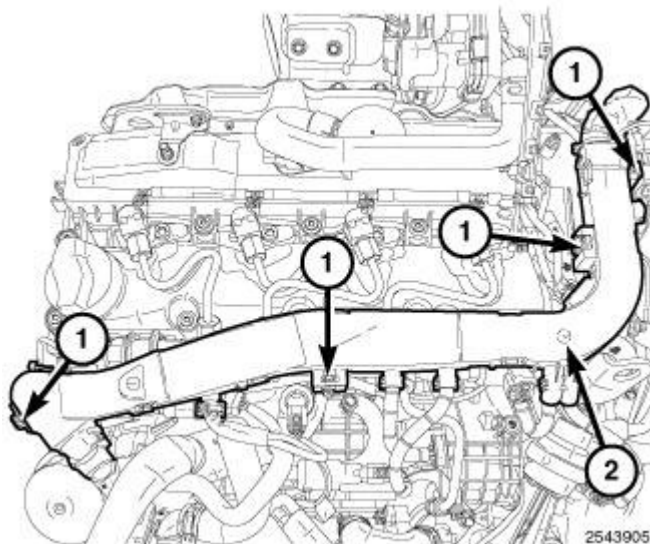
Fig. 161: Lock Tabs & Engine Wire Harness
