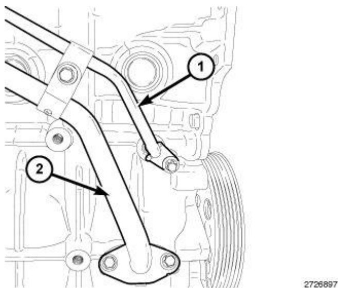
Fig. 575: Oil Supply & Return Lines Courtesy of CHRYSLER LLC
