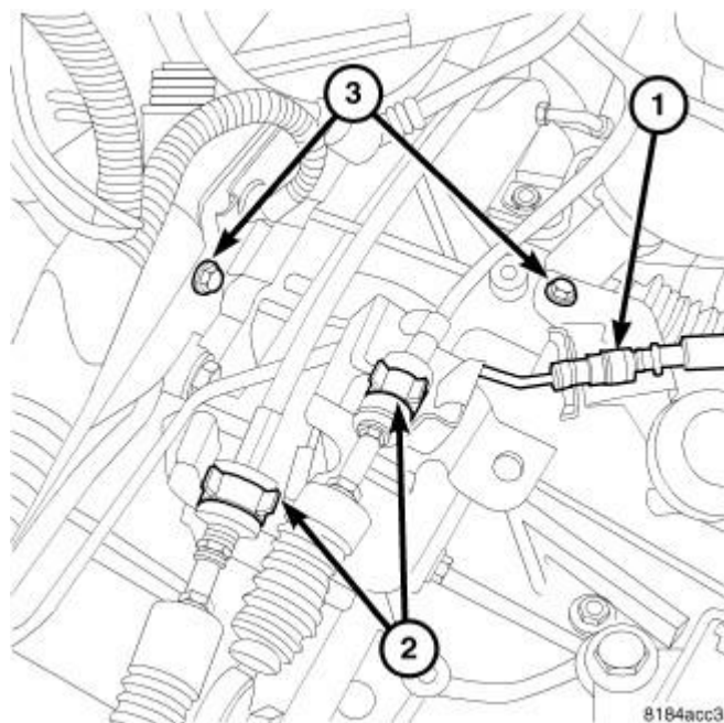
Fig. 72: Hydraulic Line, Shift Cables & Bolts Courtesy of CHRYSLER LLC
