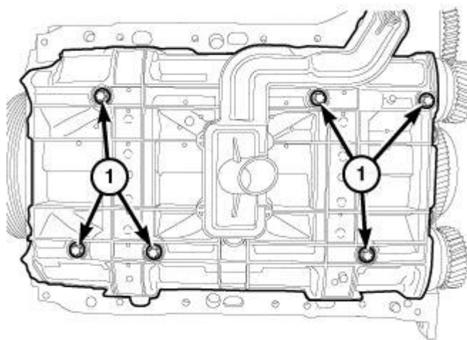
Fig. 327: Oil Pump Pickup Bolts Courtesy of CHRYSLER LLC
