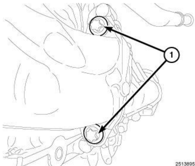
Fig. 612: EGR Assembly Bolts Courtesy of CHRYSLER LLC
