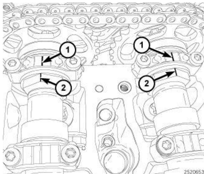
Fig. 634: Ensuring Camshaft Mark Is Aligned With Bearing Cap Mark Courtesy of CHRYSLER LLC
