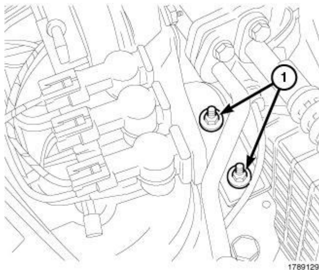
Fig. 561: Nuts Securing Solenoid Mounting Bracket Courtesy of CHRYSLER LLC
