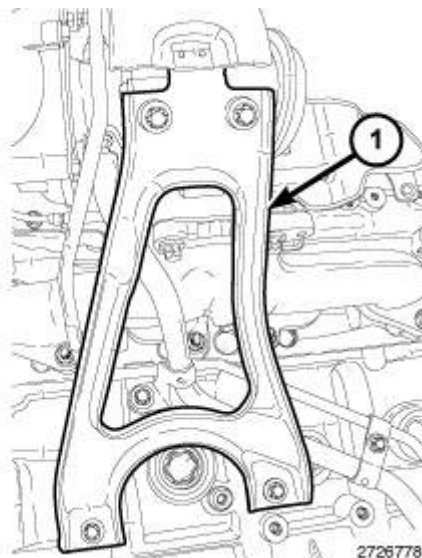
Fig. 578: Turbocharger Bracket Courtesy of CHRYSLER LLC
