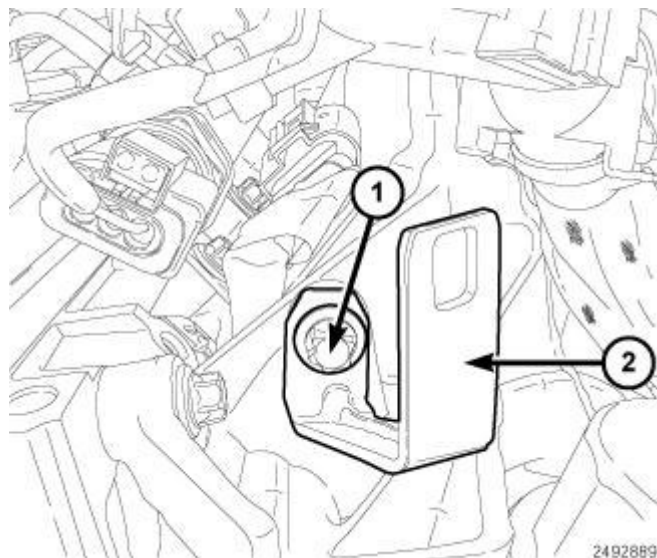
Fig. 464: Wire Harness Support Bracket & Bolts Courtesy of CHRYSLER LLC
