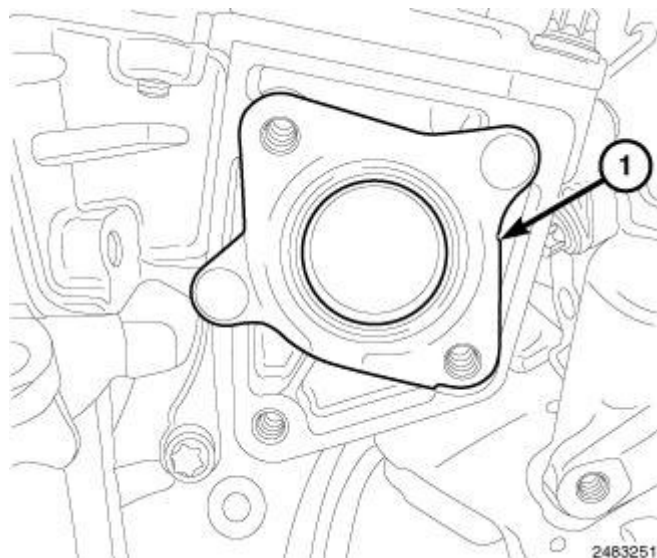
Fig. 621: EGR Tube Gasket Onto EGR Actuator Courtesy of CHRYSLER LLC
