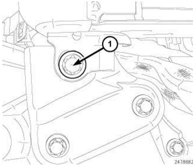
Fig. 601: Lower EGR Cooler Bolt Courtesy of CHRYSLER LLC
