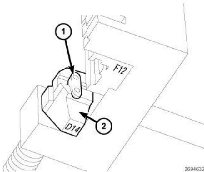
Fig. 585: Placing Outer Plate Into Thrust Piece With Digit D14
