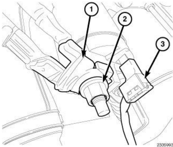
Fig. 74: Battery Feed Wire To Starter, Starter Harness Connections & Nut Courtesy of CHRYSLER LLC
