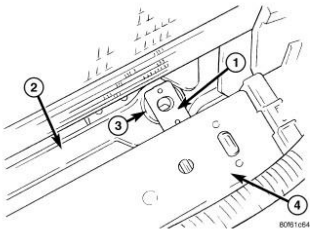
Fig. 543: Charge Air Cooler Locating Tab Courtesy of CHRYSLER LLC
