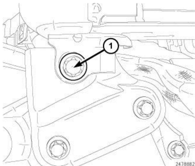
Fig. 615: Lower EGR Cooler Bolt Courtesy of CHRYSLER LLC
