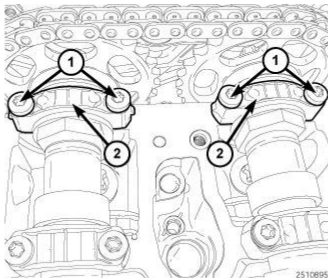
Fig. 646: No. 1 Camshaft Bearing Caps & Bolts Courtesy of CHRYSLER LLC
