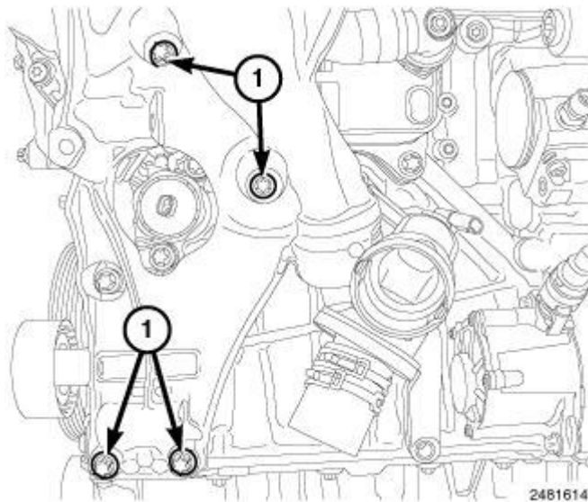
Fig. 309: Accessory Carrier Bolts
