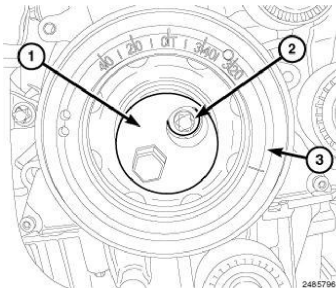
Fig. 632: Vibration Damper Holder, Bolts & Vibration Damper Courtesy of CHRYSLER LLC
