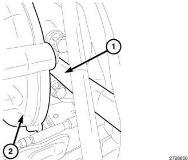
Fig. 569: Oil Return Line At Turbocharger Courtesy of CHRYSLER LLC
