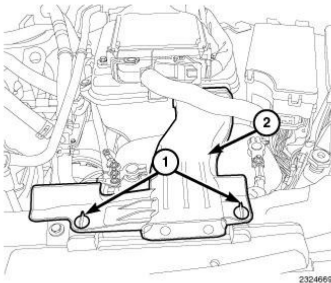
Fig. 181: Quarter Turn Lock Tabs & Air Inlet Duct Courtesy of CHRYSLER LLC
