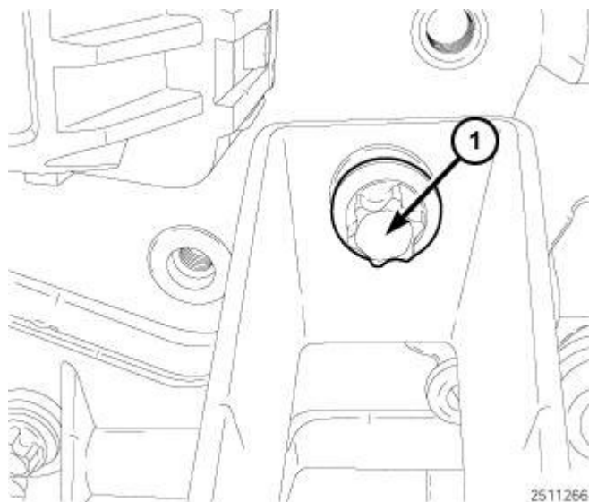
Fig. 650: Bolt Securing CAC Tube To Glow Plug Module Courtesy of CHRYSLER LLC
