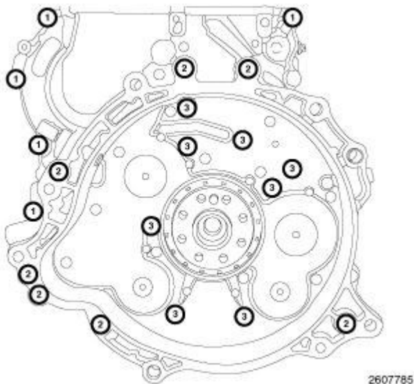
Fig. 607: Timing Chain Cover At Engine Bolts Courtesy of CHRYSLER LLC
