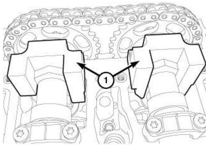
Fig. 661: Camshaft Lock Tools Courtesy of CHRYSLER LLC
