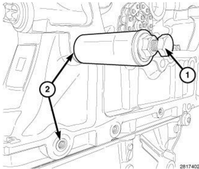
Fig. 639: Extractor Bolt Tool & Timing Guide Pin Courtesy of CHRYSLER LLC
