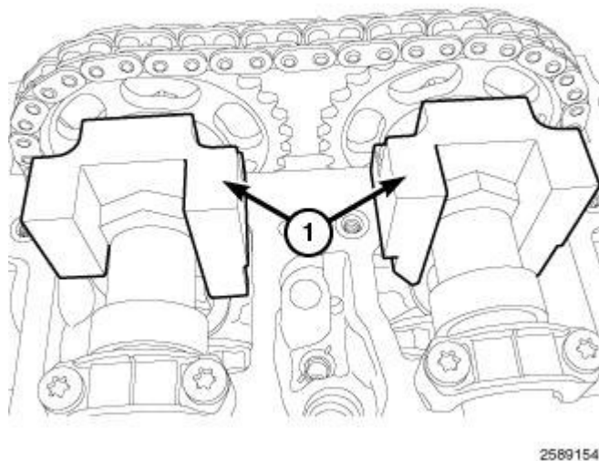
Fig. 645: Camshaft Lock Tools Courtesy of CHRYSLER LLC
