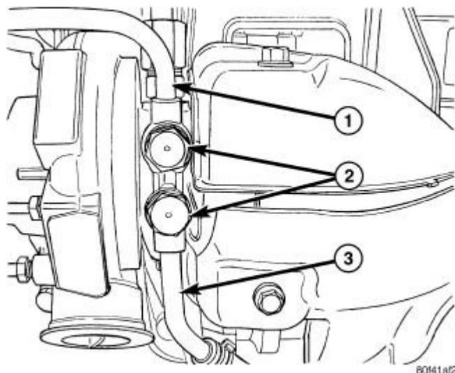
Fig. 552: Coolant Lines & Banjo Fittings Courtesy of CHRYSLER LLC
