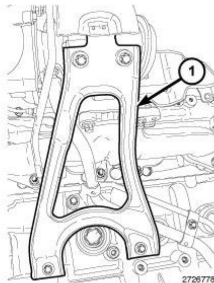
Fig. 568: Turbocharger Bracket Courtesy of CHRYSLER LLC
