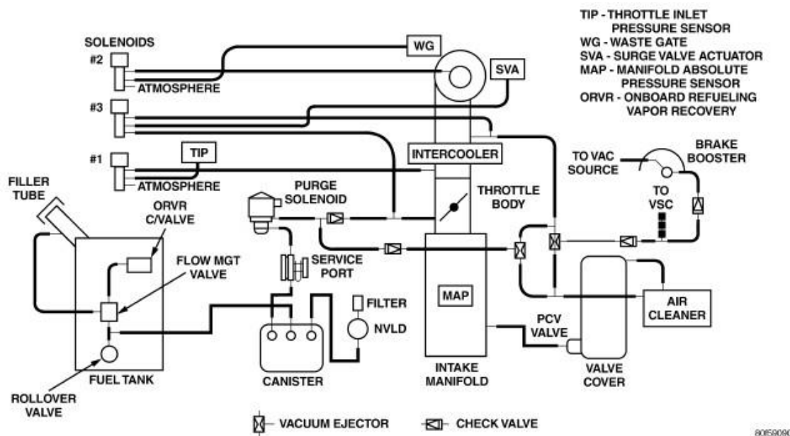
Fig. 556: Vacuum Harness Schematic Courtesy of CHRYSLER LLC
