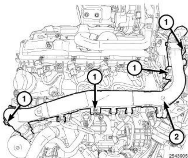
Fig. 463: Lock Tabs & Engine Wire Harness Courtesy of CHRYSLER LLC
