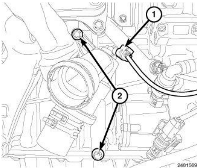
Fig. 310: ECT Sensor Connector & Thermostat Housing Bolts
