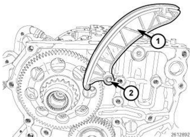
Fig. 640: Tensioning Rail & Pin Courtesy of CHRYSLER LLC
