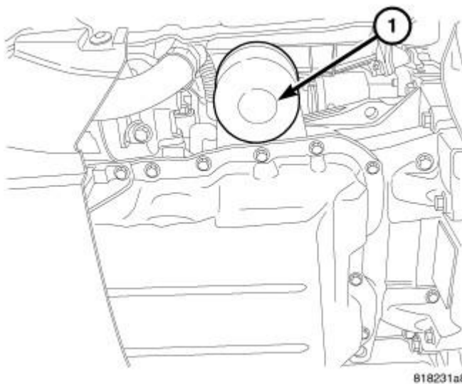
Fig. 189: Oil Filter
