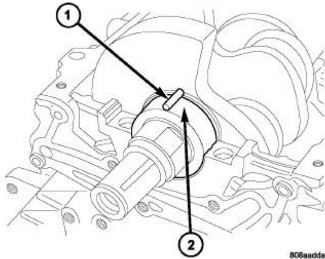
Fig. 8: Plastigage Placed In Lower Shell Courtesy of CHRYSLER GROUP, LLC
