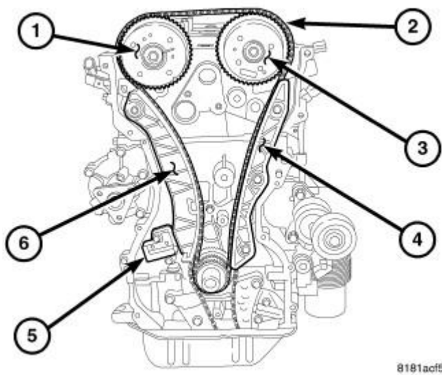
Fig. 388: Timing Drive System
