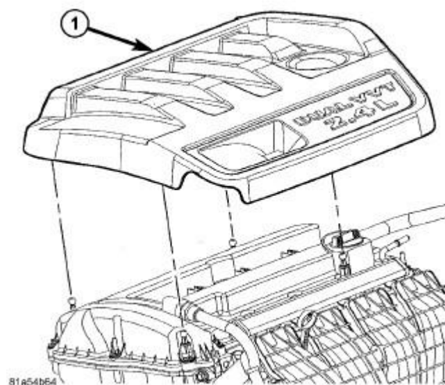
Fig. 336: Engine Cover - 2.4L
