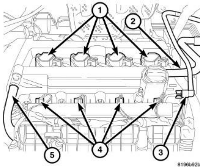
Fig. 11: Ignition Coils, Air Hose, Fuel Line, Injectors & PCV Hose
