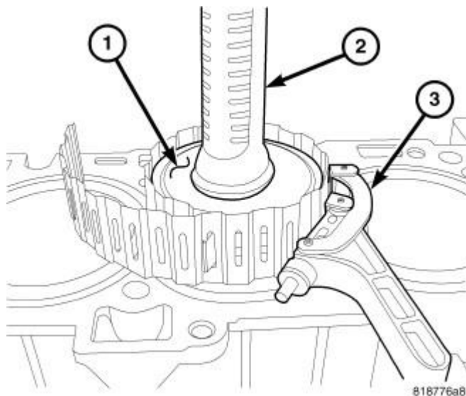
Fig. 212: Piston, Hammer Handle & Ring Compressor
