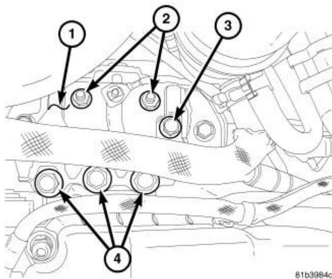
Fig. 57: Power Steering Hose Hold Down, Right Engine Mount Bracket & Fasteners Courtesy of CHRYSLER GROUP, LLC
