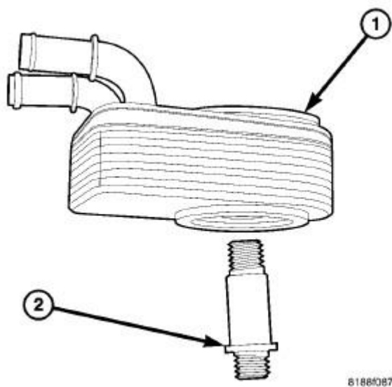
Fig. 274: Oil Cooler Mounting Courtesy of CHRYSLER GROUP, LLC
