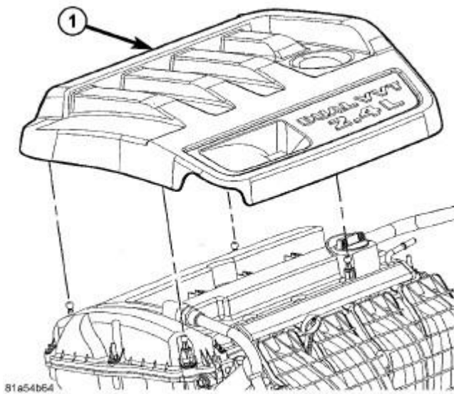
Fig. 10: Engine Cover - 2.4L
