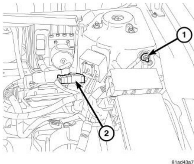
Fig. 323: Battery Cables
