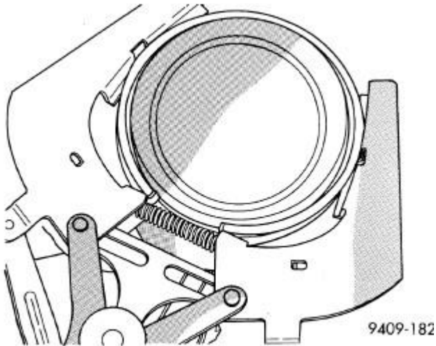
Fig. 200: Piston Rings-Removing And Installing Courtesy of CHRYSLER GROUP, LLC
