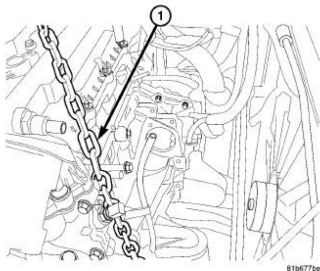
Fig. 214: Lift Chain
