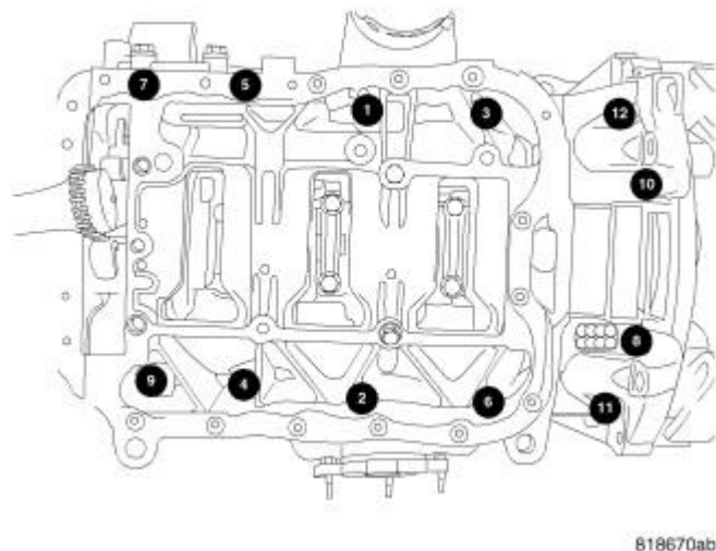
Fig. 197: Ladder Frame Bolts Tightening Sequence
