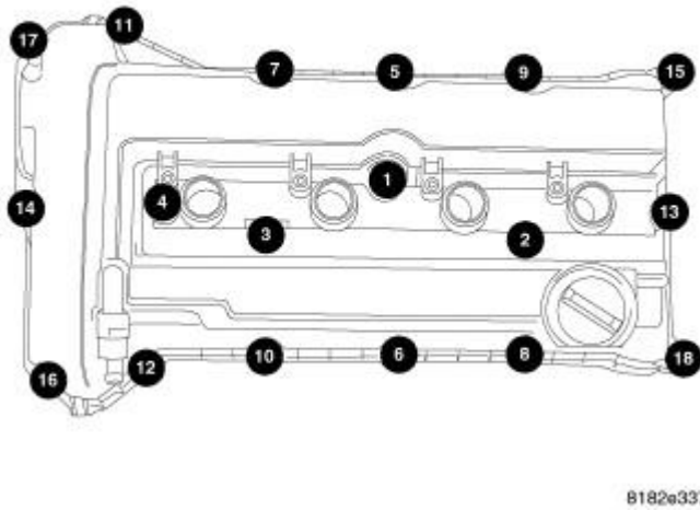
Fig. 359: Removing/Installing Cylinder Head Cover Bolts In Sequence Courtesy of CHRYSLER GROUP, LLC
