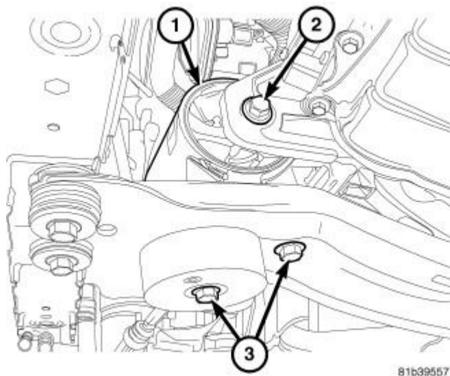
Fig. 226: Front Mount & Bolts
