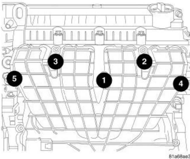
Fig. 19: Intake Bolt Removal/Tightening Sequence Courtesy of CHRYSLER GROUP, LLC
