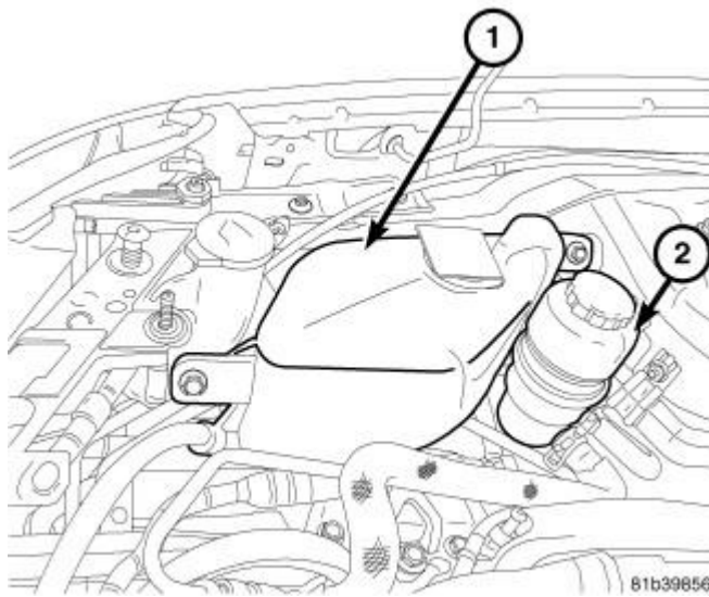
Fig. 248: Coolant Reservoir & Power Steering Reservoir Courtesy of CHRYSLER GROUP, LLC
