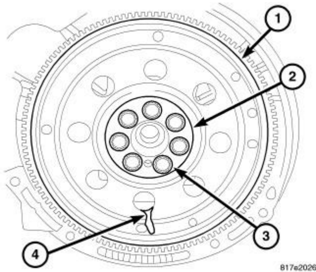
Fig. 224: Flex Plate
