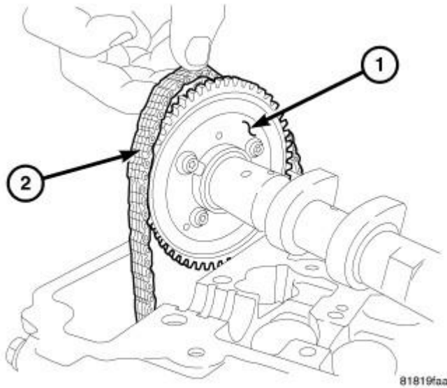
Fig. 129: Chain Removal
