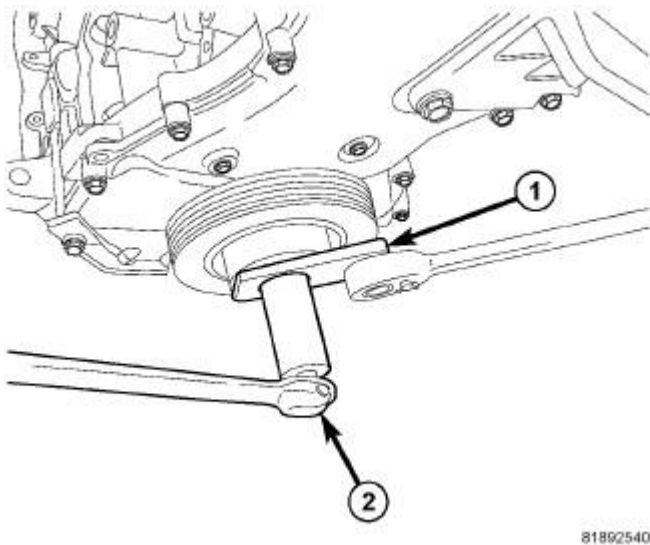
Fig. 190: Removing/Installing Crankshaft Damper Courtesy of CHRYSLER GROUP, LLC
