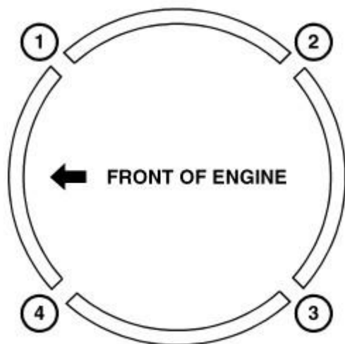
Fig. 202: Piston Ring End Gap Positions Courtesy of CHRYSLER GROUP, LLC
