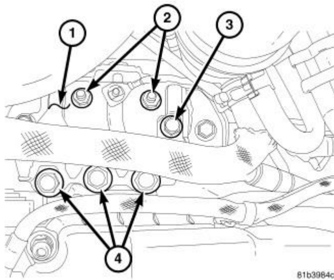
Fig. 377: Power Steering Hose Hold Down, Right Engine Mount Bracket & Fasteners Courtesy of CHRYSLER GROUP, LLC
