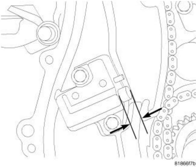
Fig. 344: Measuring Distance From Tensioner Body To Edge Of Chain Guide Courtesy of CHRYSLER GROUP, LLC
