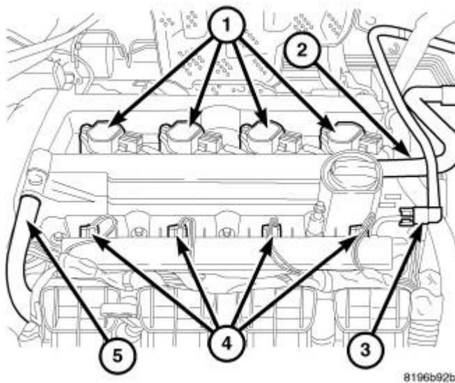
Fig. 328: Ignition Coils, Air Hose, Fuel Line, Injectors & PCV Hose Courtesy of CHRYSLER GROUP, LLC
