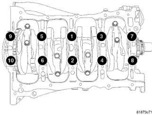
Fig. 177: Main Bearing Cap Removal/Installation Sequence Courtesy of CHRYSLER GROUP, LLC
