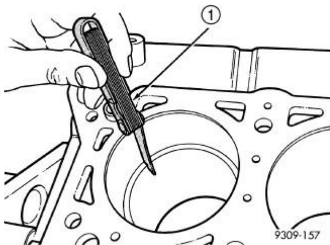
Fig. 198: Measuring Piston Ring Gap
