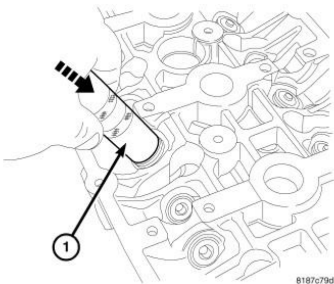
Fig. 154: Valve Removal
