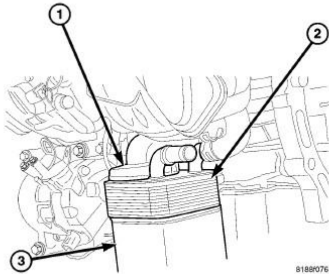
Fig. 275: Identifying Oil Cooler Courtesy of CHRYSLER GROUP, LLC
