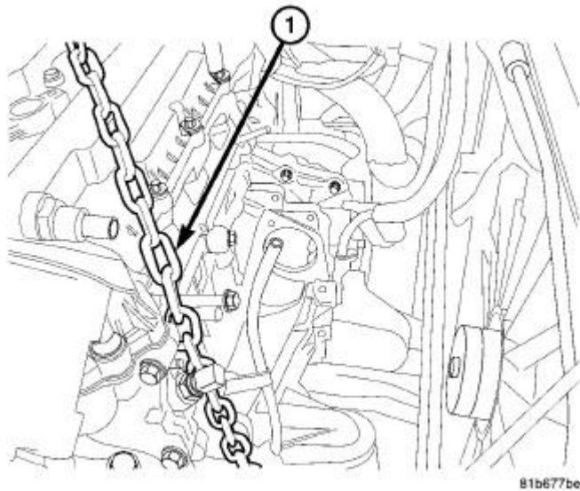
Fig. 27: Lift Chain Courtesy of CHRYSLER GROUP, LLC
