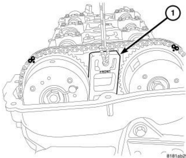
Fig. 138: Inserting Wedge 9701 Between Camshaft Phasers Courtesy of CHRYSLER GROUP, LLC
