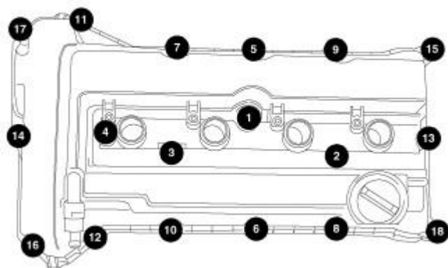
Fig. 98: Removing/Installing Cylinder Head Cover Bolts In Sequence
