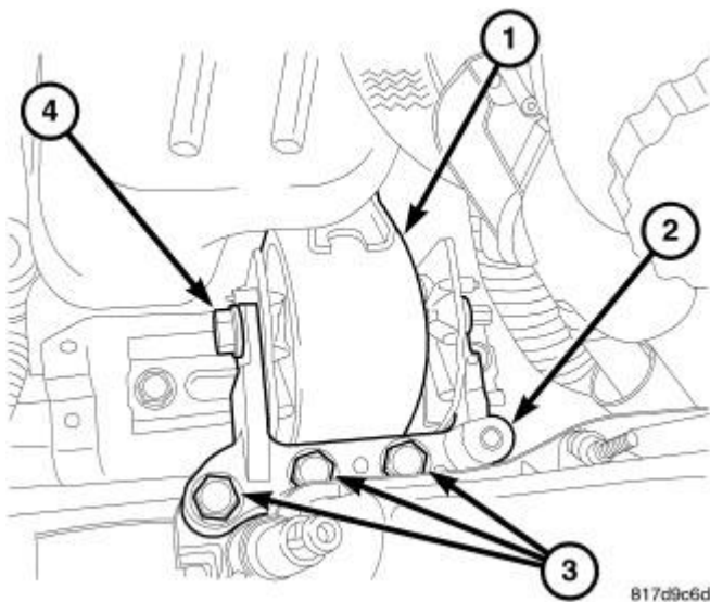
Fig. 30: Right Engine Mount & Fasteners
