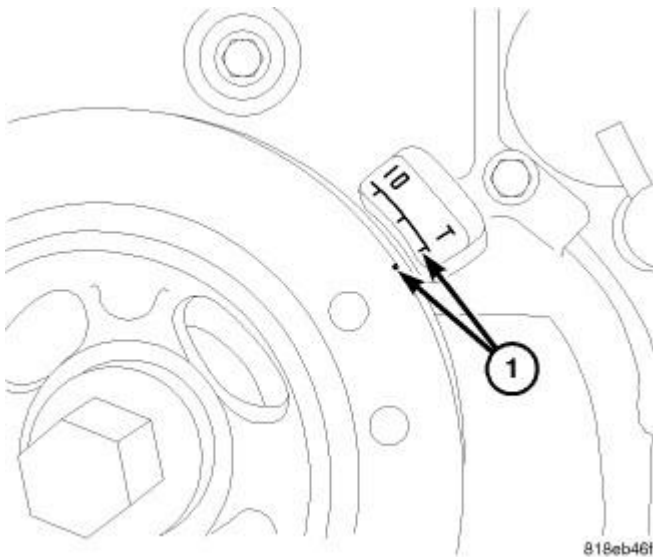
Fig. 120: TDC Courtesy of CHRYSLER GROUP, LLC
