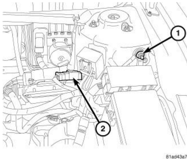
Fig. 335: Battery Cables
