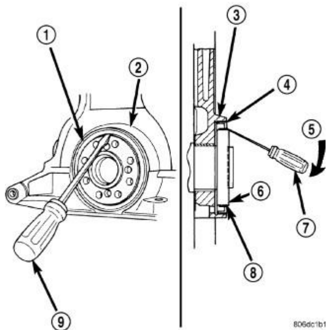
Fig. 222: Removing Rear Crankshaft Oil Seal
