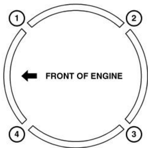
Fig. 210: Piston Ring End Gap Positions Courtesy of CHRYSLER GROUP, LLC
