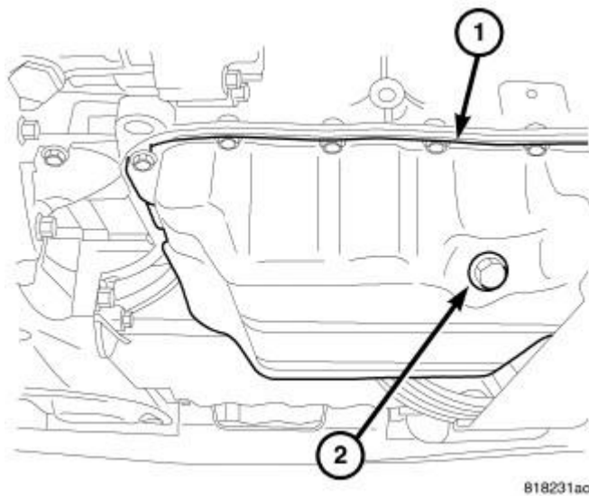
Fig. 207: Oil Drain Plug & Oil Pan
