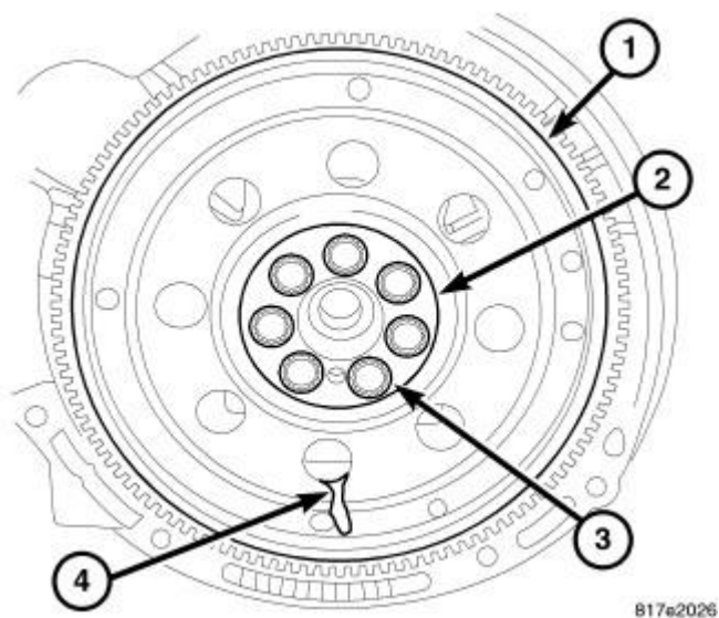
Fig. 221: Flex Plate
