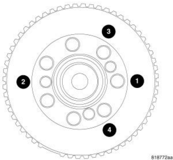
Fig. 180: Target Wheel Tightening Sequence Courtesy of CHRYSLER GROUP, LLC
