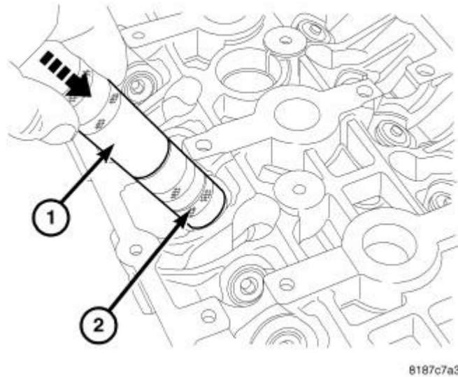
Fig. 156: Valve Installation
