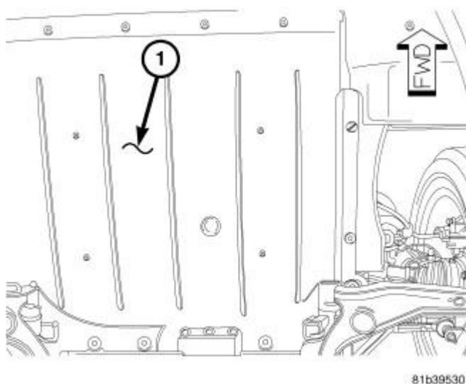
Fig. 225: Lower Silencer
