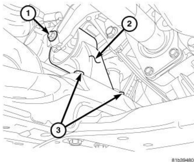
Fig. 236: Rear Engine Mount & Bolts Courtesy of CHRYSLER GROUP, LLC
