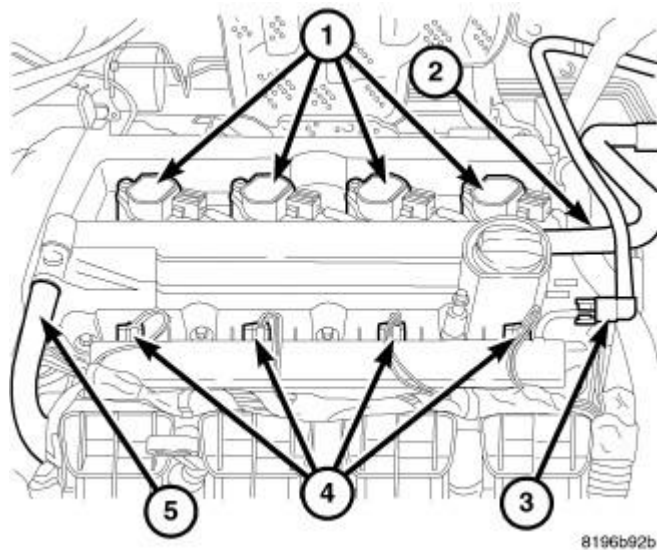
Fig. 44: Ignition Coils, Air Hose, Fuel Line, Injectors & PCV Hose Courtesy of CHRYSLER GROUP, LLC
