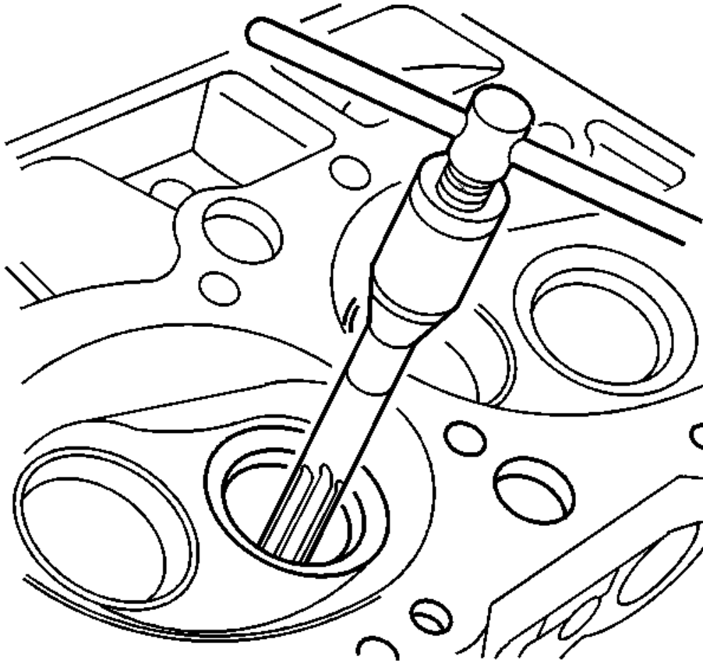
Fig. 366: Reaming Valve Guide Courtesy of GENERAL MOTORS CORP.
