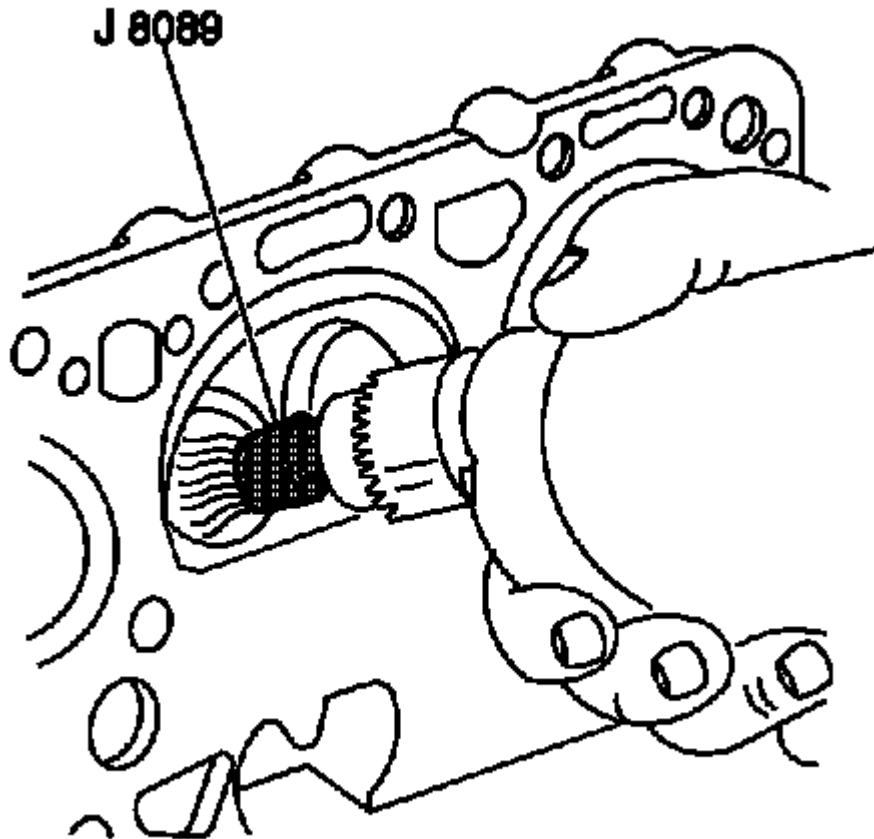
Fig. 357: Removing Carbon From Combustion Chambers Courtesy of GENERAL MOTORS CORP.
