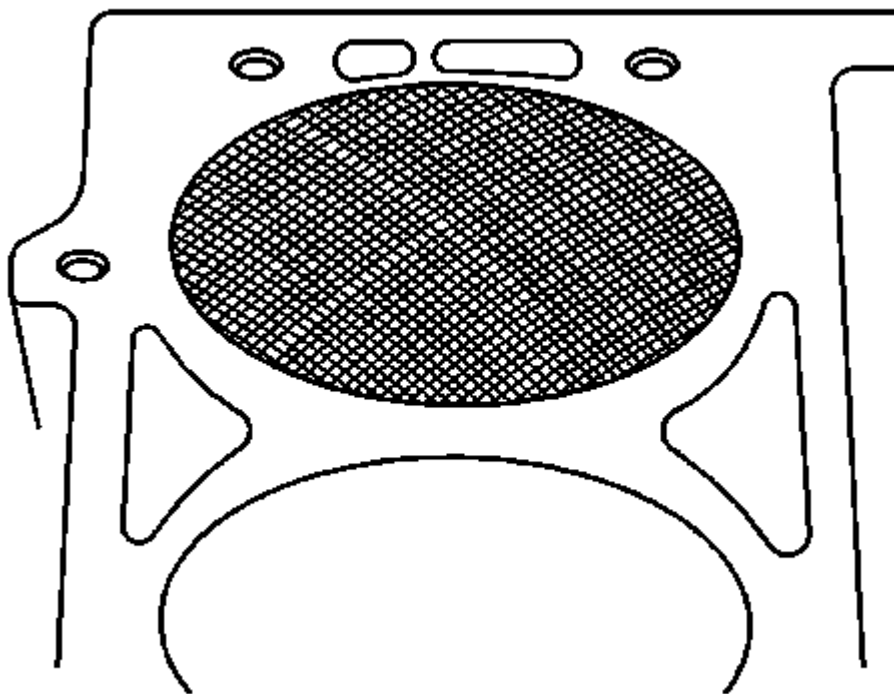
Fig. 302: Identifying Cylinder Bore Cross Hatch Pattern Courtesy of GENERAL MOTORS CORP.
