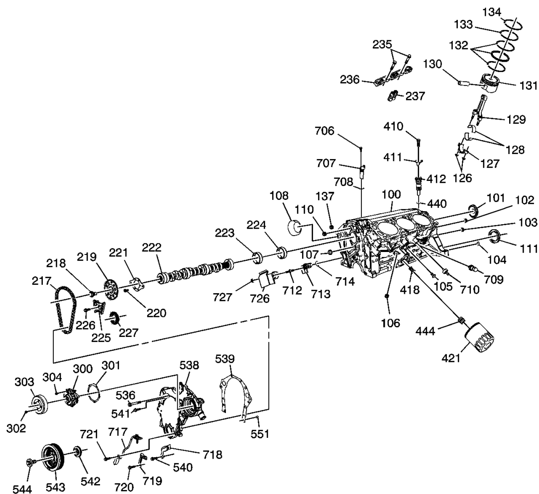
Fig. 3: Engine Block and Components Courtesy of GENERAL MOTORS CORP.
