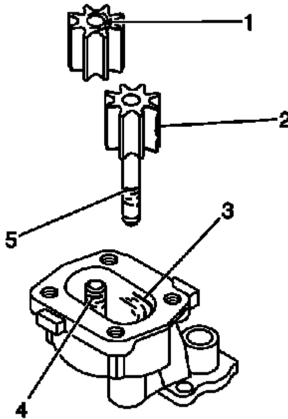
Fig. 378: Inspecting Oil Pump Housing & Gears, Idler Shaft, & Drive Gear Shaft Courtesy of GENERAL MOTORS CORP.
