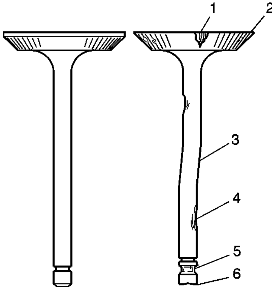
Fig. 361: Identifying Inspection Points For Valves Damage Courtesy of GENERAL MOTORS CORP.
