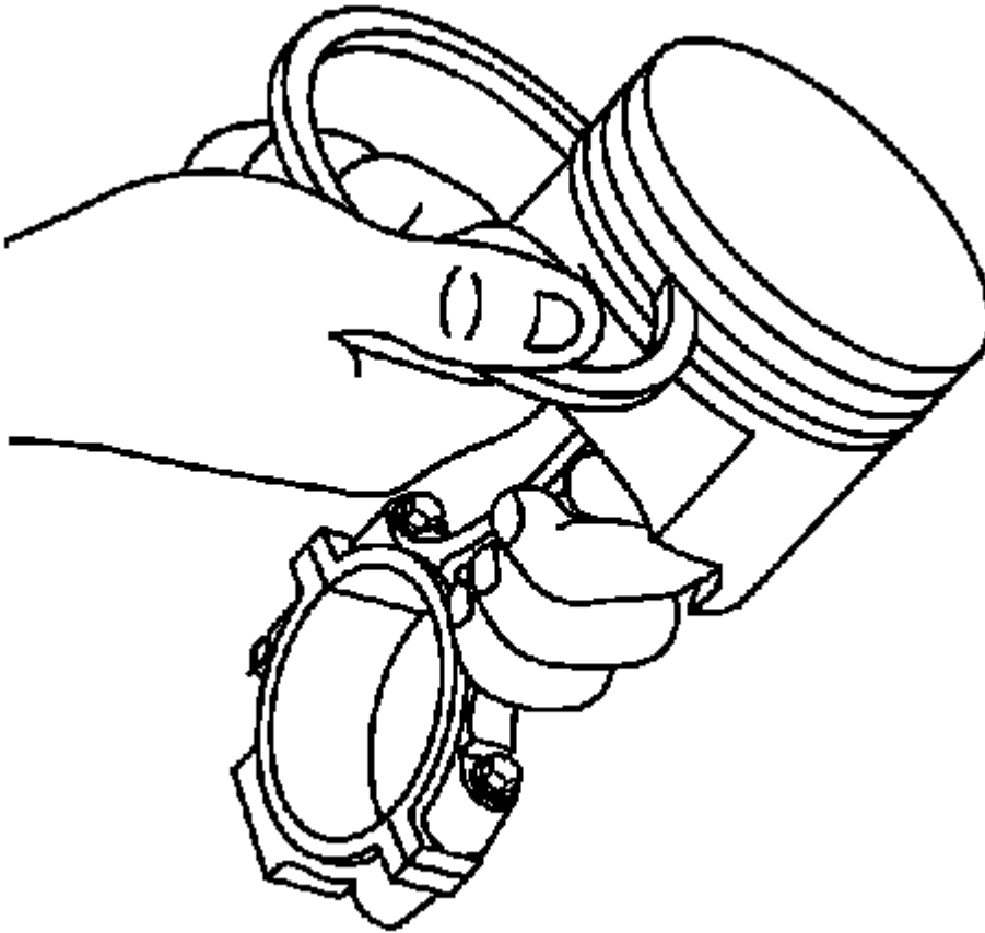
Fig. 327: Inserting Piston Ring Into Ring Groove Courtesy of GENERAL MOTORS CORP.
