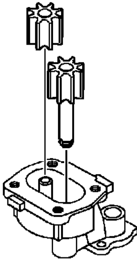
Fig. 384: View Of Oil Pump Drive Gear & Driven Gear Courtesy of GENERAL MOTORS CORP.
