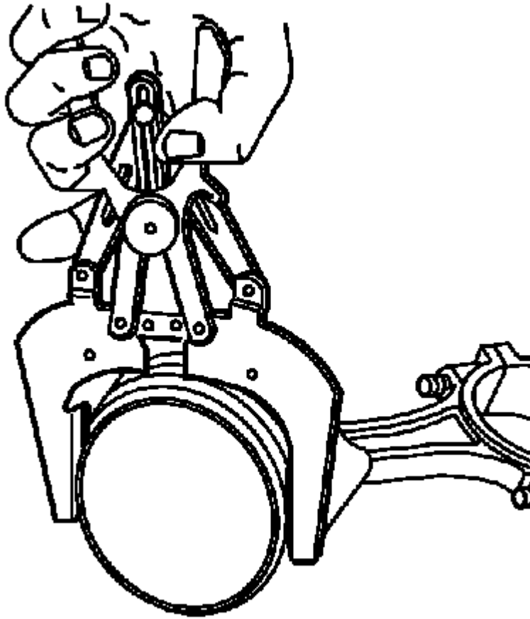
Fig. 325: Cleaning The Piston Ring Grooves With Suitable Ring Groove Cleaning Tool Courtesy of GENERAL MOTORS CORP.
