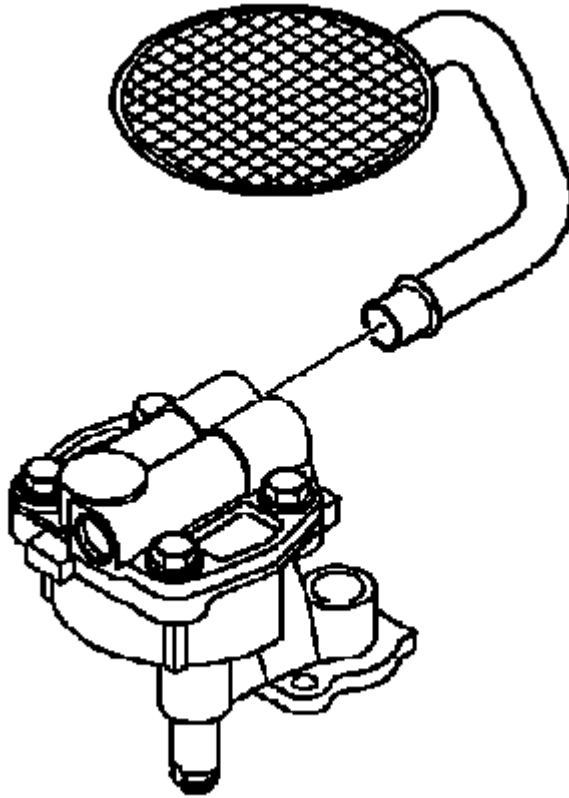
Fig. 373: View Of Oil Pump Screen
