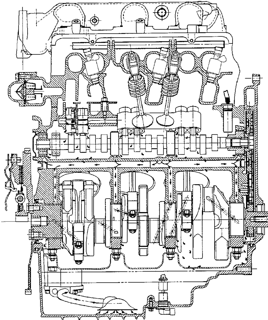
Fig. 491: Right View Of Engine Courtesy of GENERAL MOTORS CORP.
