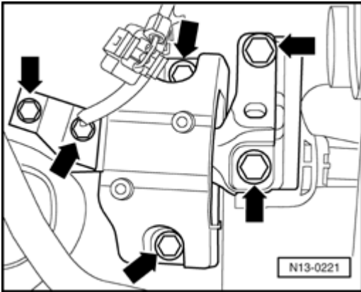
Fig. 66: Locating Securing Bolts From Assembly Mounting/Engine Bracket, Assembly Mounting/Body And Assembly Mounting Bracket/Body
