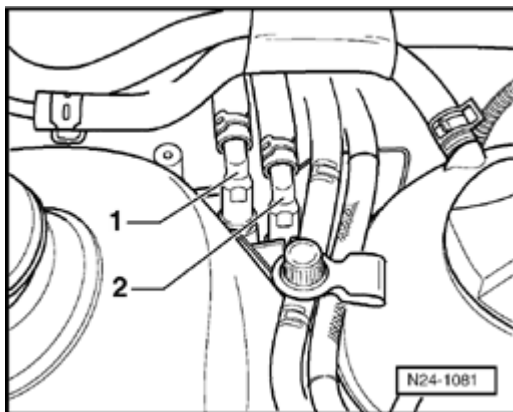
Fig. 6: Identifying Supply Line And Return Line
