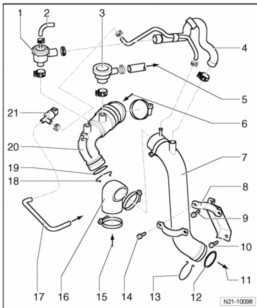
Fig. 214: Turbocharger With Attachments, Assembly Overview - Part II Courtesy of VOLKSWAGEN UNITED STATES, INC.
