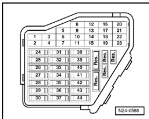
Fig. 163: Identifying Main Fuse Panel
