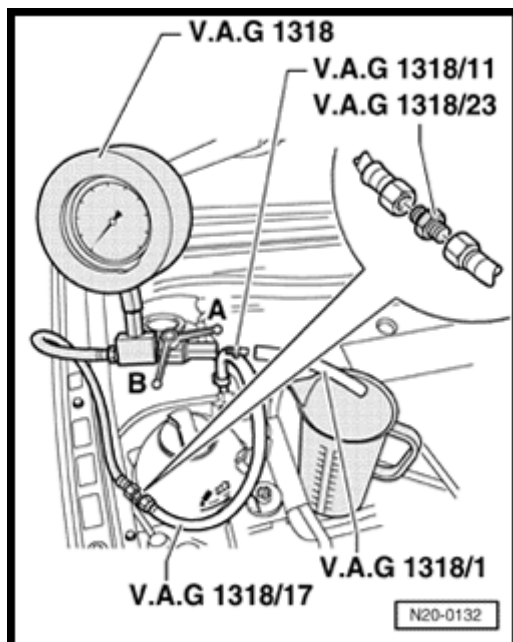
Fig. 183: Pressure Gauge V.A.G 1318 Connections
