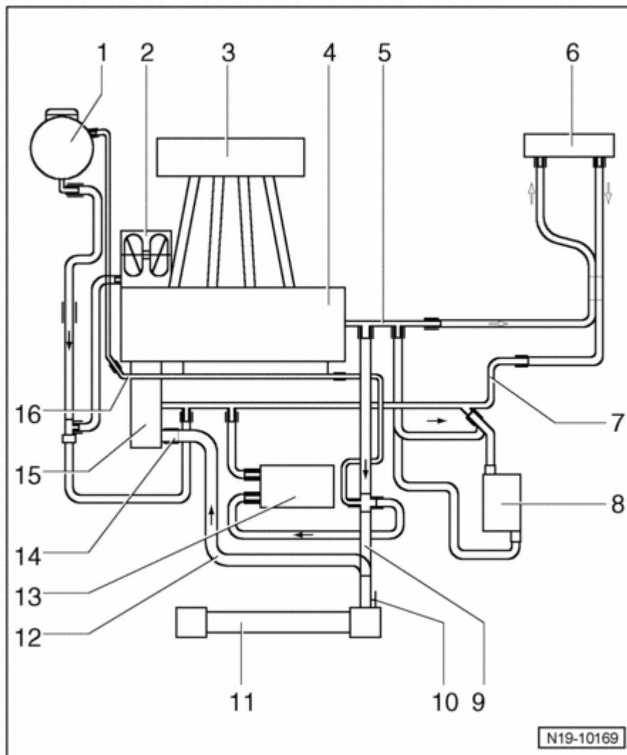
Fig. 138: Coolant Hose Connection Diagram - Vehicles With Engine Code AWP (Manual Transmission), AWW (Manual And Automatic Transmission)
