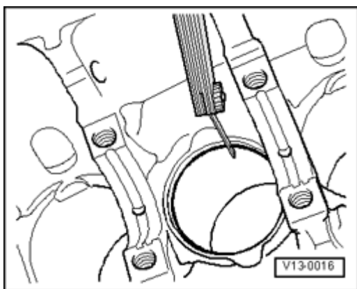
Fig. 49: Checking Piston Ring Gap
