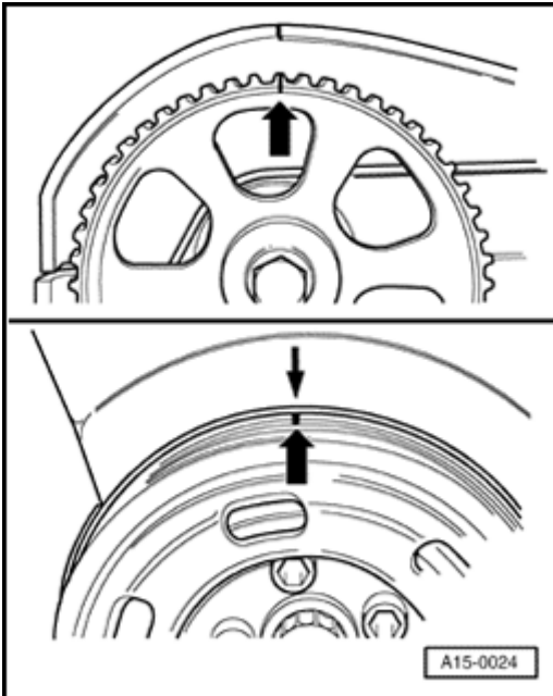
Fig. 74: Marking On Camshaft Gear Aligned With Marking On Cylinder Head Cover Courtesy of VOLKSWAGEN UNITED STATES, INC.
