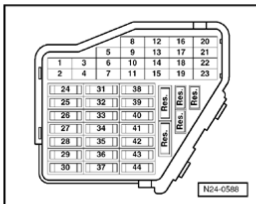
Fig. 194: Identifying Main Fuse Panel
