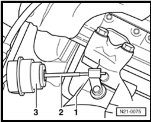
Fig. 228: Boost Pressure Regulator Valve And Actuator Rod Courtesy of VOLKSWAGEN UNITED STATES, INC.
