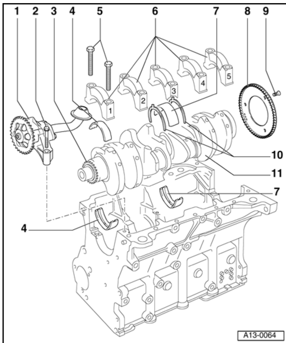
Fig. 46: Crankshaft, Assembly Overview
