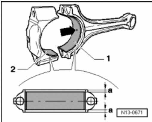
Fig. 57: Installation Position Of Bearing Shells Courtesy of VOLKSWAGEN UNITED STATES, INC.
