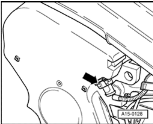
Fig. 103: Locating Connector At Camshaft Position Sensor G40 Courtesy of VOLKSWAGEN UNITED STATES, INC.
