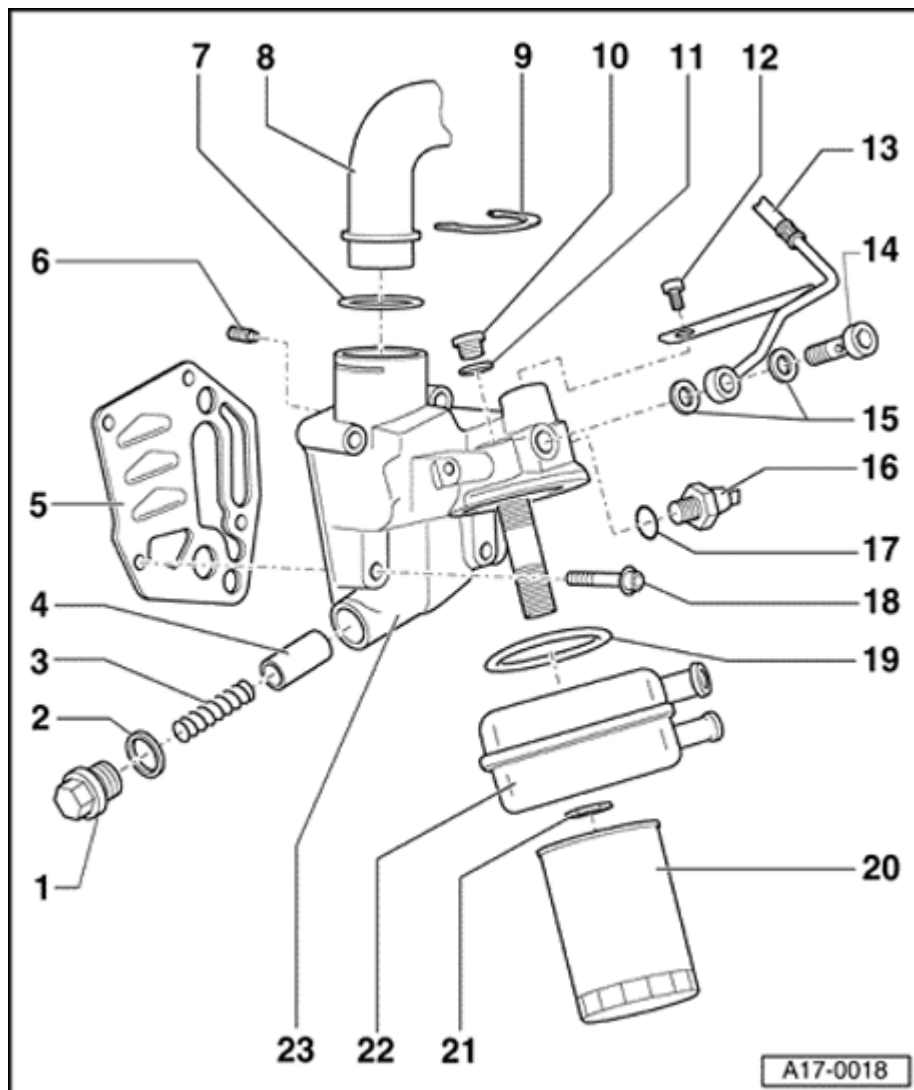
Fig. 127: Lubrication System Components, Assembly Overview - Part II Courtesy of VOLKSWAGEN UNITED STATES, INC.
