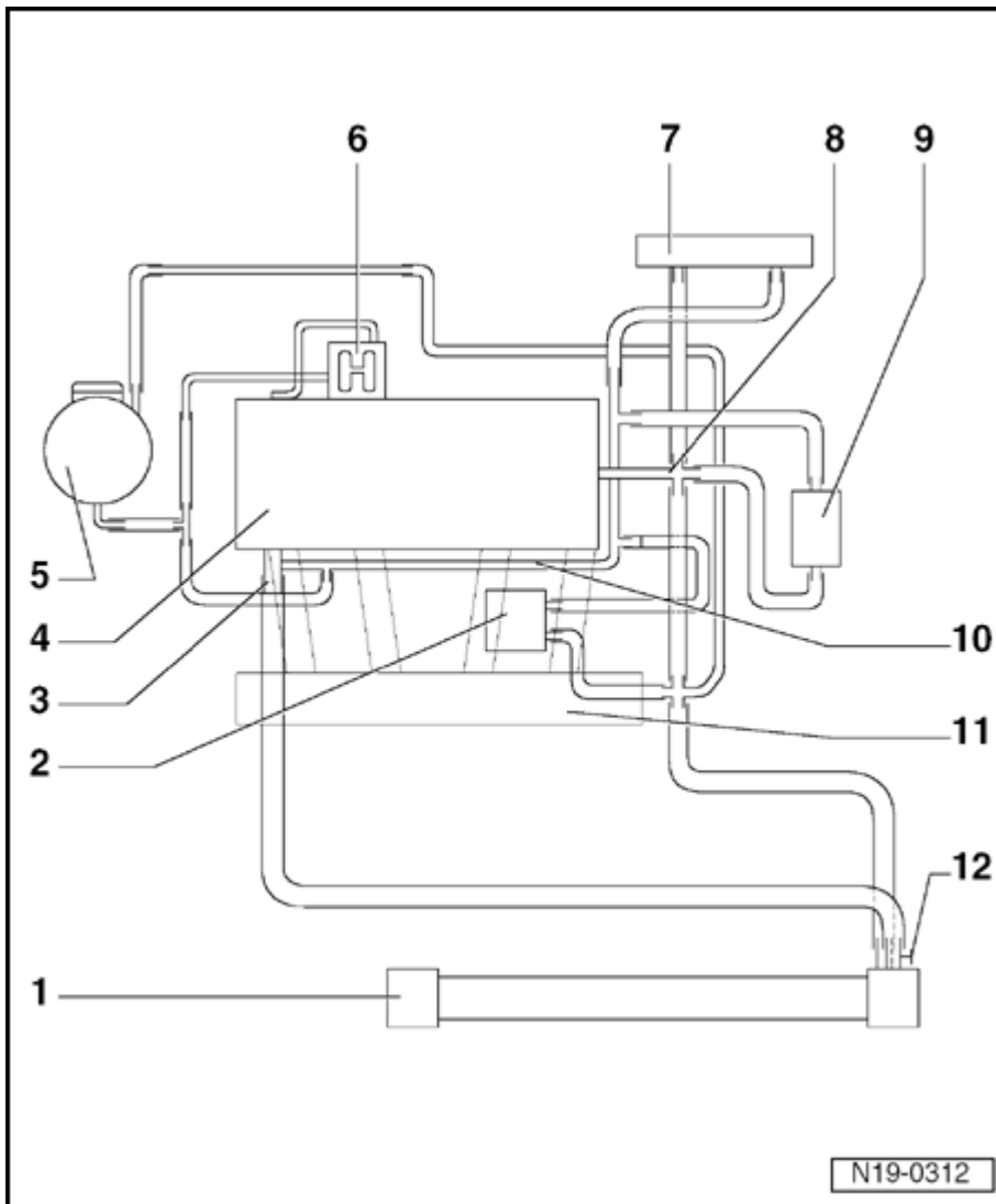
Fig. 137: Coolant Hose Connection Diagram - Vehicles With Engine Code AWD Courtesy of VOLKSWAGEN UNITED STATES, INC.
