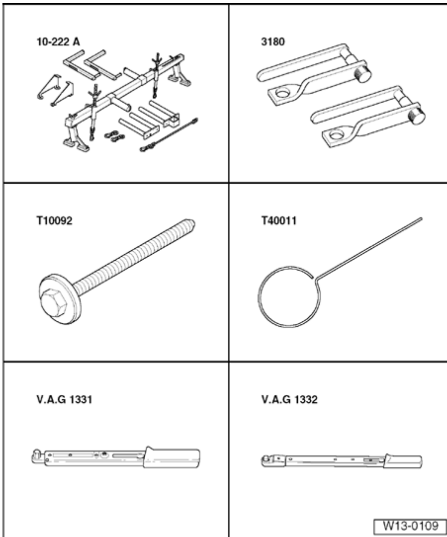
Fig. 61: Identifying Special Tools - Toothed Belt, Removing, Installing And Tensioning Courtesy of VOLKSWAGEN UNITED STATES, INC.
