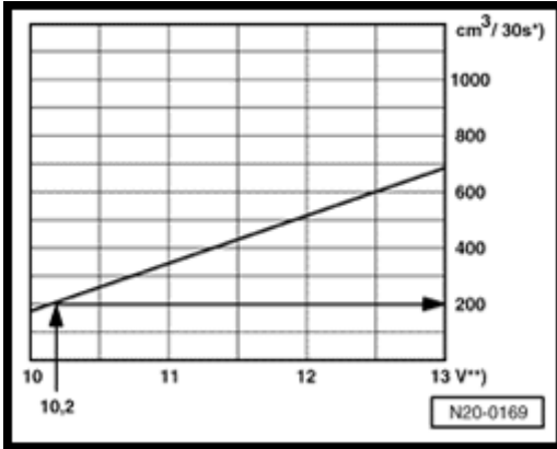
Fig. 180: Fuel Delivery Rate Graph
