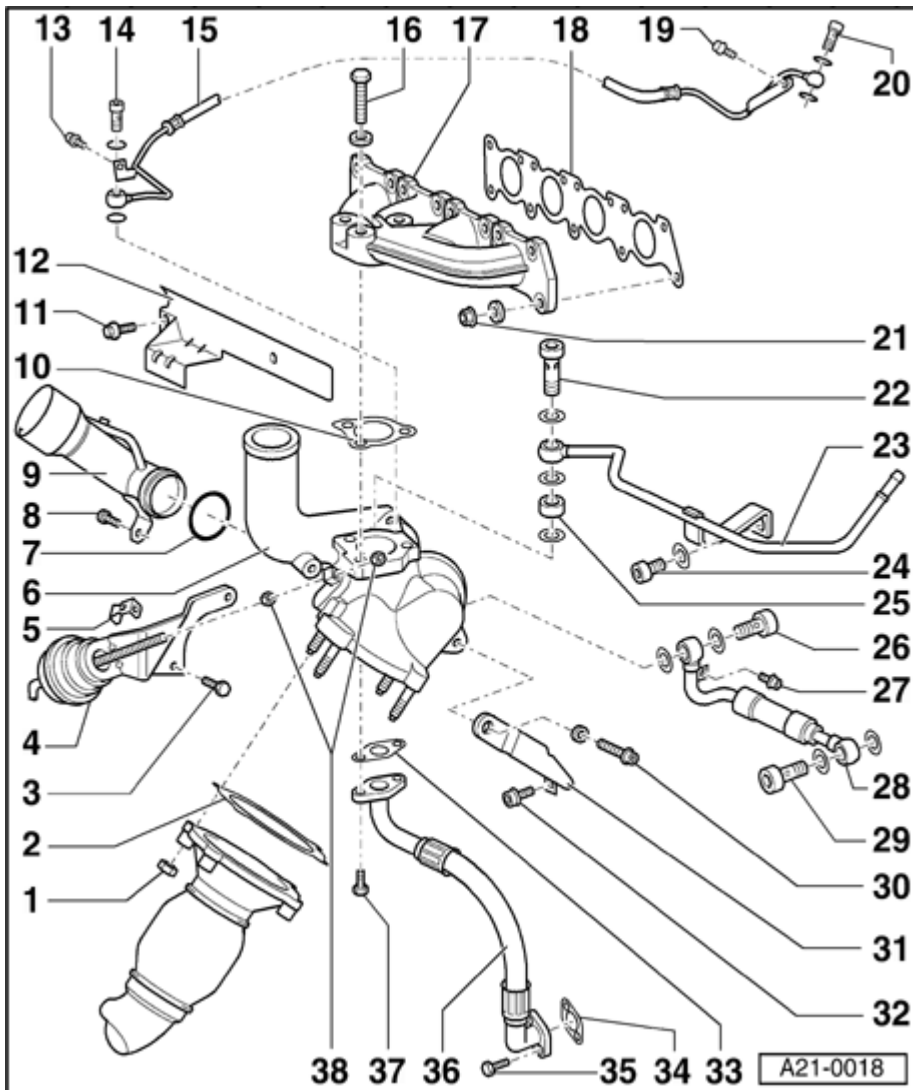
Fig. 213: Turbocharger With Attachments, Assembly Overview - Part I Courtesy of VOLKSWAGEN UNITED STATES, INC.
