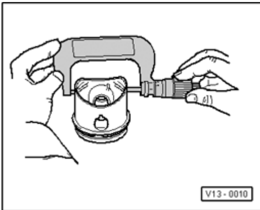
Fig. 51: Checking Piston Courtesy of VOLKSWAGEN UNITED STATES, INC.
