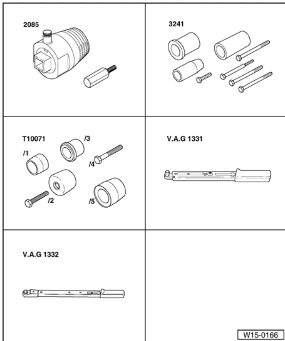
Fig. 95: Identifying Special Tools - Camshaft Position Sensor G40 Gasket, Removing Courtesy of VOLKSWAGEN UNITED STATES, INC.
