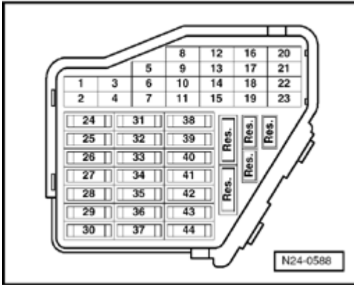
Fig. 187: Identifying Main Fuse Panel
