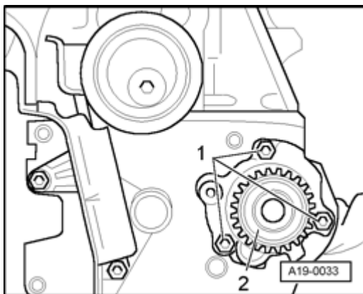
Fig. 150: Coolant Pump & Securing Bolts
