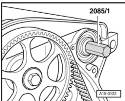
Fig. 97: Adapter 2085/1 Threaded In Camshaft
