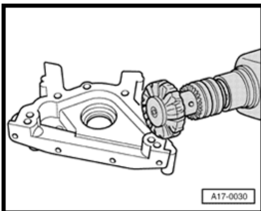
Fig. 38: Removing Sealant Remains On Sealing Flange With A Rotating Plastic Brush Courtesy of VOLKSWAGEN UNITED STATES, INC.
