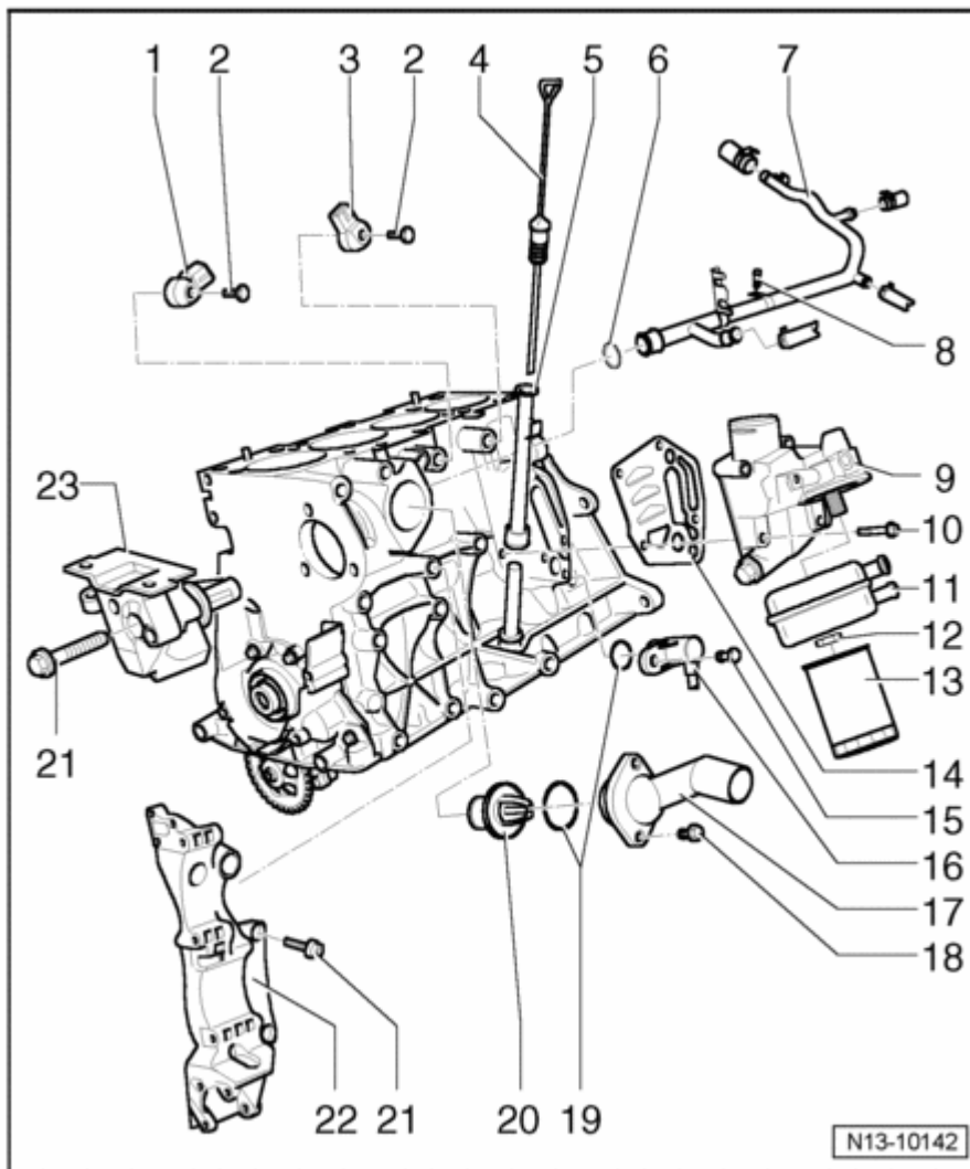
Fig. 22: Engine Assembly Overview II
