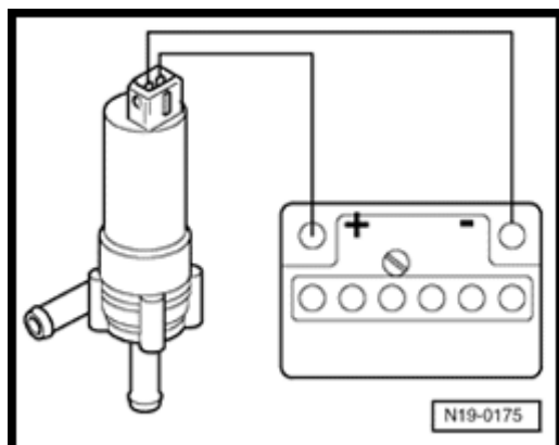
Fig. 157: Contacts Of After-Run Coolant Pump V51 Connected To Battery
