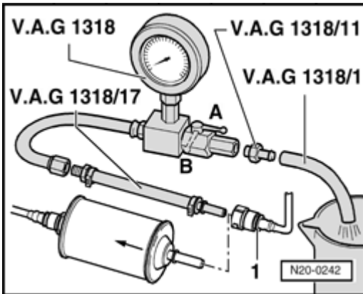
Fig. 181: Pressure Gauge V.A.G 1318 Connections (2 Of 2) Courtesy of VOLKSWAGEN UNITED STATES, INC.
