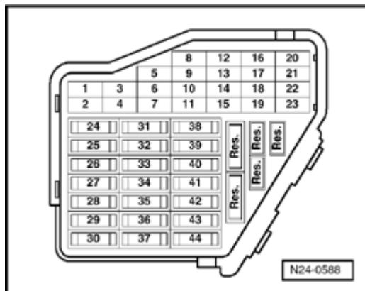
Fig. 193: Identifying Main Fuse Panel
