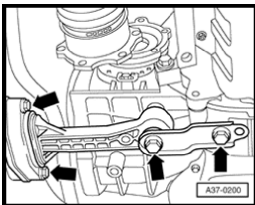
Fig. 7: Identifying Pendulum Support & Bolts
