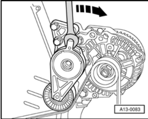
Fig. 24: Relieving Tension On Poly V-Belt Courtesy of VOLKSWAGEN UNITED STATES, INC.
