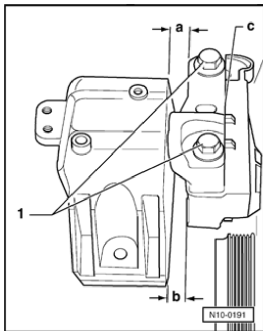
Fig. 14: Measuring Engine Mounting Courtesy of VOLKSWAGEN UNITED STATES, INC.
