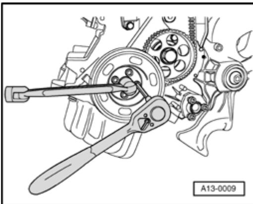
Fig. 67: Removing/Installing Vibration Damper/Belt Pulley
