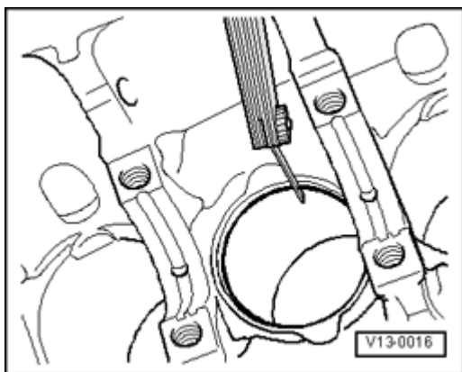
Fig. 54: Checking Piston Ring Gap
