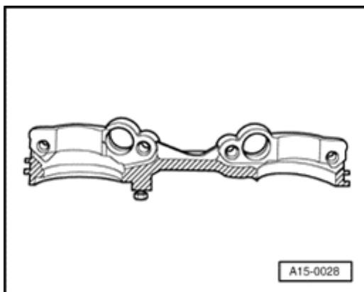
Fig. 114: Identifying Double Bearing Cap Sealant Application Area
