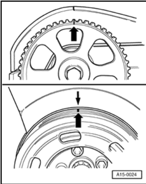
Fig. 90: Marking On Camshaft Gear Aligned With Marking On Cylinder Head Cover Courtesy of VOLKSWAGEN UNITED STATES, INC.
