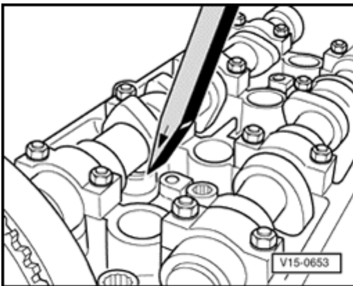
Fig. 104: Pressing Valve Lifter Downward Using Wedge Courtesy of VOLKSWAGEN UNITED STATES, INC.
