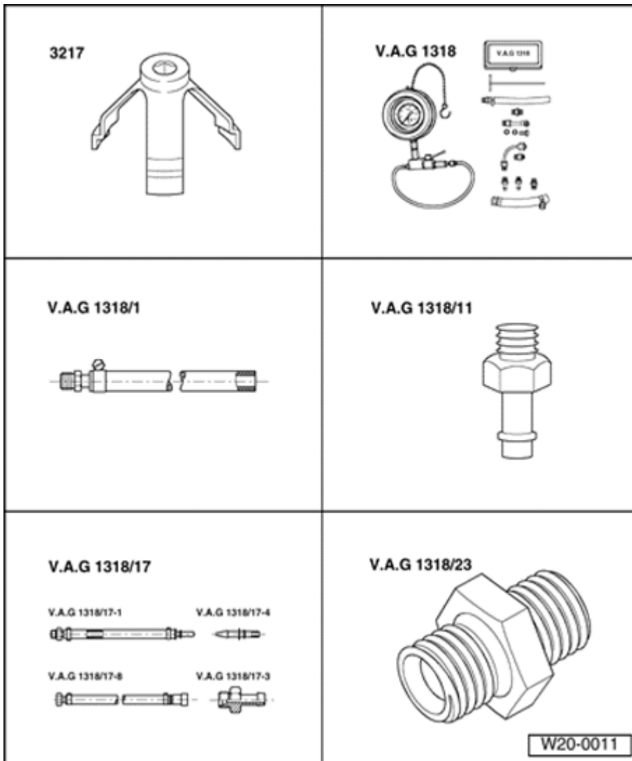
Fig. 172: Identifying Special Tools - Fuel Pump, Checking (1 Of 2) Courtesy of VOLKSWAGEN UNITED STATES, INC.
