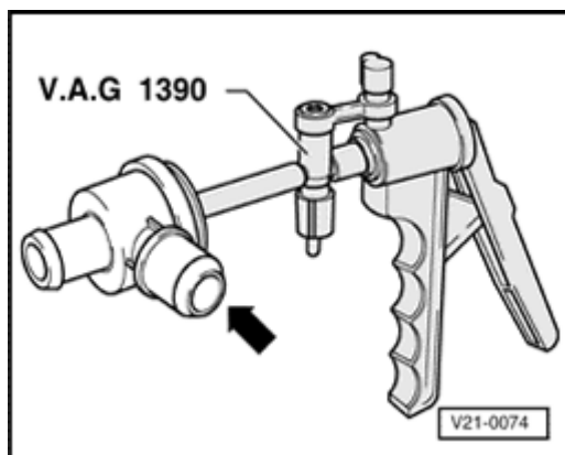
Fig. 230: Hand Vacuum Pump V.A.G 1390 Connect To Vacuum Connection Of Deceleration Shut-Off Valve In Proper Direction Courtesy of VOLKSWAGEN UNITED STATES, INC.
