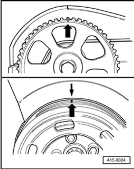
Fig. 106: Marking On Camshaft Gear Aligned With Marking On Cylinder Head Cover Courtesy of VOLKSWAGEN UNITED STATES, INC.
