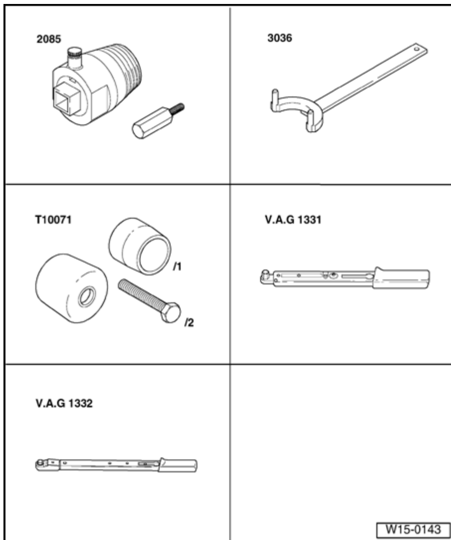
Fig. 89: Identifying Special Tools - Oil Seal At Camshaft Gear, Removing And Installing Courtesy of VOLKSWAGEN UNITED STATES, INC.
