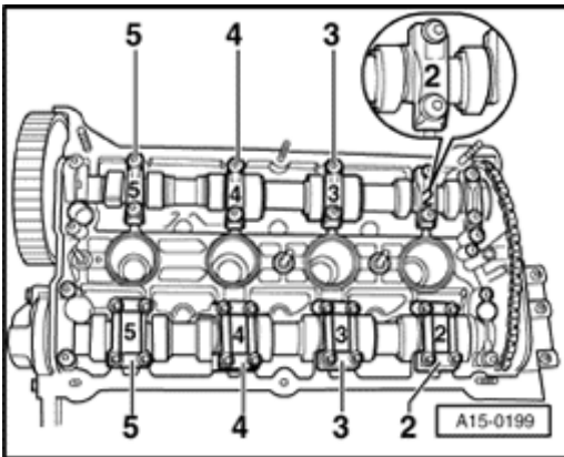
Fig. 112: Identifying Bearing Cap Positions Courtesy of VOLKSWAGEN UNITED STATES, INC.
