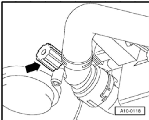
Fig. 141: Locating Radiator Drain Plug
