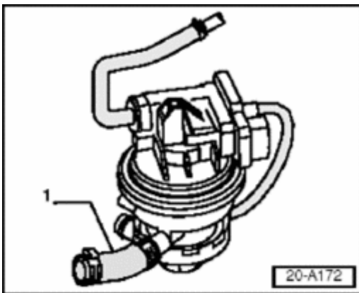
Fig. 211: Identifying LDP Outlet EVAP Side
