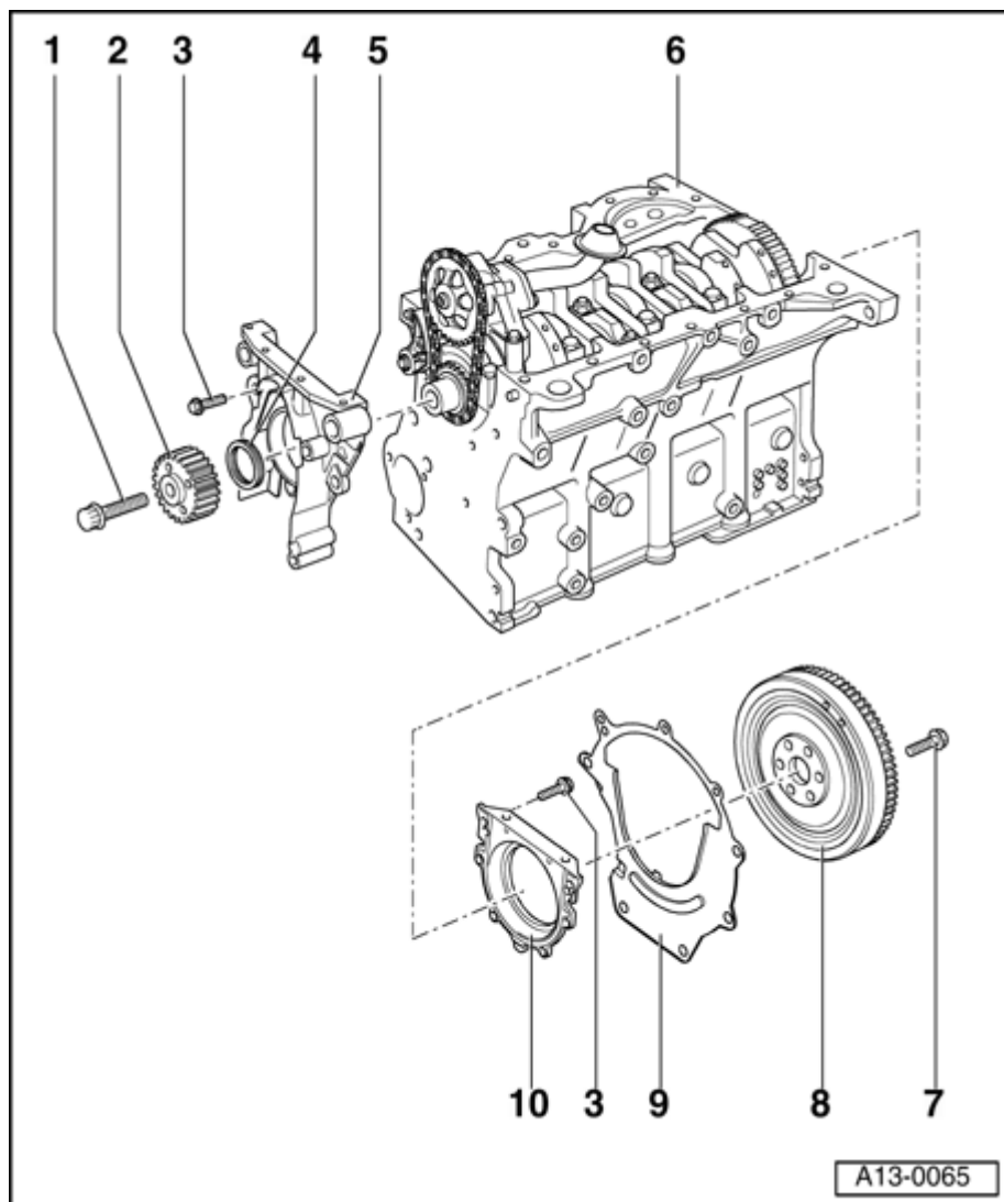
Fig. 28: Identifying Sealing Flanges And Flywheel/Drive Plate Courtesy of VOLKSWAGEN UNITED STATES, INC.
