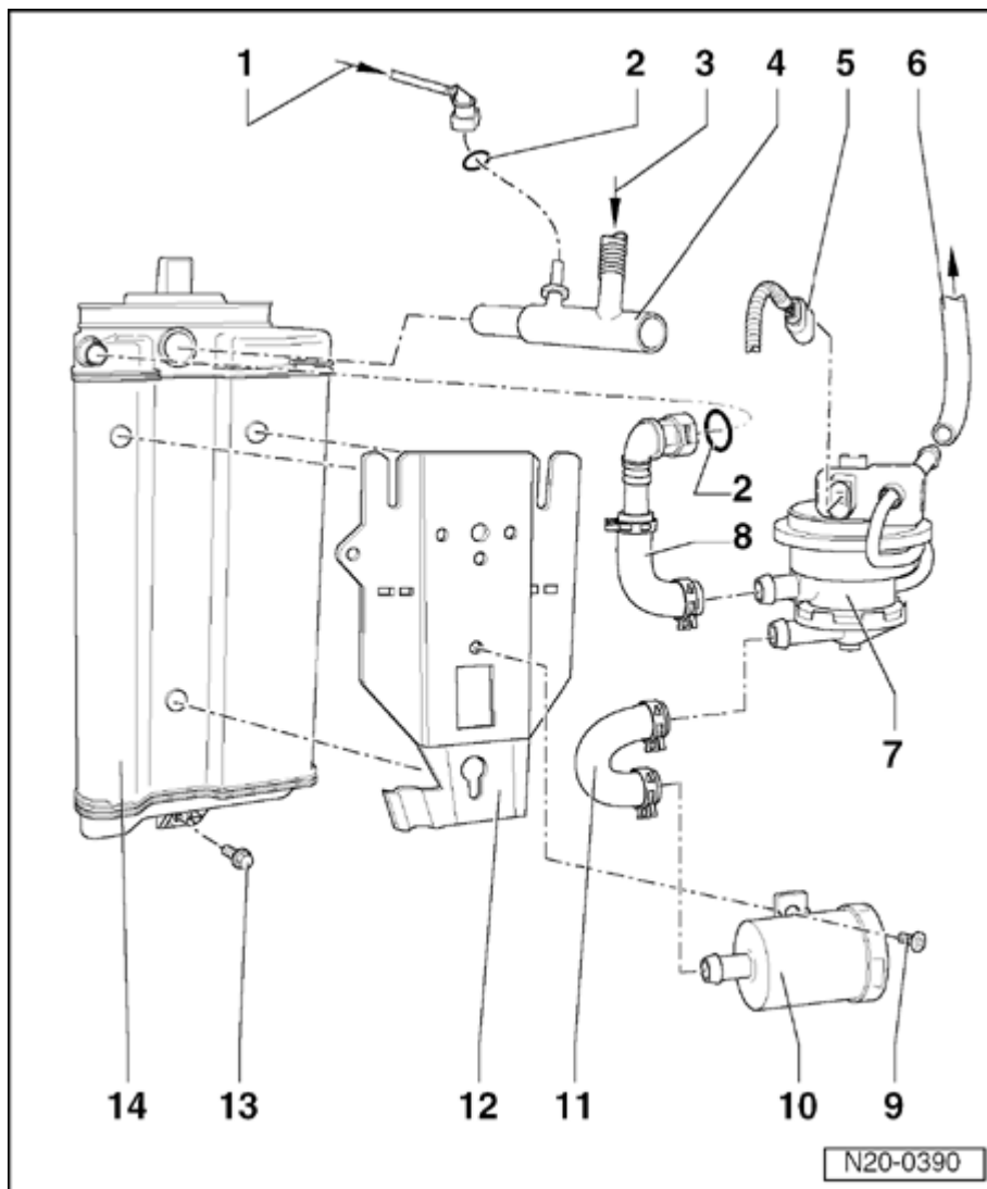
Fig. 191: EVAP Canister System, Assembly Overview
