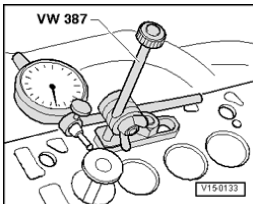
Fig. 119: Identifying Special Tool - VW 387 Installed
