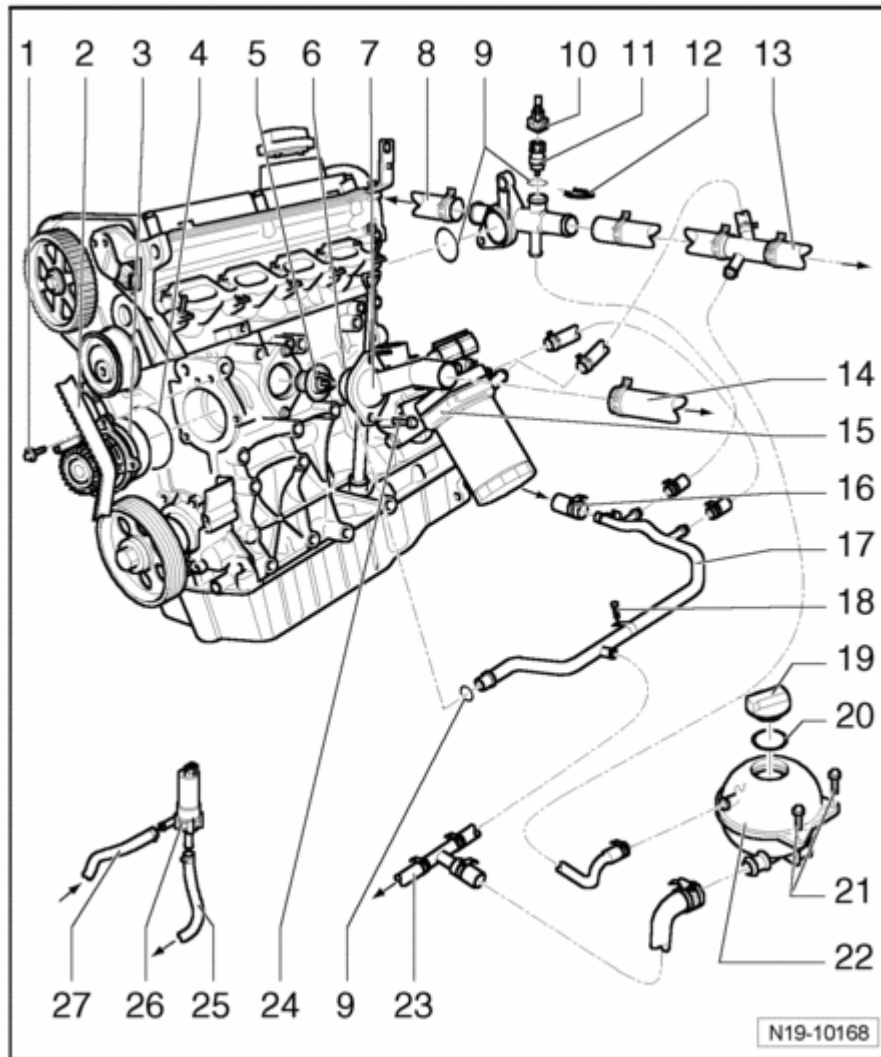
Fig. 136: Cooling System Components (On Engine), Assembly Overview Courtesy of VOLKSWAGEN UNITED STATES, INC.
