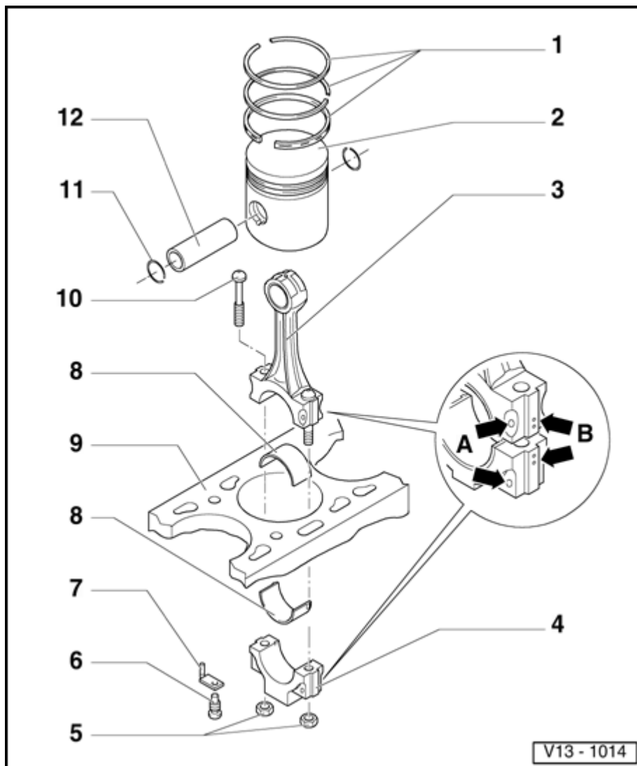
Fig. 48: Pistons And Connecting Rods (Engine Code AWD), Assembly Overview Courtesy of VOLKSWAGEN UNITED STATES, INC.
