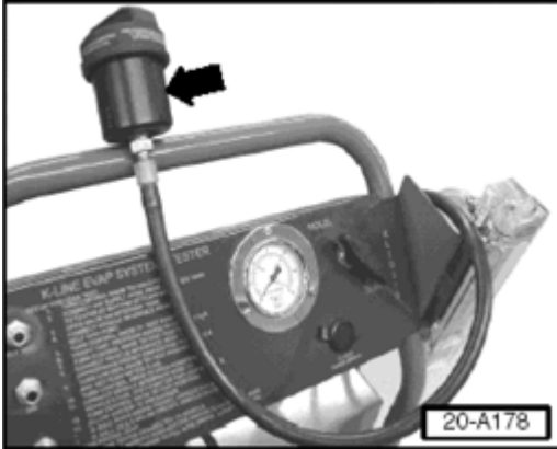
Fig. 202: Fuel Cap Receiver Connect To Hose
