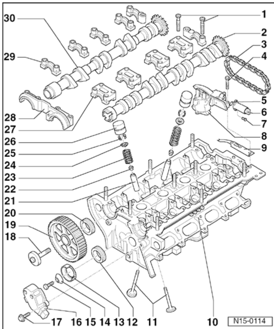
Fig. 81: Valvetrain, Assembly Overview
