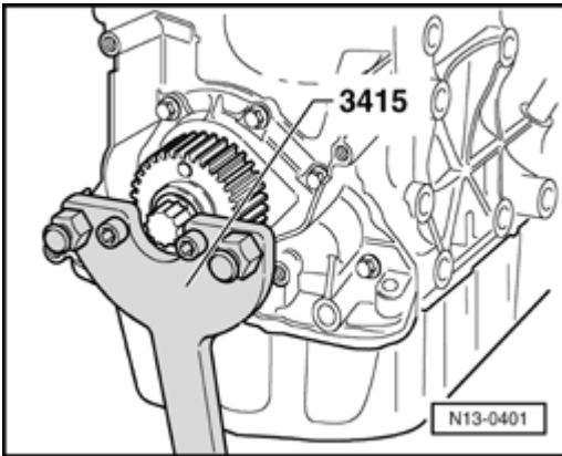
Fig. 40: Counter-Holding Crankshaft Toothed Belt Sprocket With 3415
