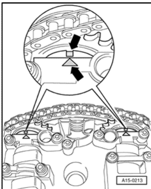
Fig. 116: Checking Position Of Camshafts To Each Other Courtesy of VOLKSWAGEN UNITED STATES, INC.
