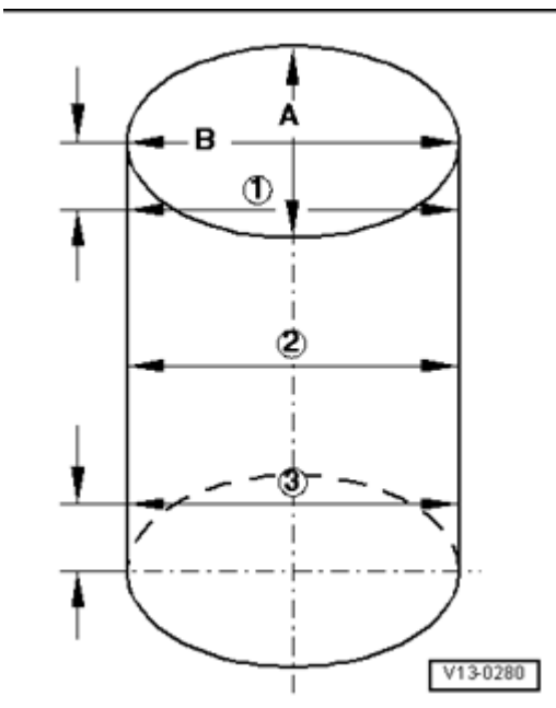
Fig. 58: Checking Cylinder Bores
