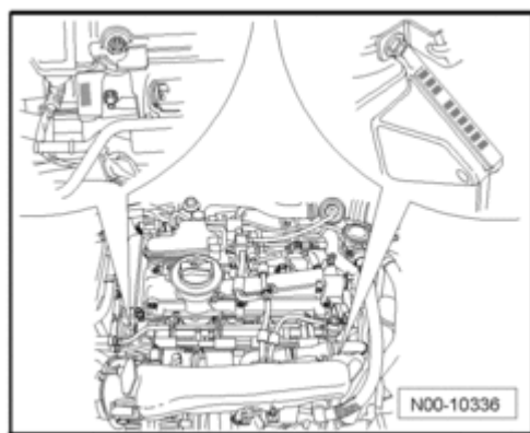
Fig. 1: Locating Engine Number
