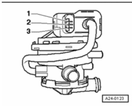
Fig. 196: Locating 3-Pin Connector At Fuel System Leak Detection Pump V144 Courtesy of VOLKSWAGEN UNITED STATES, INC.
