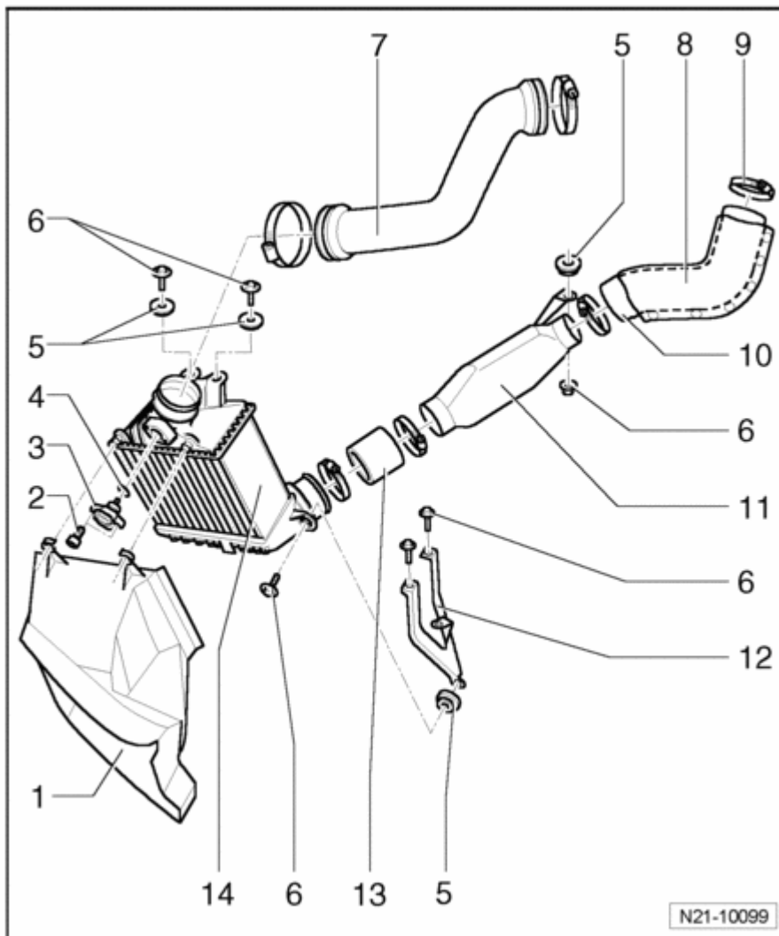
Fig. 215: Charge Air Cooler Components, Assembly Overview Courtesy of VOLKSWAGEN UNITED STATES, INC.
