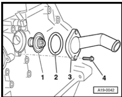
Fig. 153: Identifying Thermostat & Fasteners
