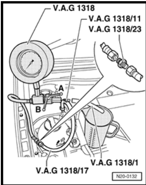
Fig. 179: Pressure Gauge V.A.G 1318 Connections (1 Of 2) Courtesy of VOLKSWAGEN UNITED STATES, INC.
