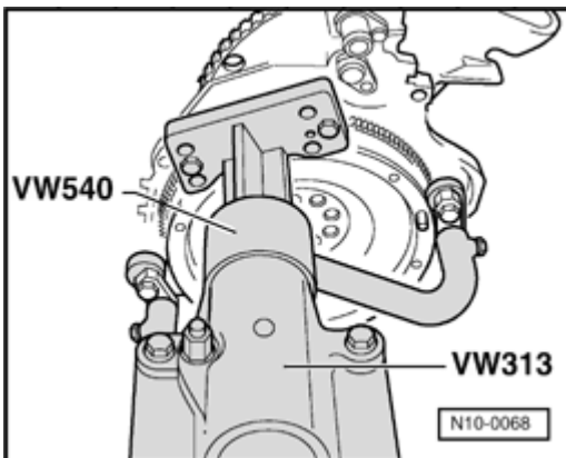
Fig. 12: Identifying Engine Fastened Using Holding Fixture VW 540 & Holding Fixture VW 313 Courtesy of VOLKSWAGEN UNITED STATES, INC.
