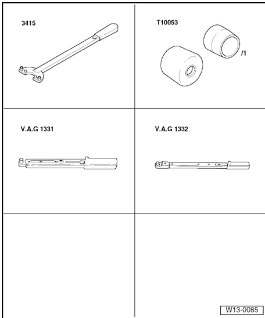
Fig. 36: Identifying Special Tools - Removing And Installing Sealing Flange (Belt Pulley Side) Courtesy of VOLKSWAGEN UNITED STATES, INC.
