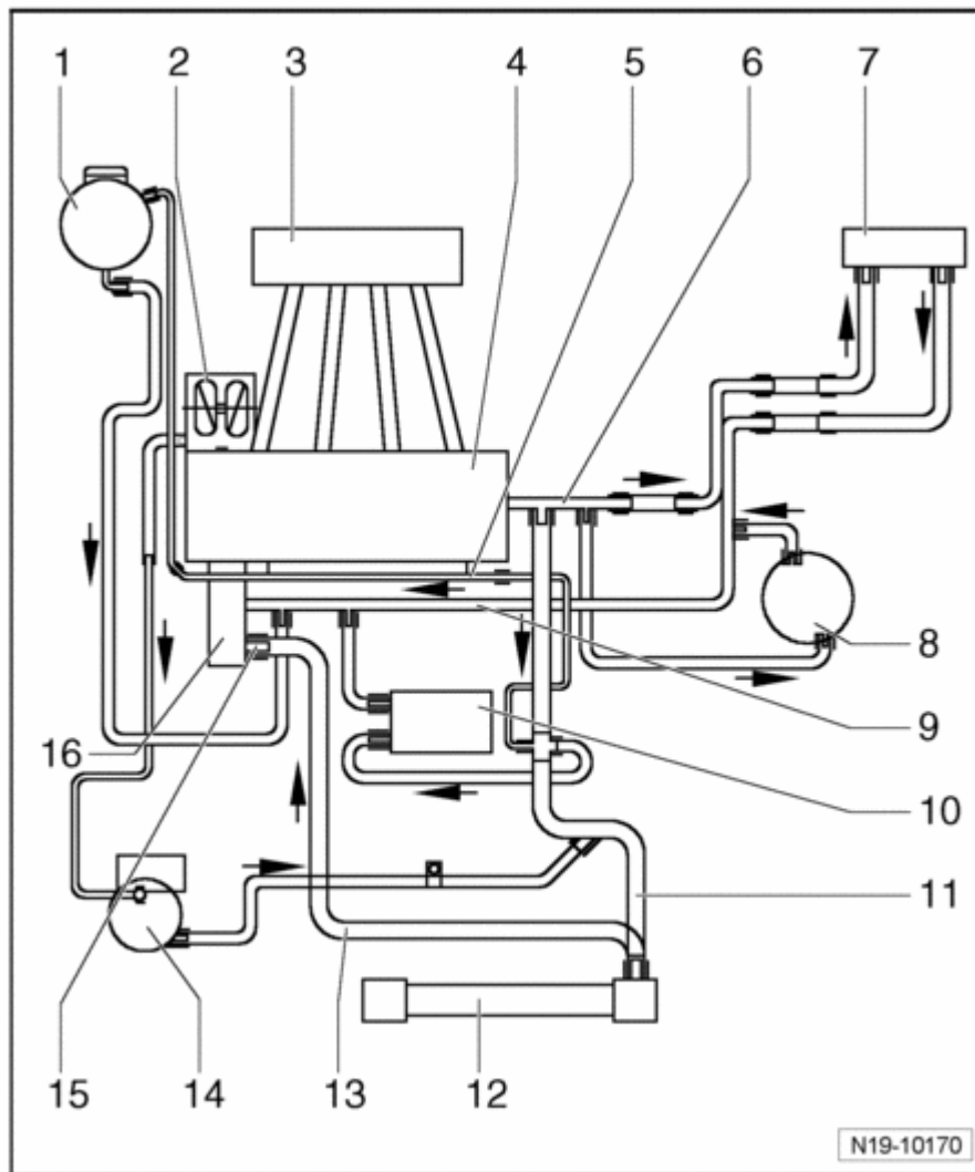
Fig. 139: Coolant Hose Connection Diagram - Vehicles With Engine Code AWP (Automatic Transmission)
