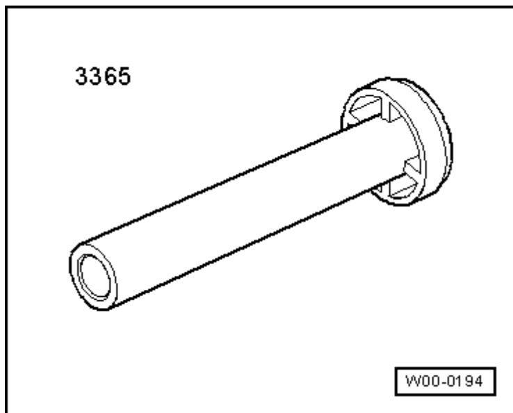
Fig. 121: Valve Stem Seal Driver 3365
