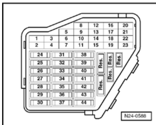
Fig. 80: Identifying Main Fuse Panel
