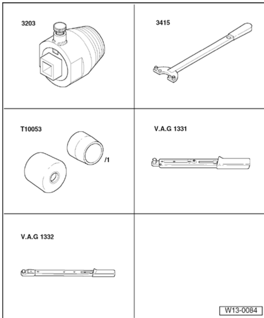
Fig. 29: Identifying Special Tools - Replacing Crankshaft Seal, Ribbed Belt Side Courtesy of VOLKSWAGEN UNITED STATES, INC.
