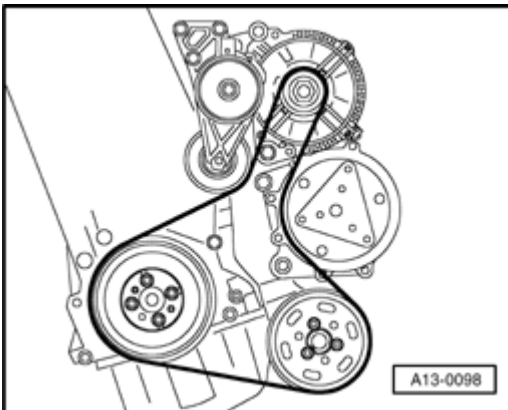
Fig. 27: Identifying Belt Drive For Vehicles With Air Conditioning Courtesy of VOLKSWAGEN UNITED STATES, INC.
