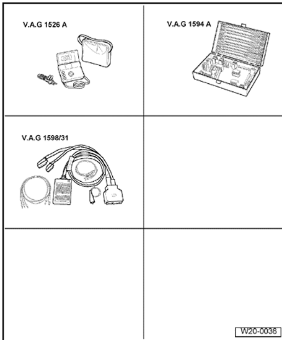
Fig. 186: Identifying Special Tools - Throttle Position Sensor G79 And Accelerator Pedal Position Sensor 2 G185 , Checking
