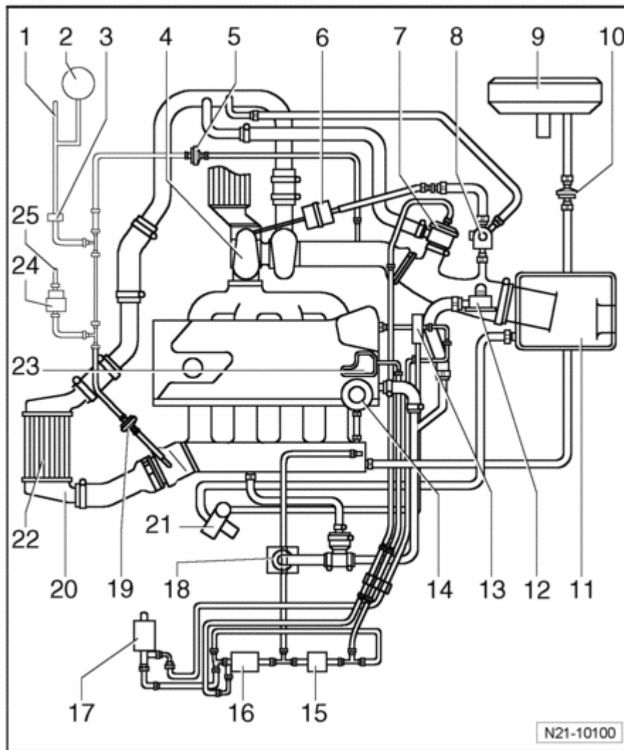
Fig. 216: Exhaust Turbocharging System (Engine Code AWD), Overview Courtesy of VOLKSWAGEN UNITED STATES, INC.
