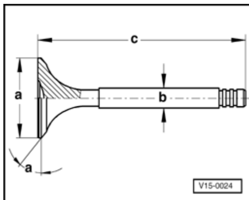
Fig. 84: Identifying Valve Dimensions
