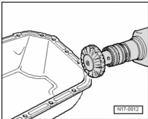
Fig. 130: Removing Sealant Residue From Oil Pan With A Rotating Brush Courtesy of VOLKSWAGEN UNITED STATES, INC.
