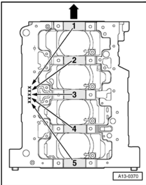
Fig. 47: Cylinder Block Crankshaft Bearing Shells Identification Courtesy of VOLKSWAGEN UNITED STATES, INC.
