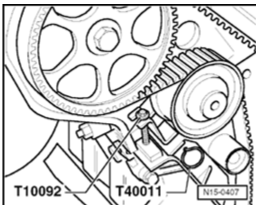
Fig. 72: Tensioning Bolt T10092 And Locking Pin T40011 Installed
