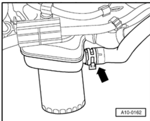
Fig. 142: Locating Oil Cooler Coolant Hose
