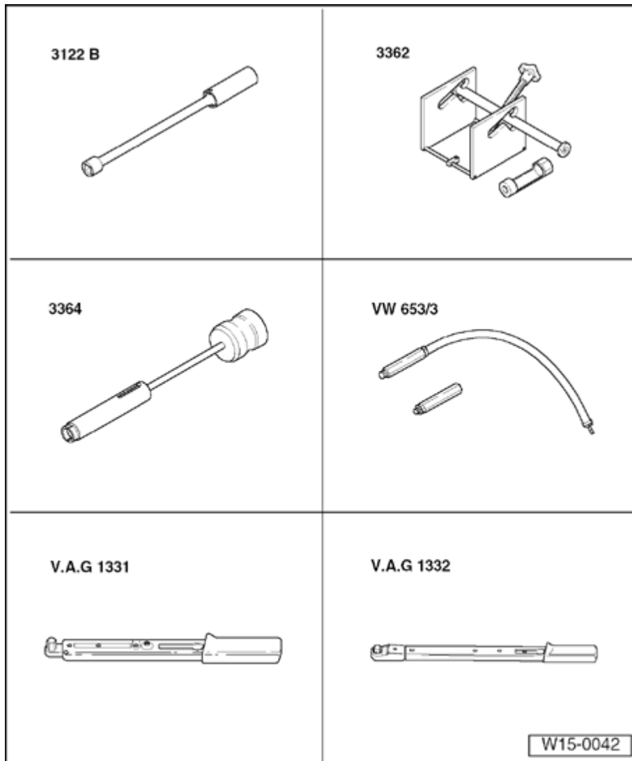
Fig. 120: Identifying Special Tools - Valve Stem Seals, Replacing Courtesy of VOLKSWAGEN UNITED STATES, INC.
