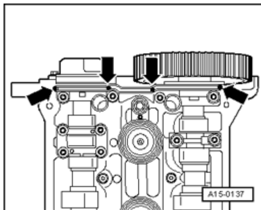
Fig. 85: Double Bearing Cap Contact Surface Sealant Application Areas
