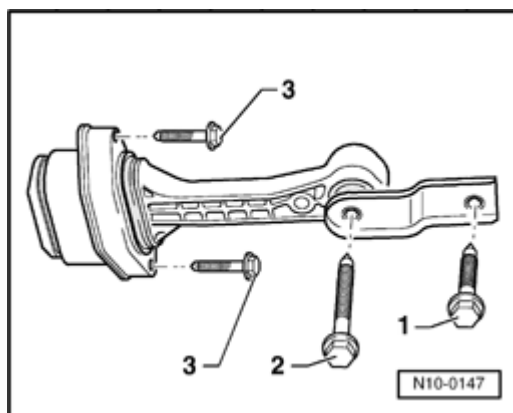
Fig. 18: Identifying Pendulum Support & Bolts Courtesy of VOLKSWAGEN UNITED STATES, INC.
