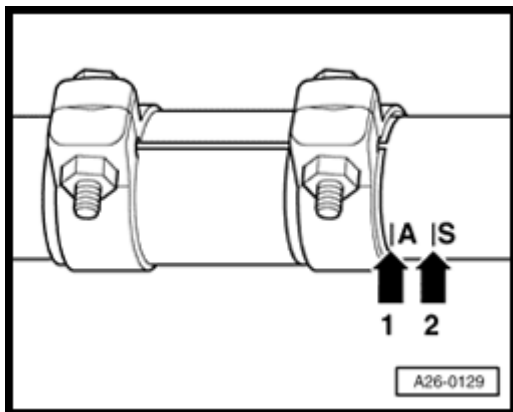
Fig. 239: Installation Position Of Double Clamp
