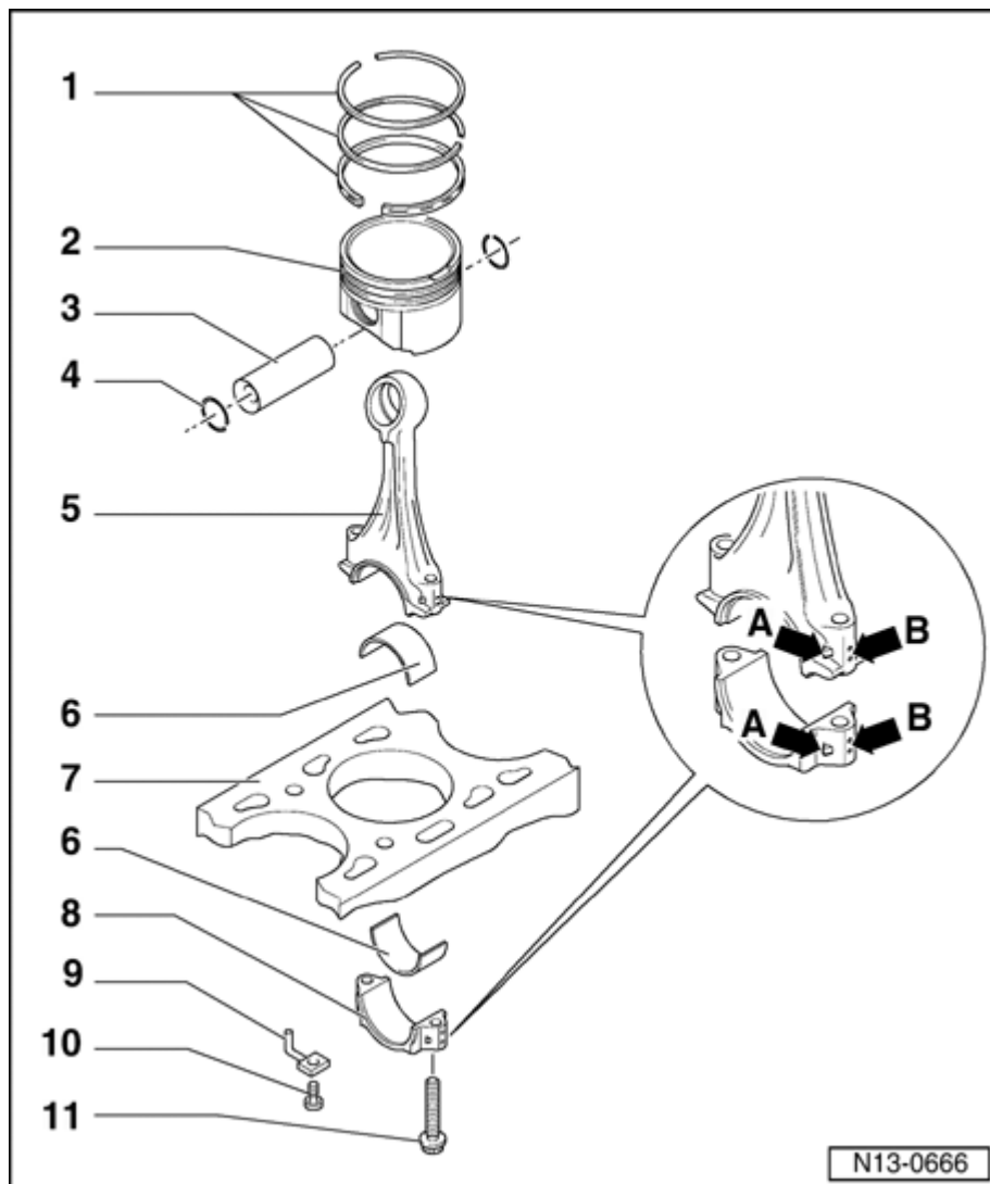
Fig. 53: Pistons And Connecting Rods (Engine Code AWD, AWW), Assembly Overview Courtesy of VOLKSWAGEN UNITED STATES, INC.
