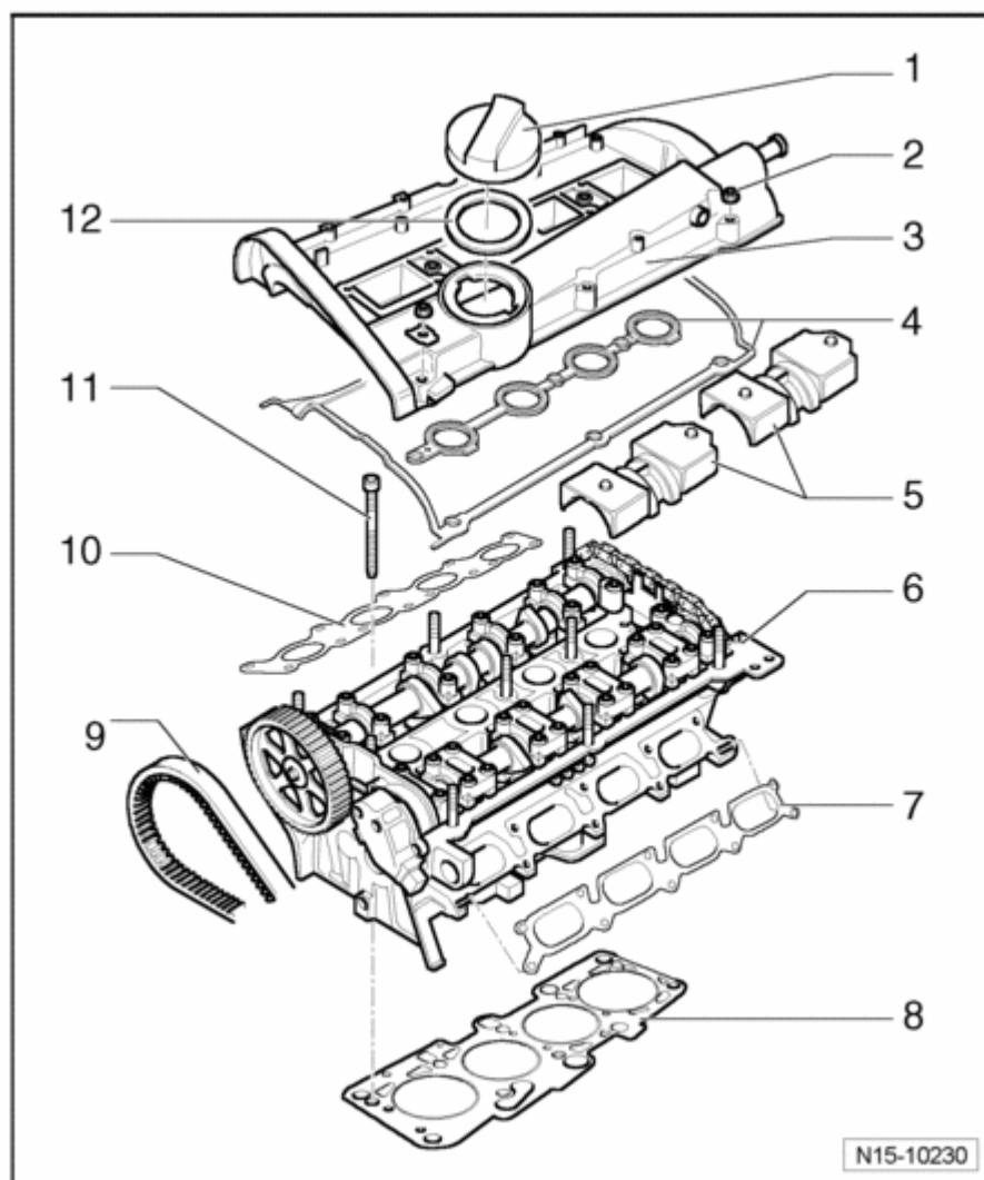
Fig. 59: Cylinder Head, Assembly Overview
