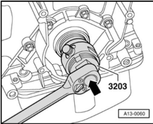
Fig. 32: Identifying Special Tool - 3203
