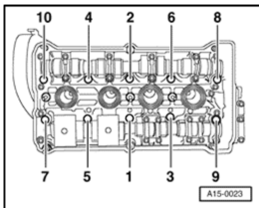
Fig. 78: Cylinder Head Bolt Position Numbers
