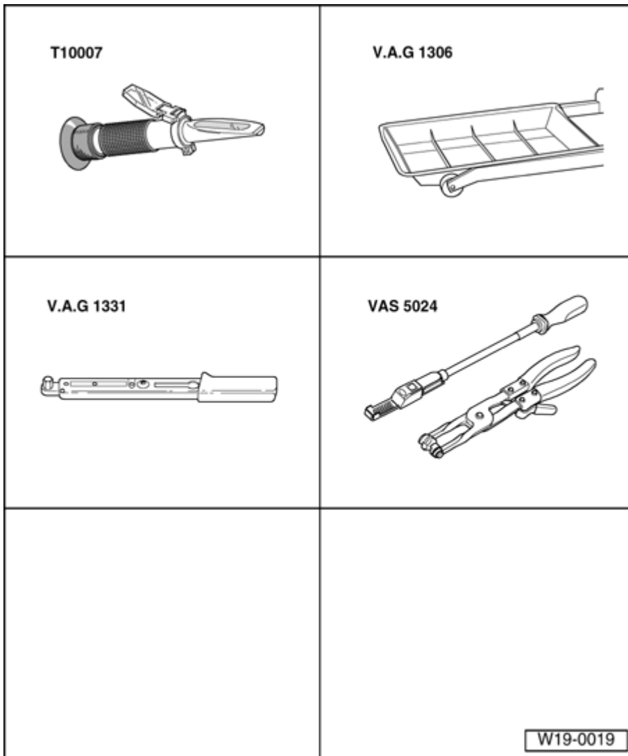
Fig. 151: Special Tools - Coolant Pump, Removing And Installing Courtesy of VOLKSWAGEN UNITED STATES, INC.
