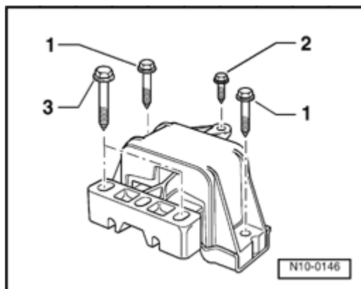
Fig. 17: Identifying Transmission Mounting Bracket & Bolts Courtesy of VOLKSWAGEN UNITED STATES, INC.
