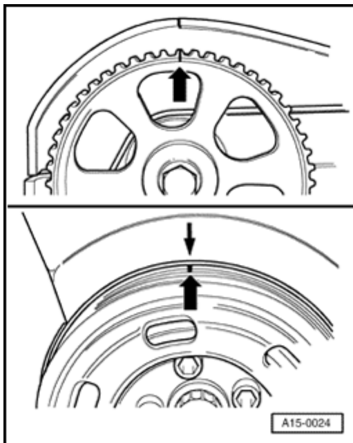
Fig. 69: Marking On Camshaft Gear Aligned With Marking On Cylinder Head Cover Courtesy of VOLKSWAGEN UNITED STATES, INC.
