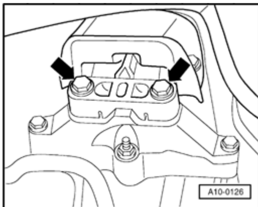
Fig. 10: Locating Engine Carrier Bolts (Transmission Side)
