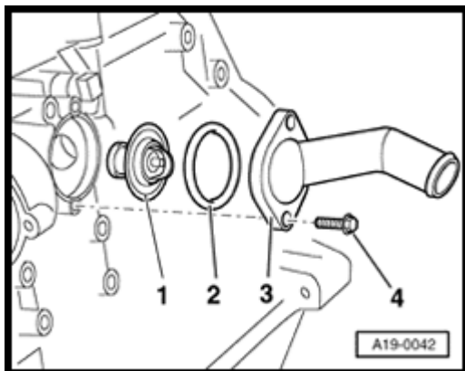
Fig. 152: Identifying Thermostat & Fasteners
