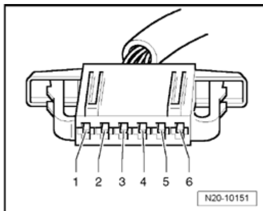
Fig. 190: Identifying Control Module Wiring Harness Pins Courtesy of VOLKSWAGEN UNITED STATES, INC.
