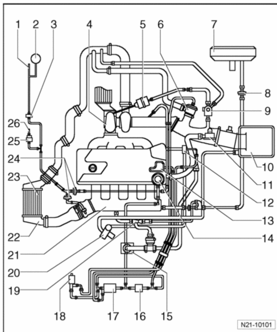
Fig. 217: Exhaust Turbocharging System (Engine Code AWP, AWW), Overview
