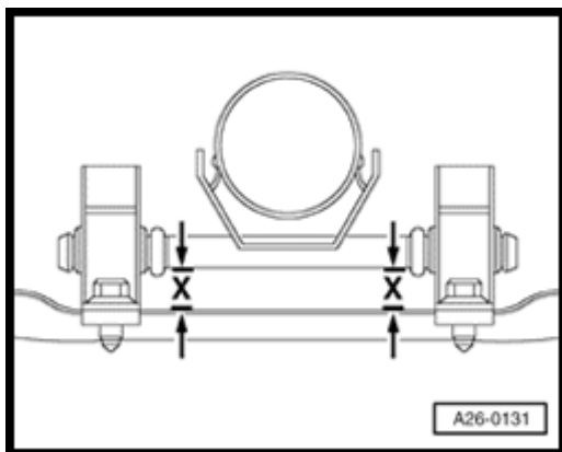
Fig. 238: Installing Muffler Free Of Tension
