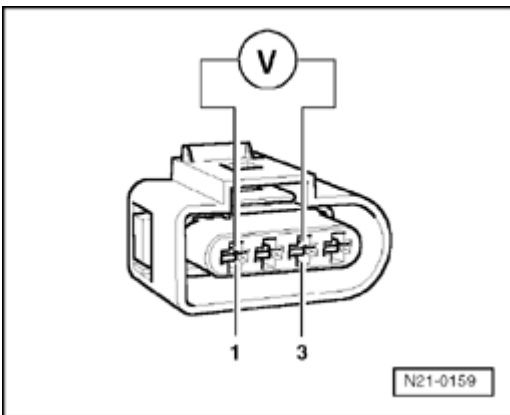
Fig. 222: Measuring Voltage Between Terminal 1(Ground) And 3 (Positive) On Connector Courtesy of VOLKSWAGEN UNITED STATES, INC.
