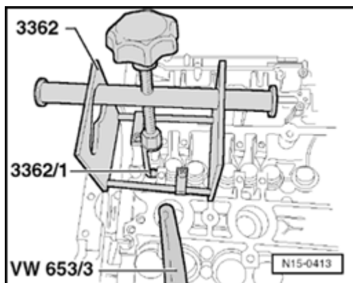
Fig. 122: Identifying Pressure Hose VW 653/3 And Thrust Piece 3362/1 In Valve Spring Compressor 3362
