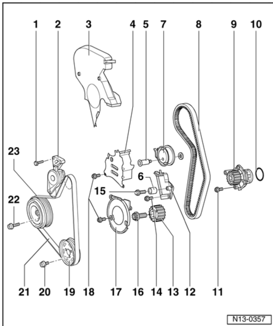
Fig. 21: Engine Assembly Overview I
