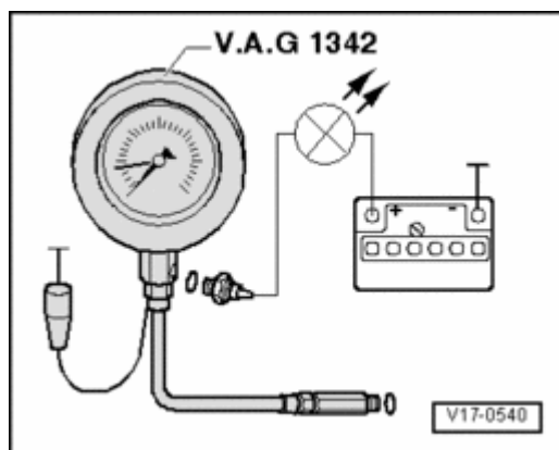
Fig. 134: Identifying V.A.G 1342 Oil Pressure Tester Courtesy of VOLKSWAGEN UNITED STATES, INC.
