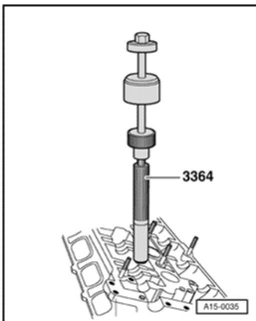
Fig. 123: Removing Valve Stem Seals Using Valve Stem Removal Tool 3364 Courtesy of VOLKSWAGEN UNITED STATES, INC.
