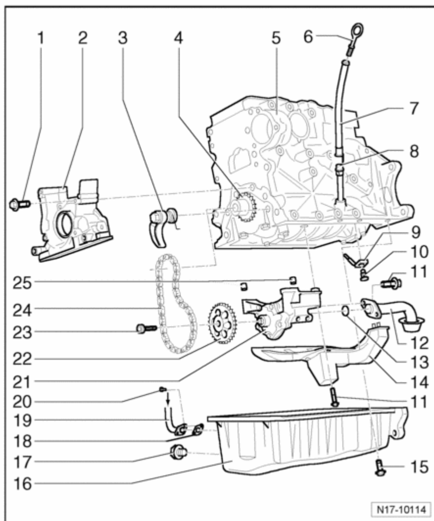
Fig. 125: Lubrication System Components, Assembly Overview - Part I Courtesy of VOLKSWAGEN UNITED STATES, INC.
