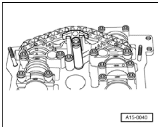
Fig. 113: Identifying Bearing Caps
