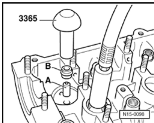
Fig. 124: Identifying Plastic Sleeve, Valve Stem Oil Seal And Valve Stem Seal Driver 3365 Courtesy of VOLKSWAGEN UNITED STATES, INC.
