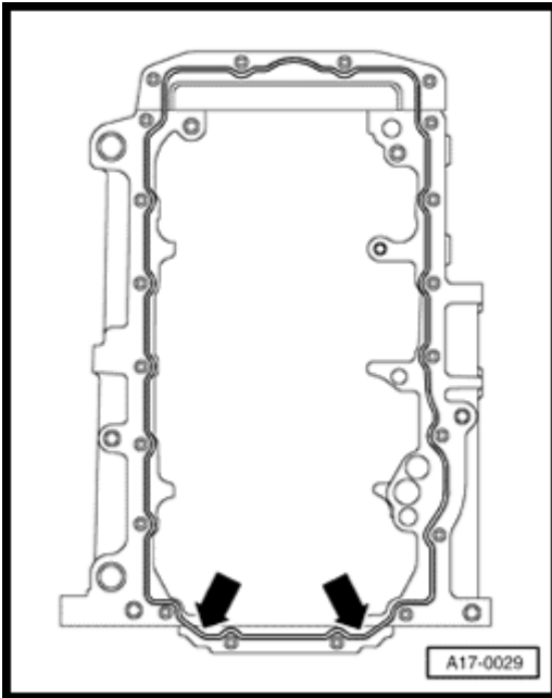
Fig. 132: Identifying Clean Sealing Surfaces Sealant Application Areas
