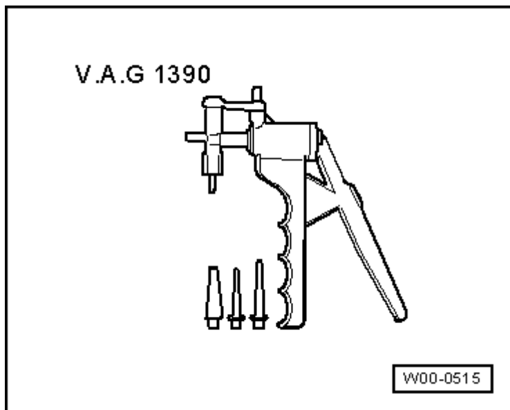
Fig. 229: Hand Vacuum Pump V.A.G 1390 Courtesy of VOLKSWAGEN UNITED STATES, INC.
