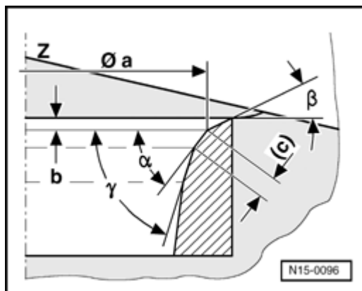
Fig. 88: Intake Valve Seat Measurements
