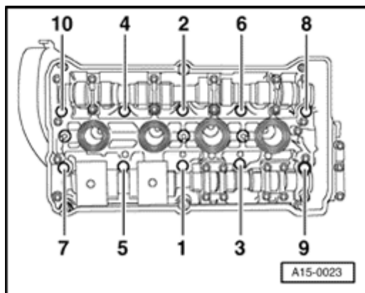
Fig. 77: Cylinder Head Bolt Position Numbers
