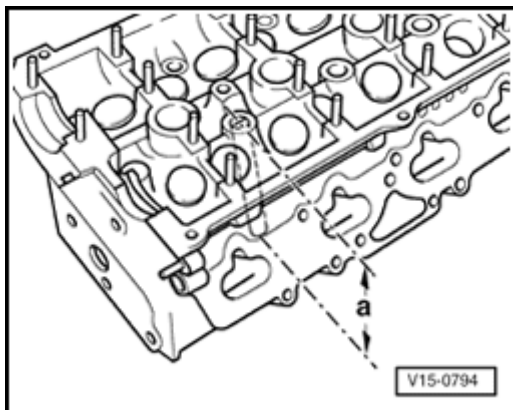
Fig. 82: Refacing Cylinder Head Sealing Surface Measurement Courtesy of VOLKSWAGEN UNITED STATES, INC.
