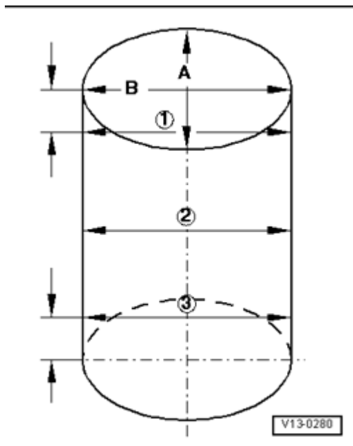
Fig. 52: Checking Cylinder Bores
