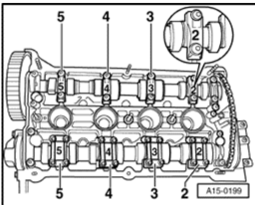
Fig. 109: Identifying Bearing Cap Positions Courtesy of VOLKSWAGEN UNITED STATES, INC.
