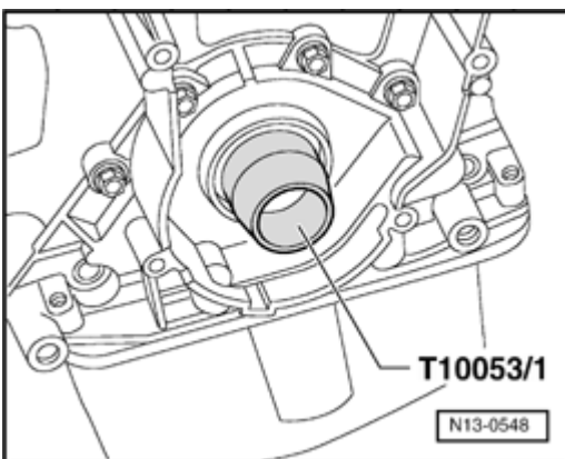
Fig. 33: Identifying Guide Sleeve T10053/1 Mounted Onto Crankshaft Journal
