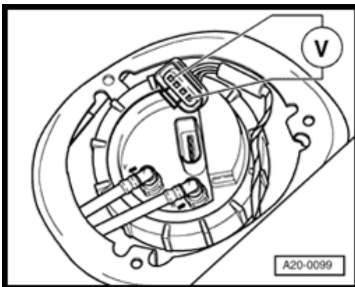
Fig. 176: Connecting Voltage Tester V.A.G 1527B Using Adapter Cables From Connector Test Kit V.A.G 1594C To Outer Terminals Of Connector Courtesy of VOLKSWAGEN UNITED STATES, INC.
