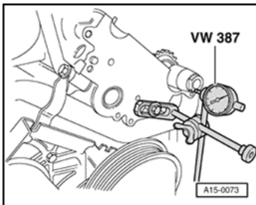
Fig. 83: Camshaft, Checking Axial Play Courtesy of VOLKSWAGEN UNITED STATES, INC.
