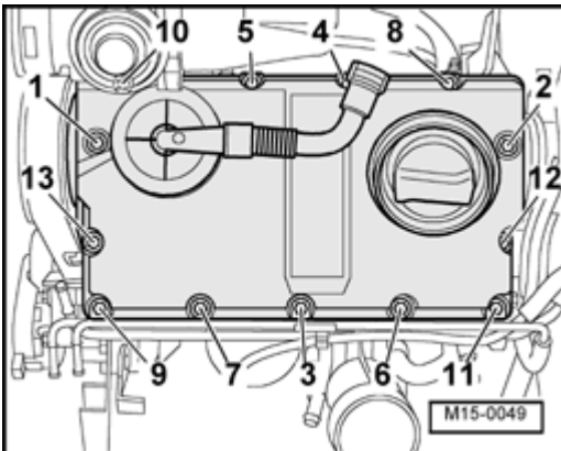
Fig. 60: Identifying Cylinder Head Cover Tightening Sequence Courtesy of VOLKSWAGEN UNITED STATES, INC.
