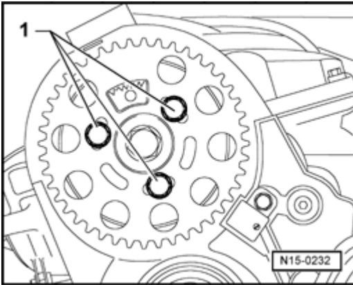
Fig. 98: Identifying Camshaft Pulley Securing Bolts Courtesy of VOLKSWAGEN UNITED STATES, INC.
