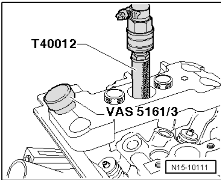
Fig. 4: Locating Pendulum Support Bolts
