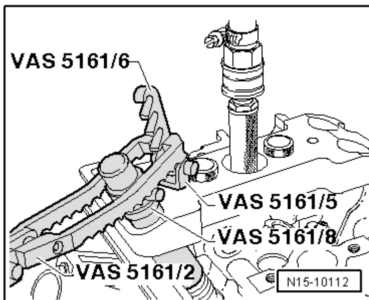
Fig. 11: Identifying Engine Mounting Bracket & Bolts
