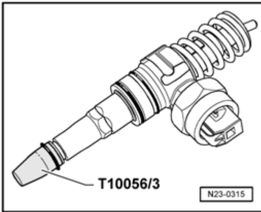
Fig. 179: Identifying Assembly Sleeve T10056/3
