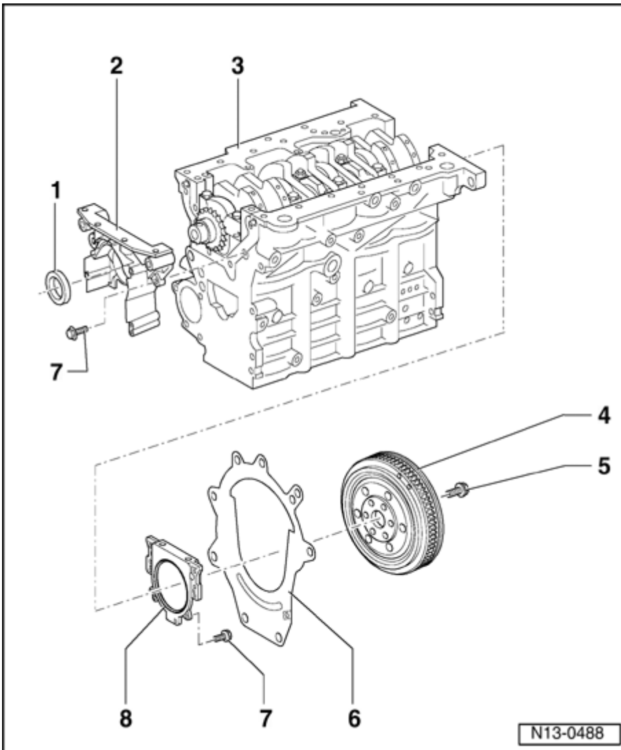
Fig. 26: Identifying Crankshaft Oil Seal
