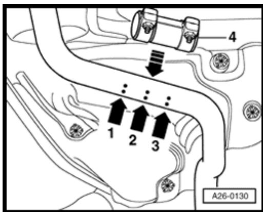
Fig. 196: Separating Point On Exhaust Pipe
