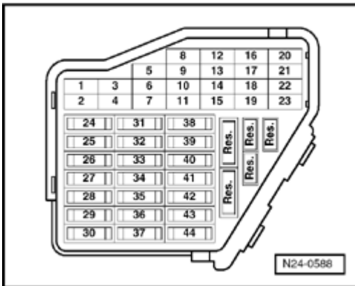
Fig. 156: Identifying Main Fuse Panel
