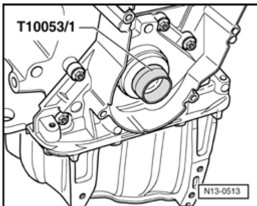
Fig. 30: Identifying Guide Sleeve T10053/1
