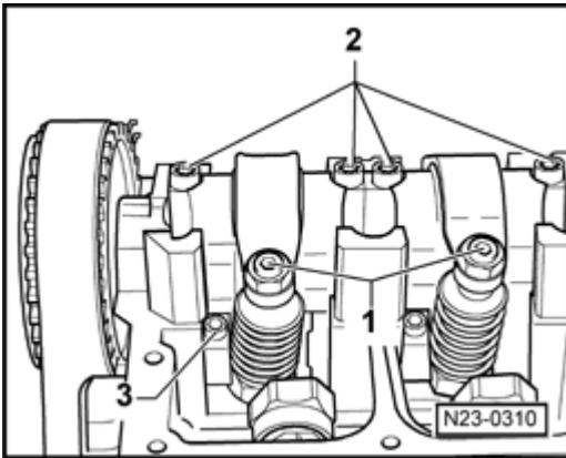
Fig. 181: Identifying Lock Nuts And Securing Bolts Courtesy of VOLKSWAGEN UNITED STATES, INC.
