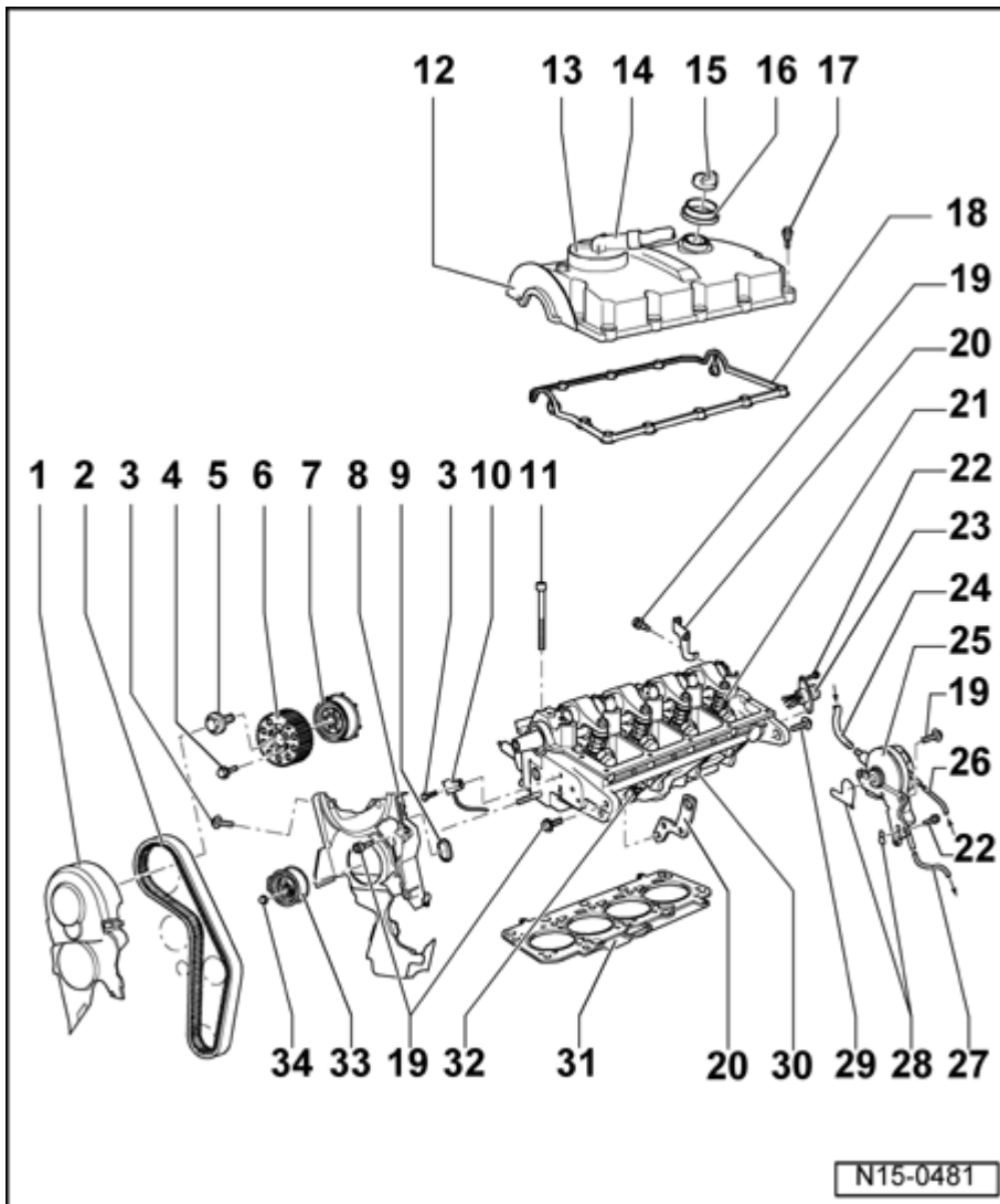
Fig. 55: Exploded View - Cylinder Head
