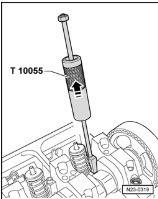
Fig. 182: Identifying Seat Puller T10055 Courtesy of VOLKSWAGEN UNITED STATES, INC.
