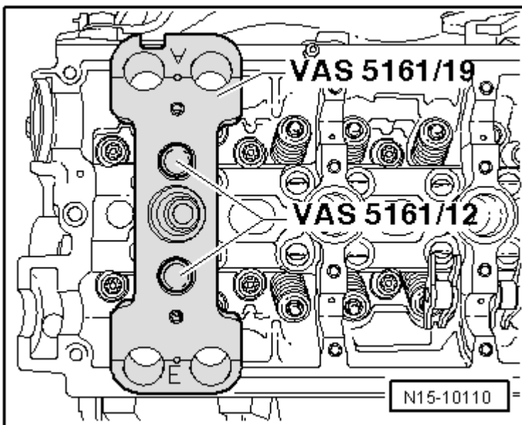
Fig. 3: Identifying Special Tools - Engine, Removing And Installing (2 Of 2) Courtesy of VOLKSWAGEN UNITED STATES, INC.
