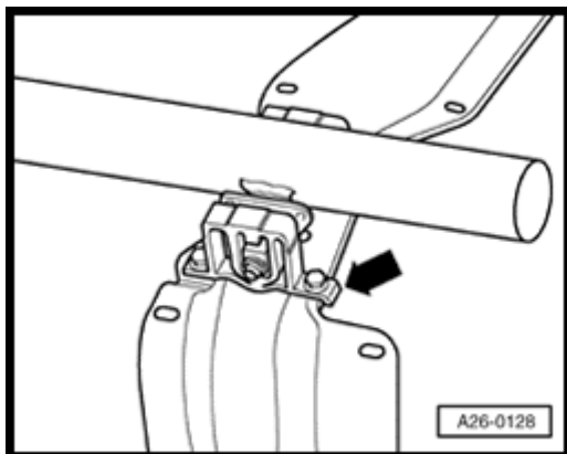
Fig. 195: Installation Position Of Mounting
