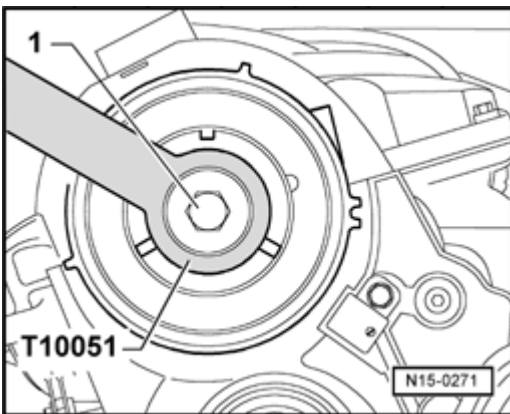
Fig. 99: Identifying Counterhold T10051 Courtesy of VOLKSWAGEN UNITED STATES, INC.
