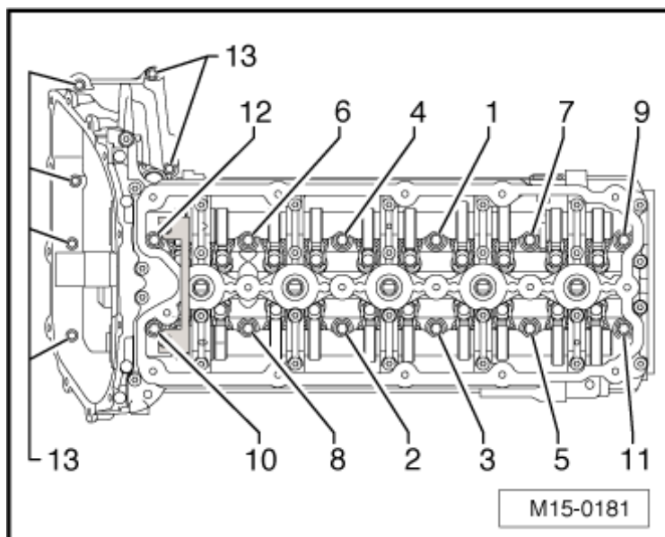
Fig. 39: Identifying Cylinder Head Bolts Tightening Sequence
