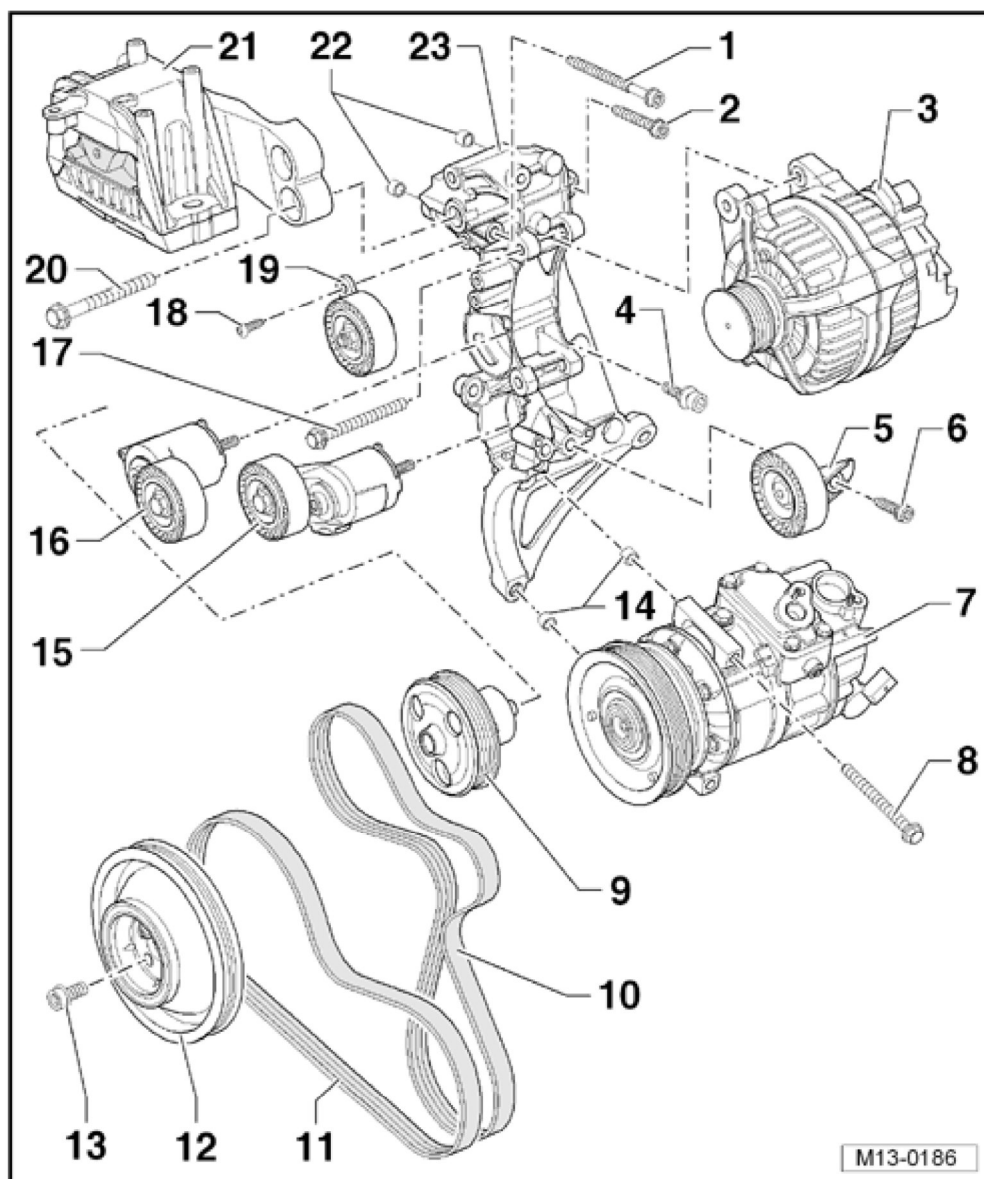
Fig. 5: Identifying Accessory Drive And Ribbed Belt - Overview
