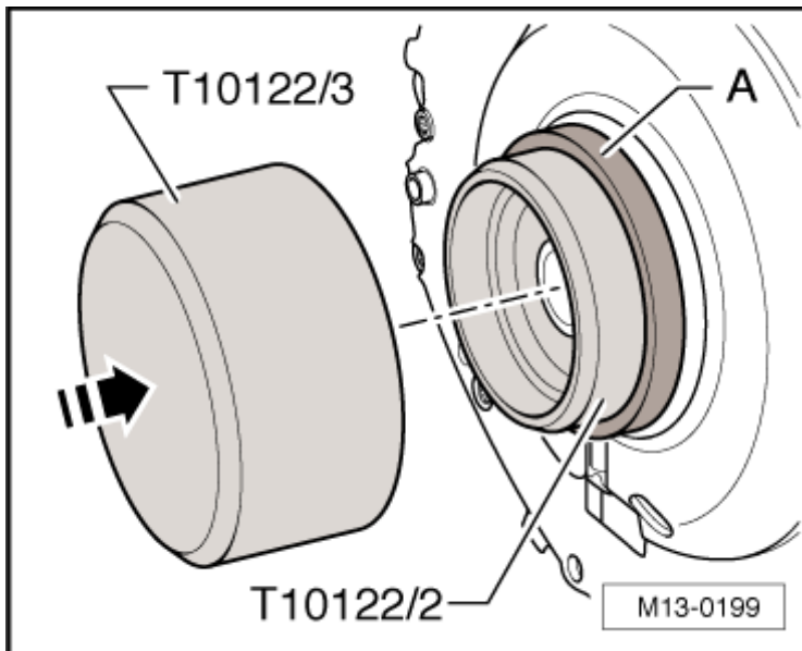
Fig. 55: Identifying Installation Of Pull Sleeve T10122/2 With Sealing Ring Onto Crankshaft Courtesy of VOLKSWAGEN GROUP OF AMERICA, INC.
