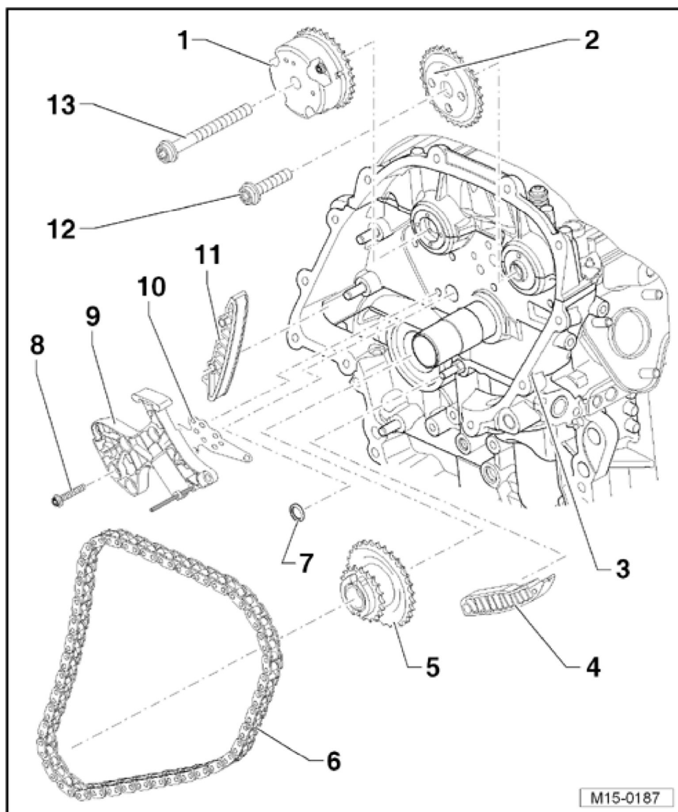
Fig. 14: Identifying Chain Drive / Timing Chain Assembly Overview Courtesy of VOLKSWAGEN GROUP OF AMERICA, INC.
