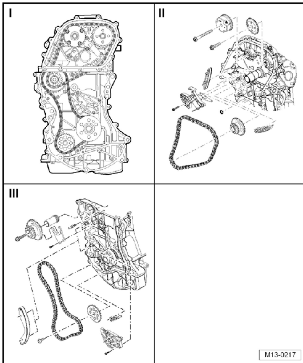
Fig. 12: Identifying Chain Drive, Assembly Overview - Part I, II, III Courtesy of VOLKSWAGEN GROUP OF AMERICA, INC.
