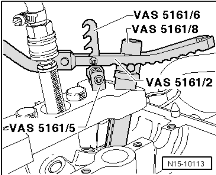
Fig. 49: Identifying Pressure Forks VAS 5161/2 Engaged
