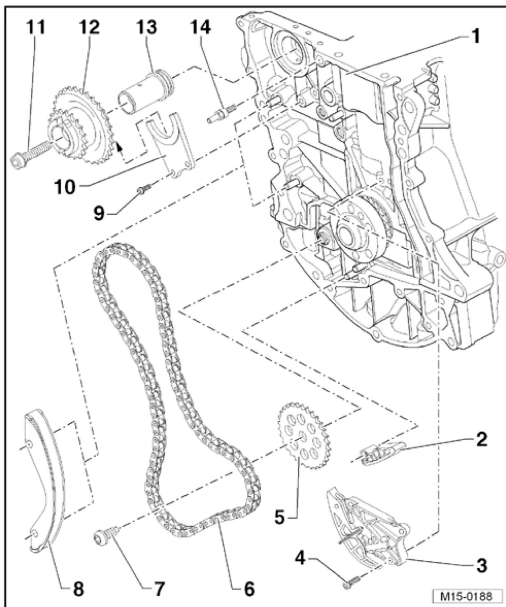
Fig. 15: Identifying Timing Chain & Oil Pump Assembly Overview Courtesy of VOLKSWAGEN GROUP OF AMERICA, INC.
