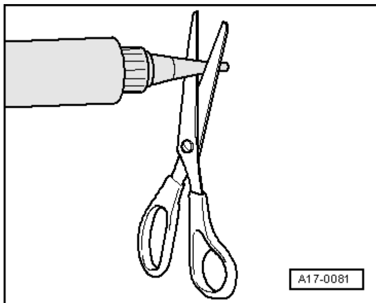
Fig. 44: Identifying Scissors To Cut Tube Nozzle At Front Marking (Nozzle Diameter Approx. 2 Mm) Courtesy of VOLKSWAGEN GROUP OF AMERICA, INC.
