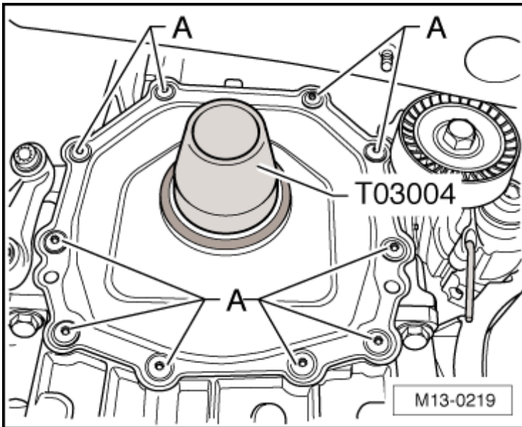
Fig. 46: Identifying Sealing Flange Inserted Using Assembly Sleeve T03004 On Crankshaft Journals And Pressed Uniformly On Cylinder Block
