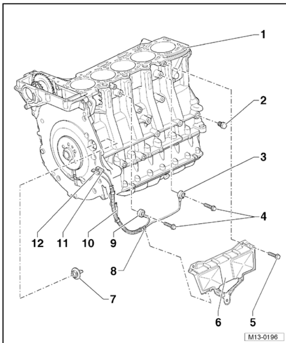
Fig. 9: Identifying Rear Engine Overview
