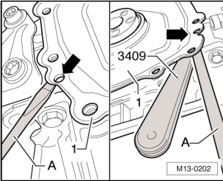
Fig. 41: Identifying Screwdriver And Trim Removal Wedge 3409 To Press Off Sealing Flange Courtesy of VOLKSWAGEN GROUP OF AMERICA, INC.
