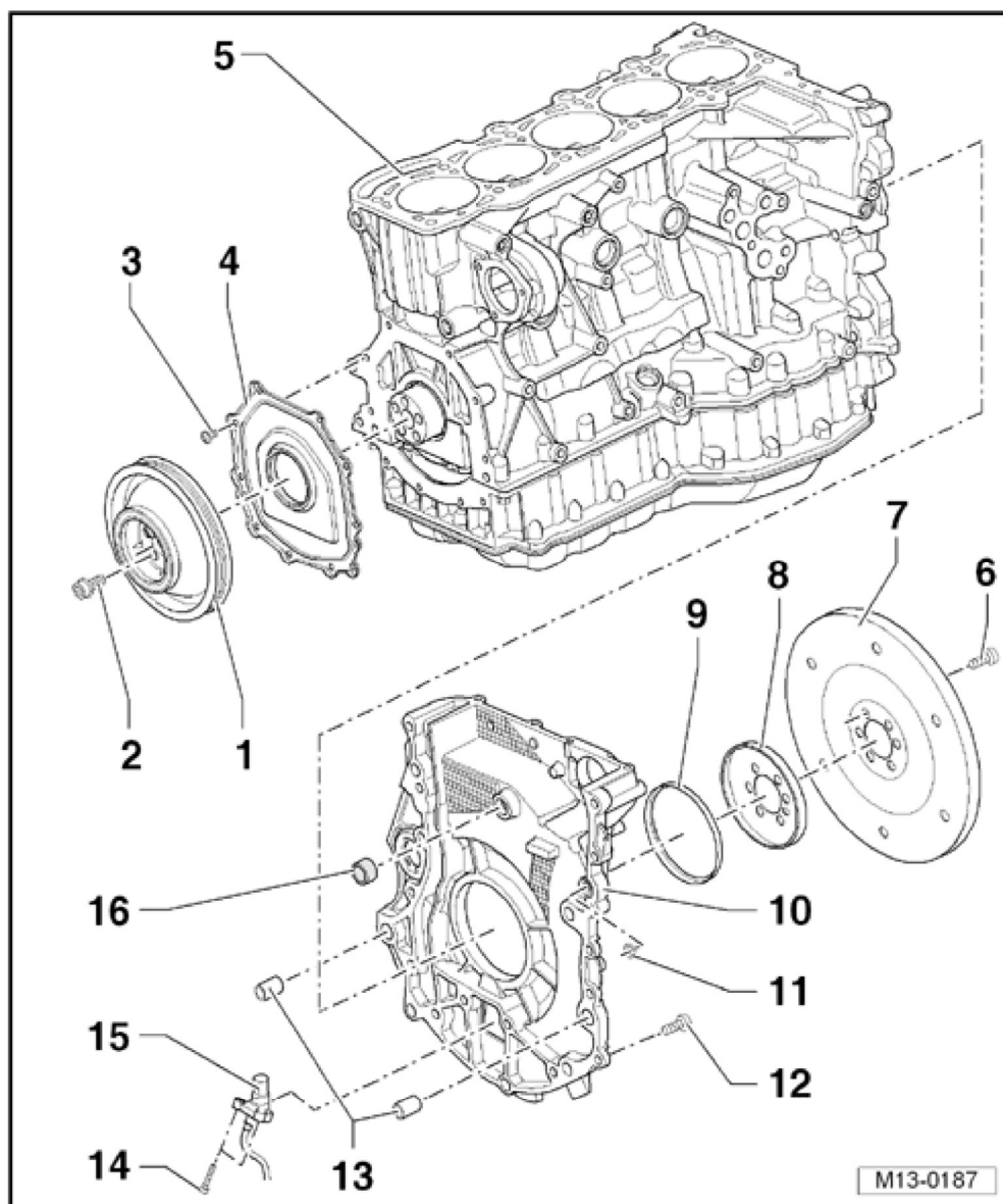
Fig. 16: Identifying Sealing Flange And Drive Plate/Flywheel Overview Courtesy of VOLKSWAGEN GROUP OF AMERICA, INC.
