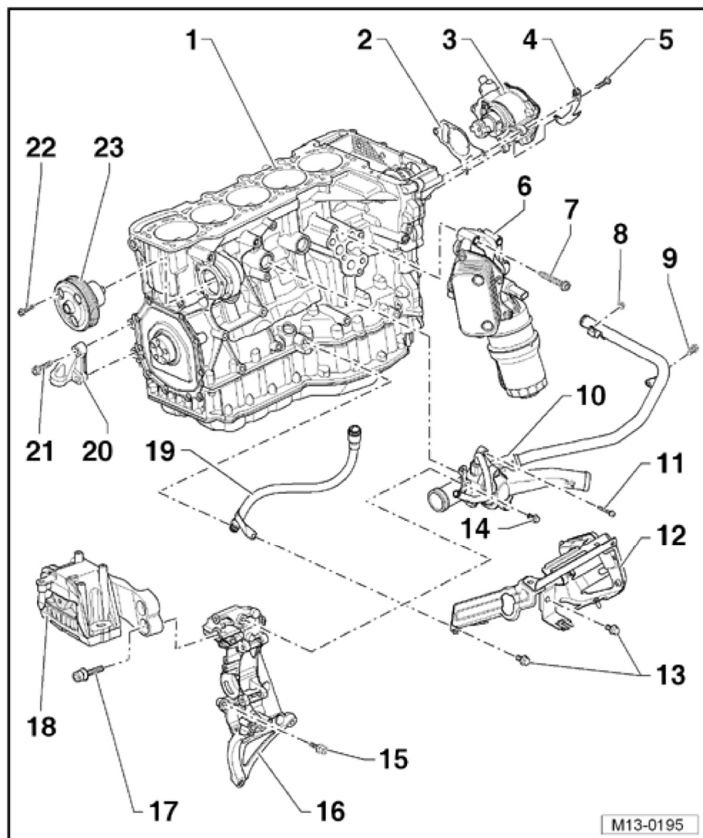
Fig. 11: Identifying Engine Front/Side Overview
