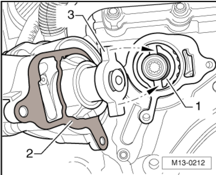
Fig. 39: Identifying New Gasket On Placed On Vacuum Pump Courtesy of VOLKSWAGEN GROUP OF AMERICA, INC.
