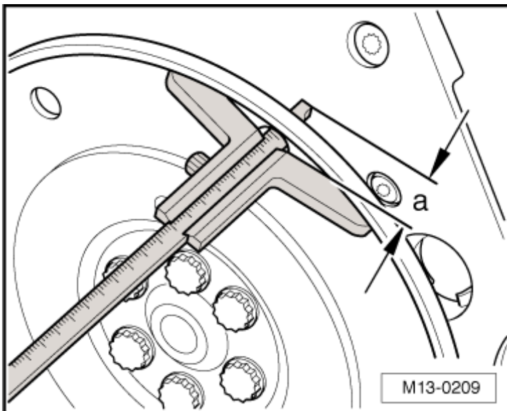
Fig. 57: Identifying Check Of Dimension Courtesy of VOLKSWAGEN GROUP OF AMERICA, INC.
