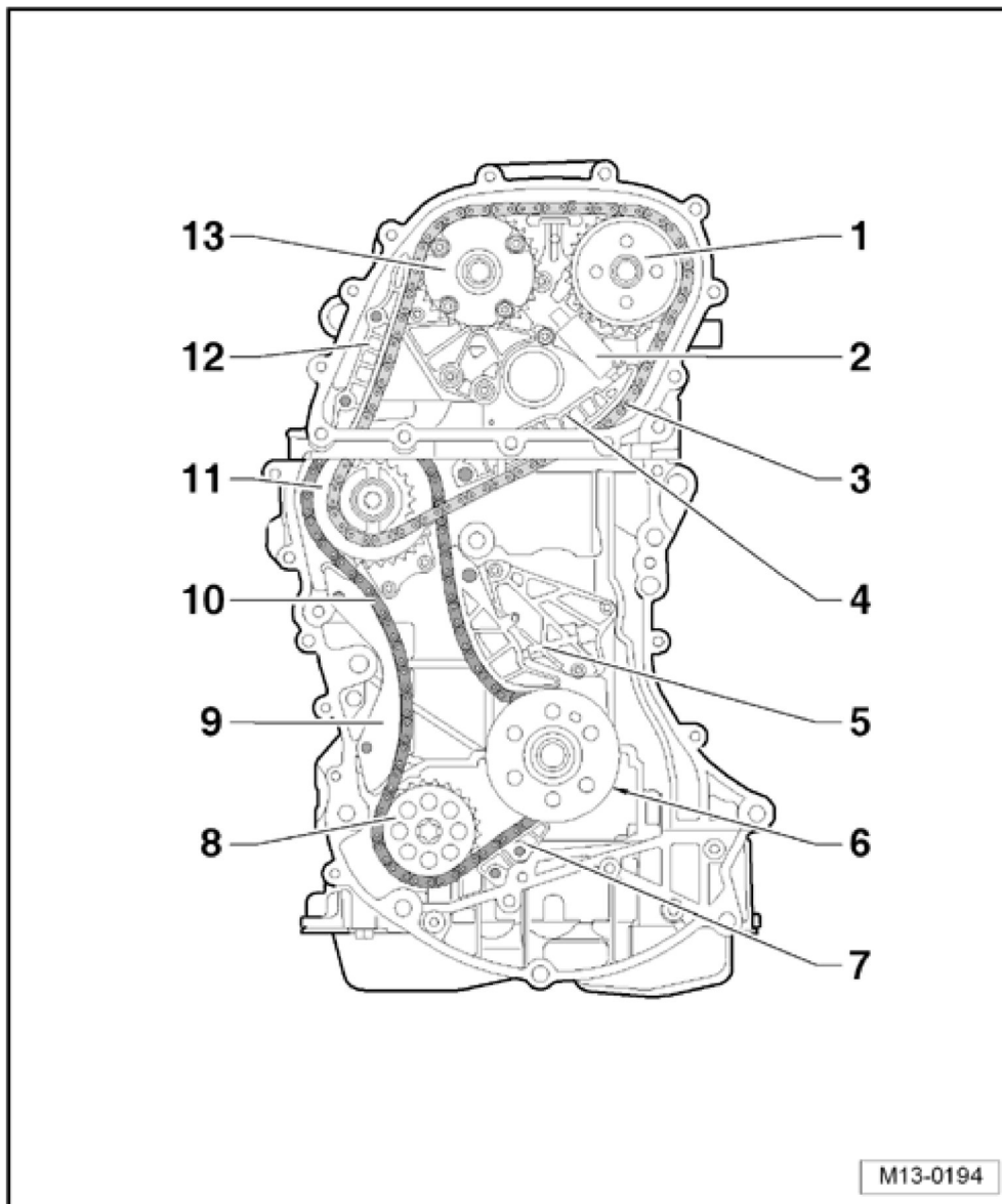
Fig. 13: Identifying Chain Drive, Assembly Overview Courtesy of VOLKSWAGEN GROUP OF AMERICA, INC.
