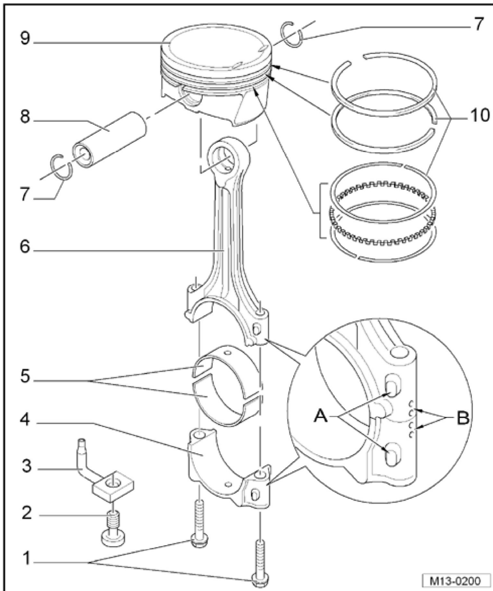
Fig. 27: Identifying Piston And Connecting Rod Assembly Overview Courtesy of VOLKSWAGEN GROUP OF AMERICA, INC.
