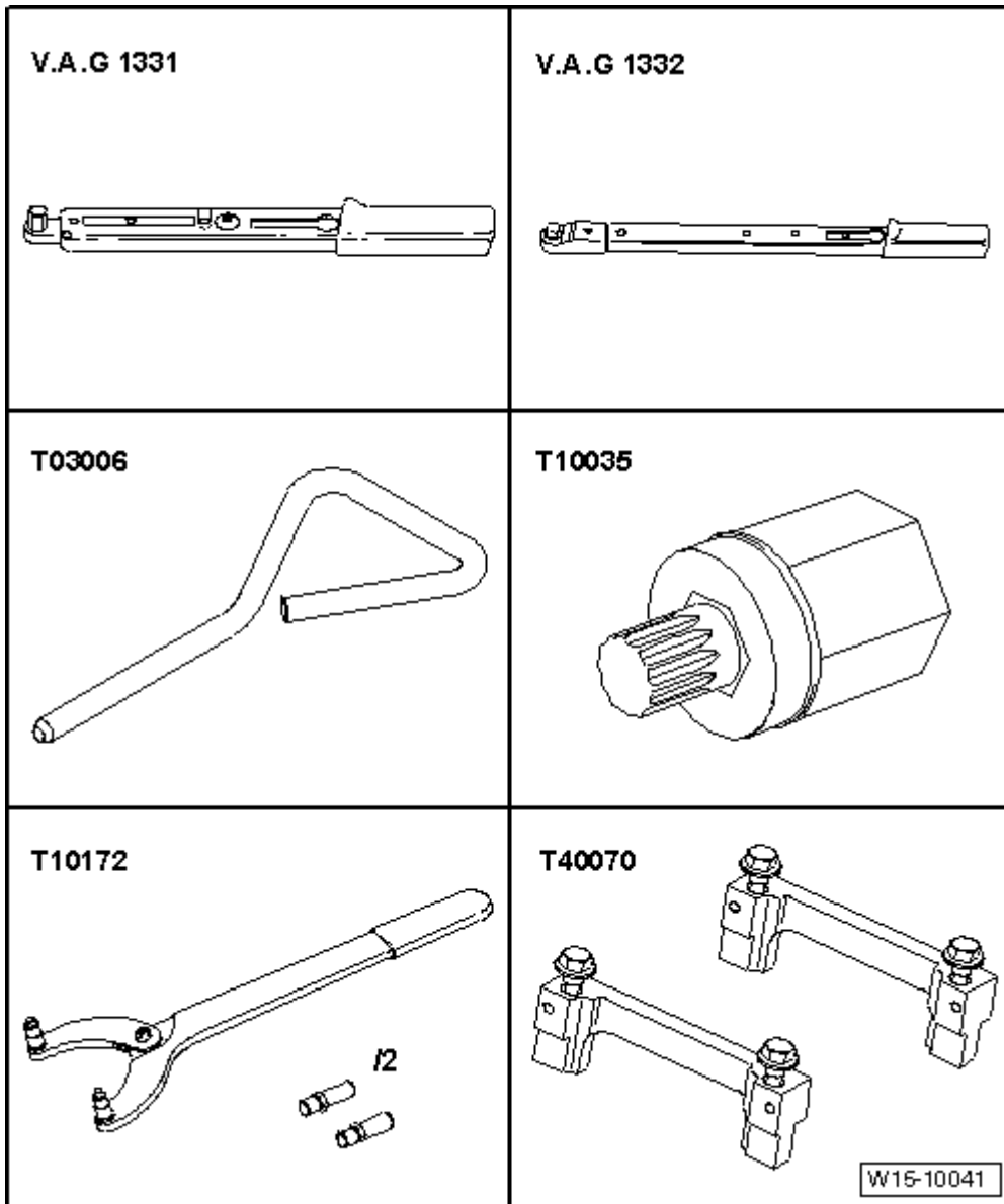
Fig. 61: Identifying Special Tools -- Valve Timing, Adjusting
