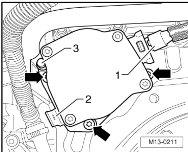
Fig. 38: Locating 3 Bolts And Vacuum Pump Courtesy of VOLKSWAGEN GROUP OF AMERICA, INC.
