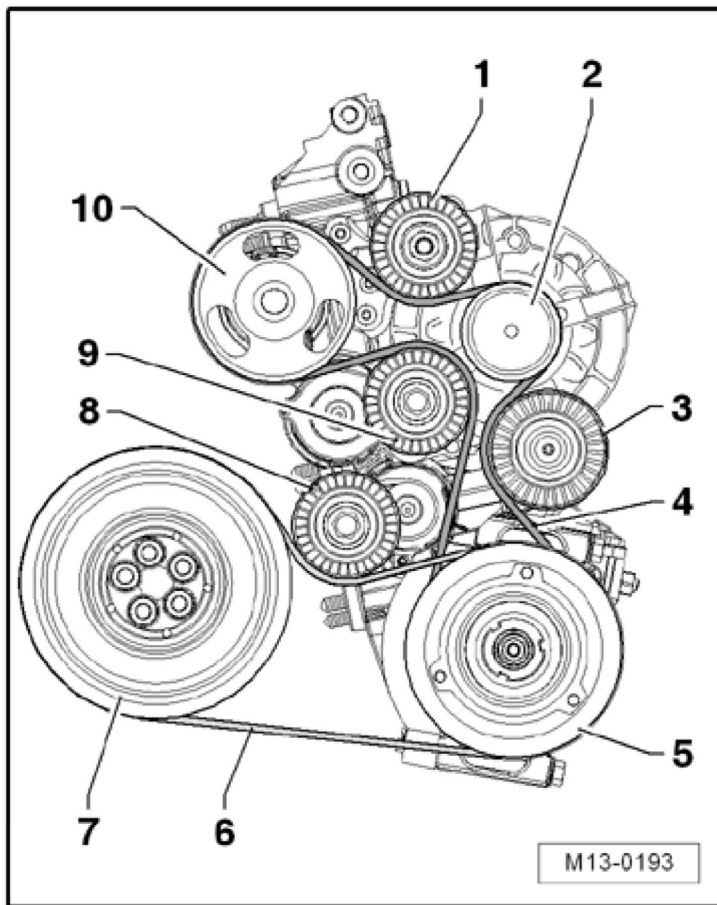
Fig. 6: Identifying Ribbed Belt Routing 2.5L 5-Cylinder Gasoline Engine Courtesy of VOLKSWAGEN GROUP OF AMERICA, INC.
