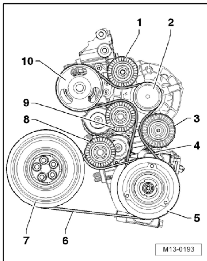
Fig. 35: Identifying Ribbed Belt Routing 2.5L 5-Cylinder Gasoline Engine Courtesy of VOLKSWAGEN GROUP OF AMERICA, INC.
