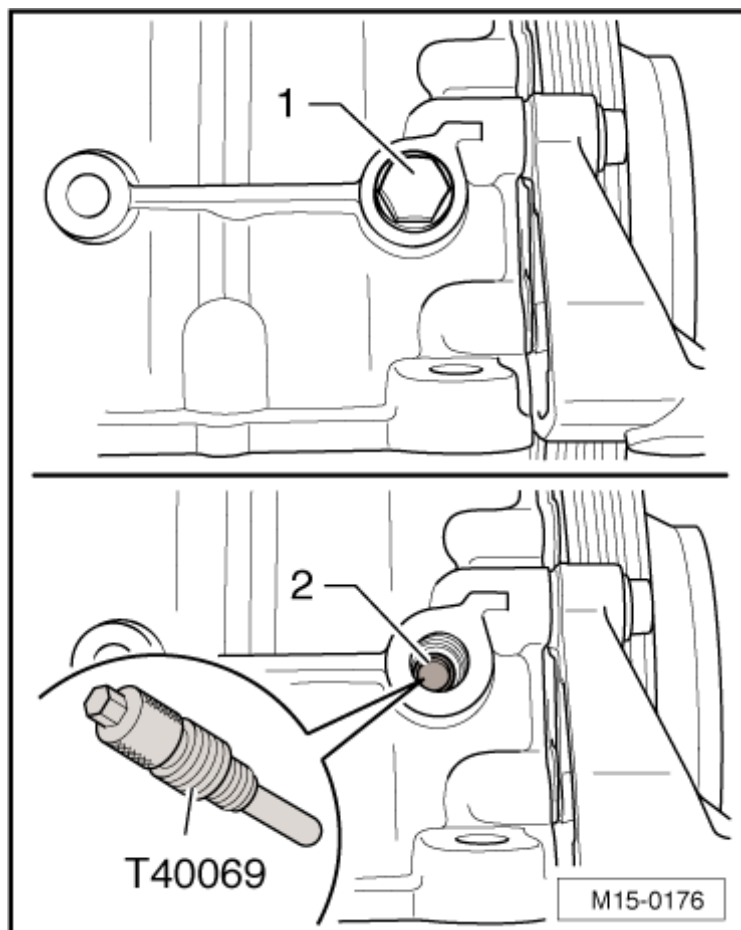
Fig. 23: Identifying Crankshaft Must Not Be Rotated Out Over TDC Marking Courtesy of VOLKSWAGEN GROUP OF AMERICA, INC.
