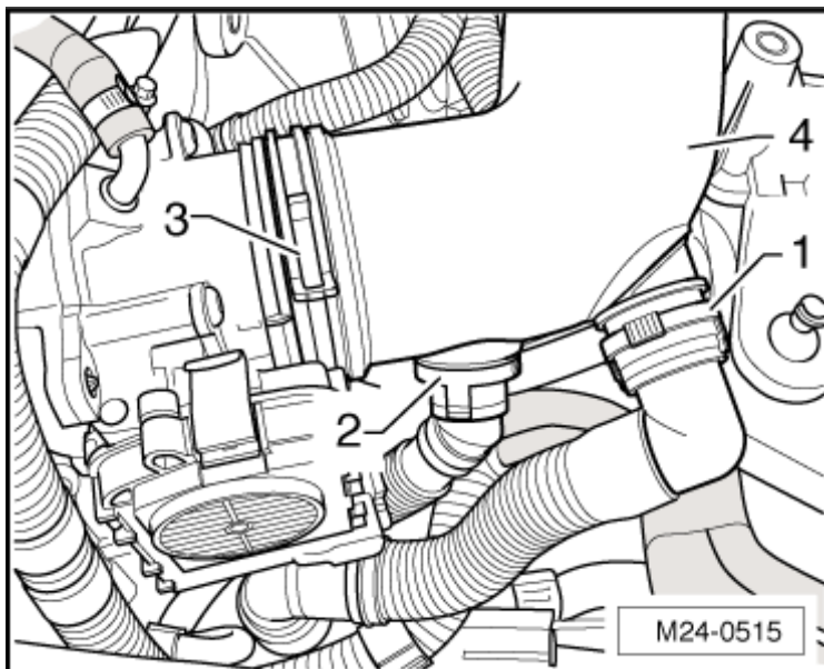
Fig. 37: Identifying Air Hoses And Are Fitted Securely Courtesy of VOLKSWAGEN GROUP OF AMERICA, INC.
