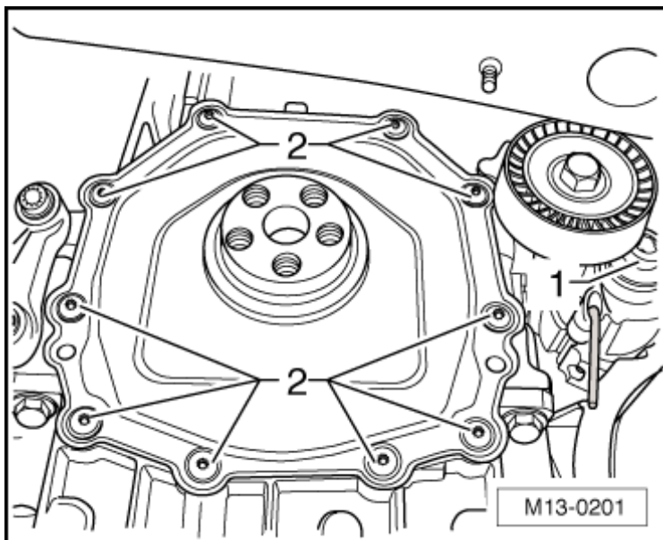
Fig. 40: Identifying Tensioning Element & Bolts
