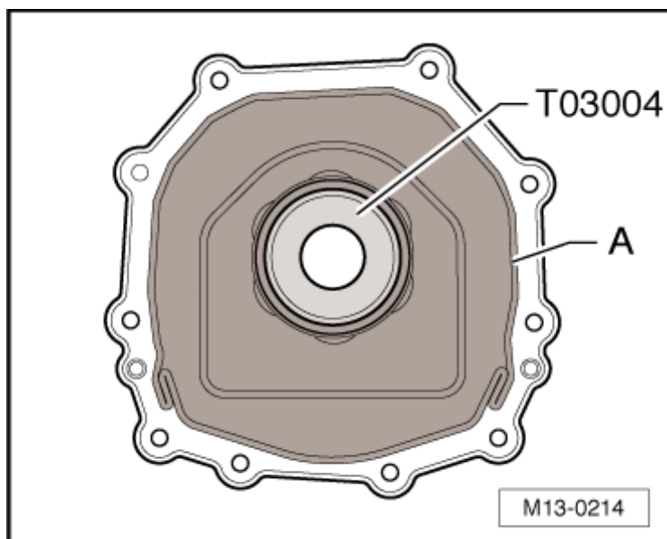
Fig. 45: Identifying Sealant Bead Applied Into Groove Of Sealing Flange
