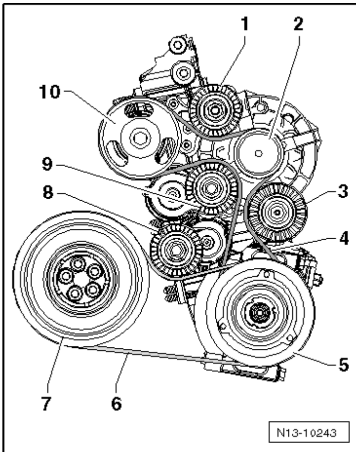
Fig. 8: Identifying Ribbed Belt Routing
