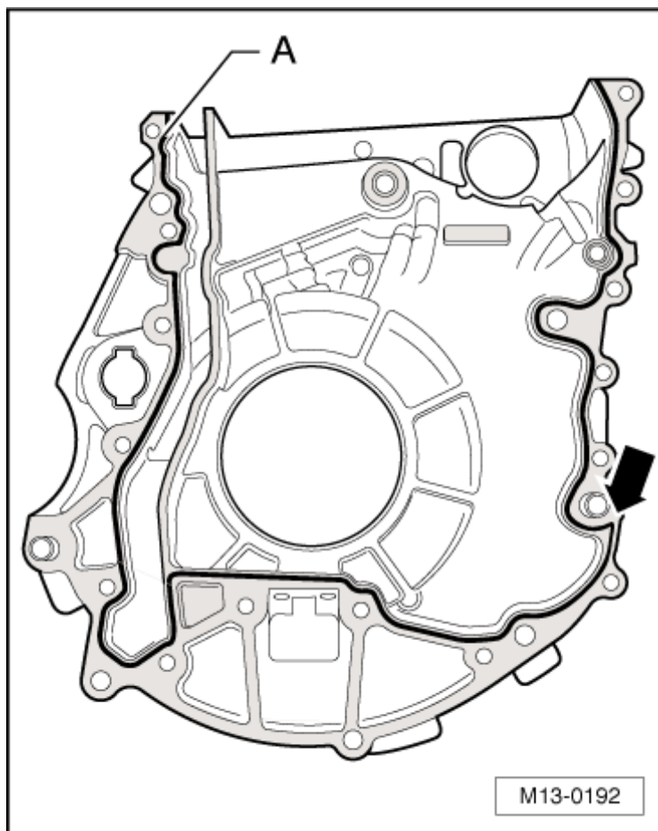
Fig. 51: Identifying Sealant Bead To Apply On Control Housing Cover Courtesy of VOLKSWAGEN GROUP OF AMERICA, INC.
