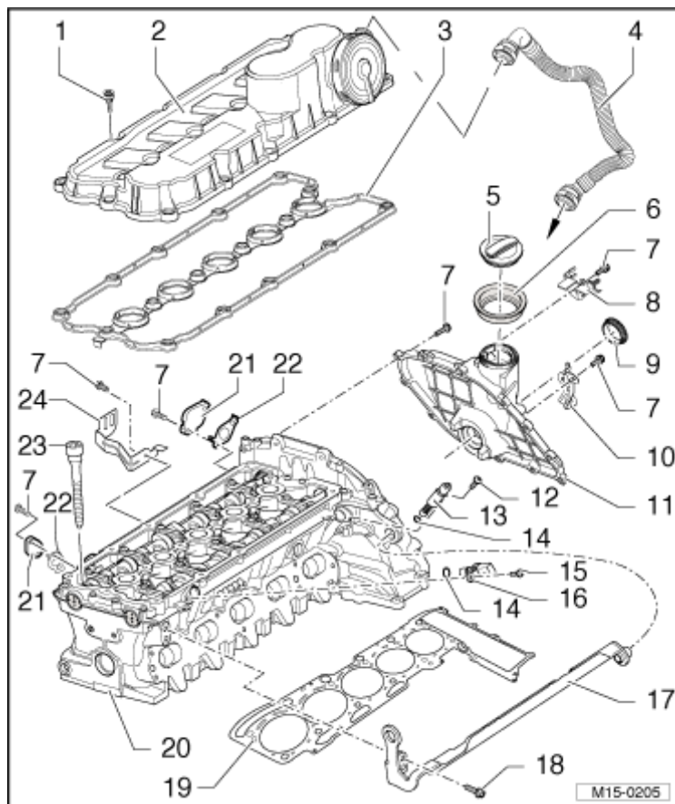
Fig. 1: Identifying Cylinder Head, Assembly Overview
