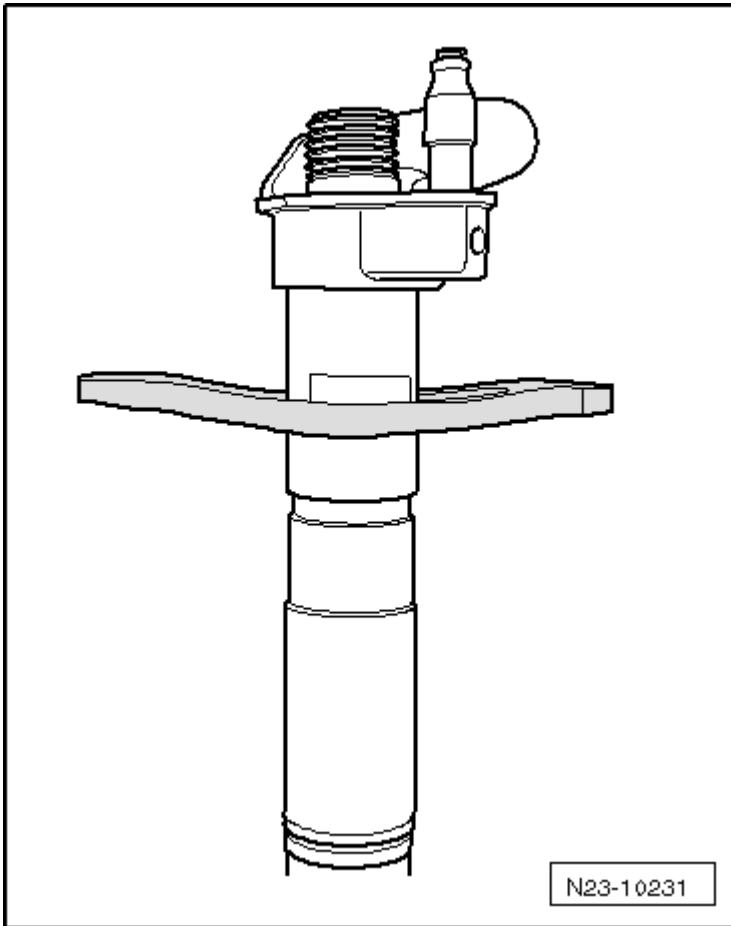
Fig. 2: Identifying Tensioning Plate Installed Position
