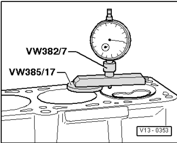
Fig. 4: Identifying Measurement Of Piston Projection
