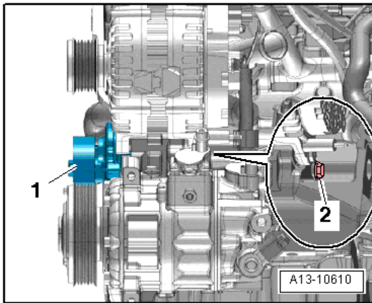
Fig. 82: Identifying Camshaft Clamping Tool T40095 Courtesy of VOLKSWAGEN GROUP OF AMERICA, INC.
