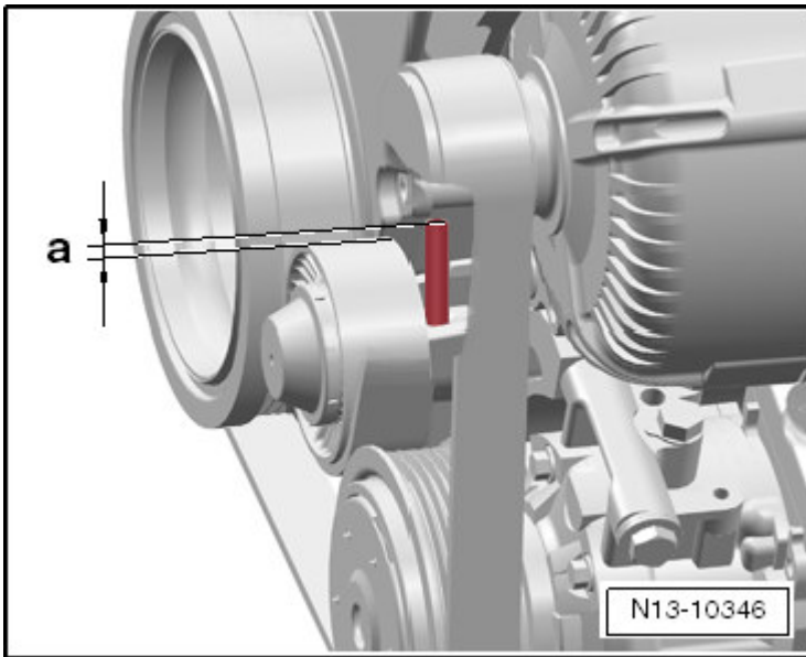
Fig. 86: Identifying Counterhold T10051 Courtesy of VOLKSWAGEN GROUP OF AMERICA, INC.
