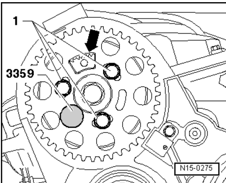
Fig. 87: Identifying Camshaft Pulley Bolts Courtesy of VOLKSWAGEN GROUP OF AMERICA, INC.
