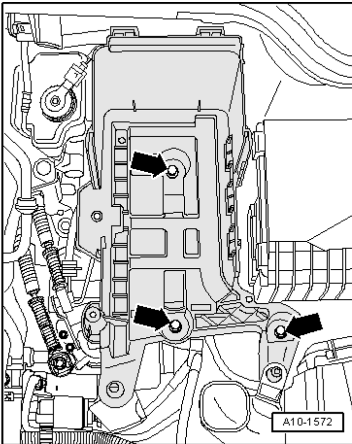
Fig. 55: Identifying Battery Holder Bolts
