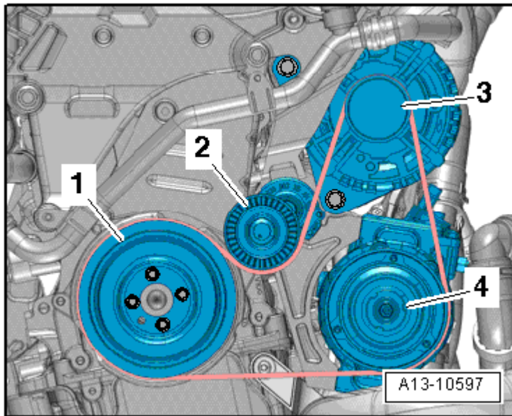
Fig. 84: Identifying Silicone Adhesive Sealant Pattern Courtesy of VOLKSWAGEN GROUP OF AMERICA, INC.
