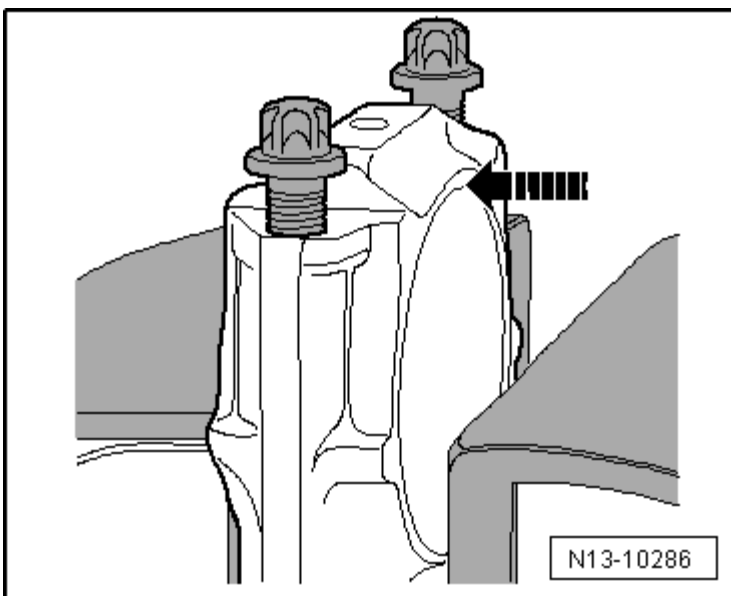
Fig. 57: Identifying Connector -1-, Clamp -2 And Coolant Hose -3-
