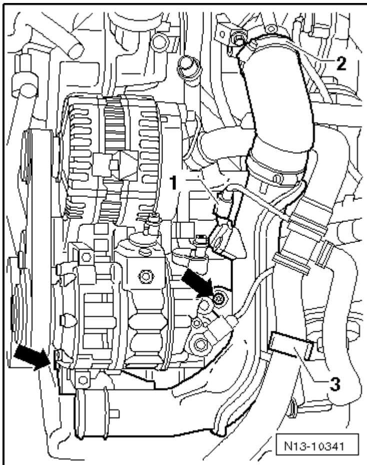
Fig. 24: Identifying Bolt To Remove
