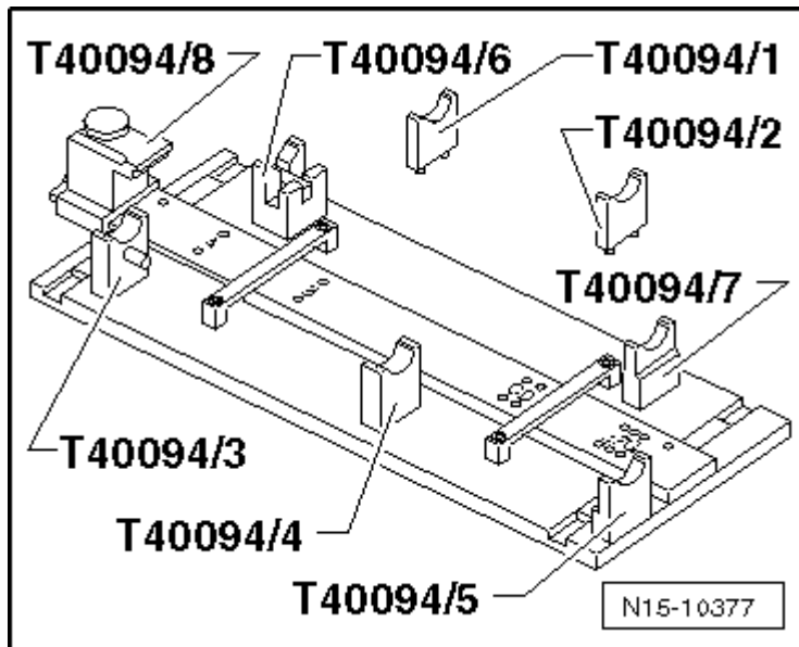
Fig. 73: Identifying Mounts T40094/1 To T40094/8
