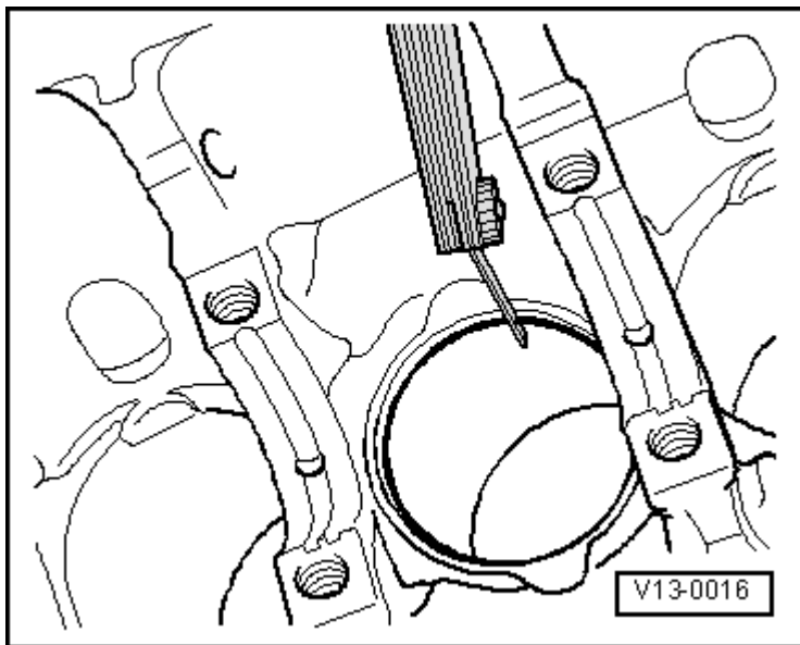
Fig. 11: Identifying Check Of Piston Ring Gap
