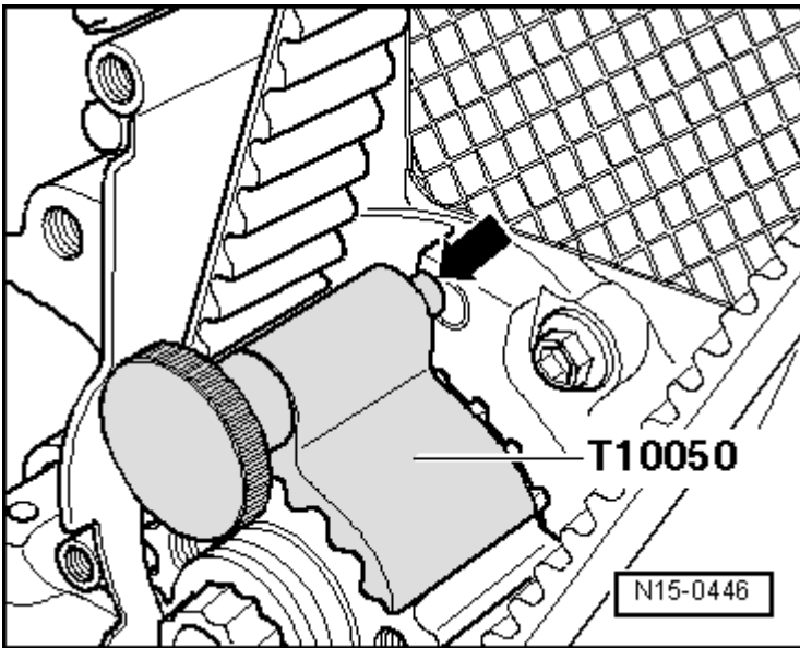
Fig. 44: Identifying Crankshaft Stop T10050
