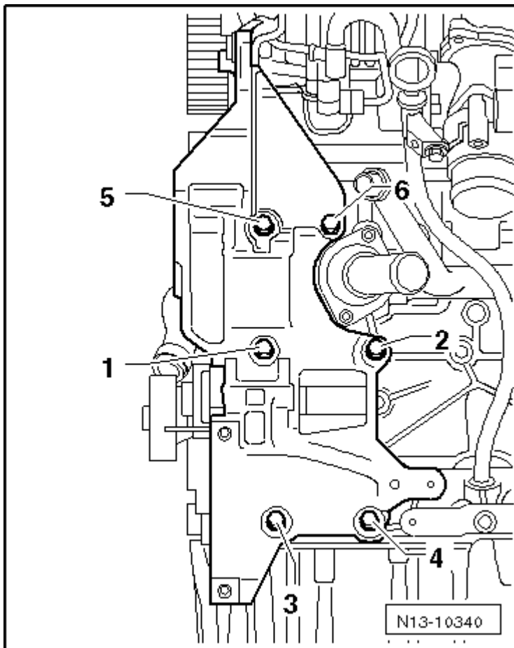
Fig. 33: Identifying Bolt Tightening Sequence
