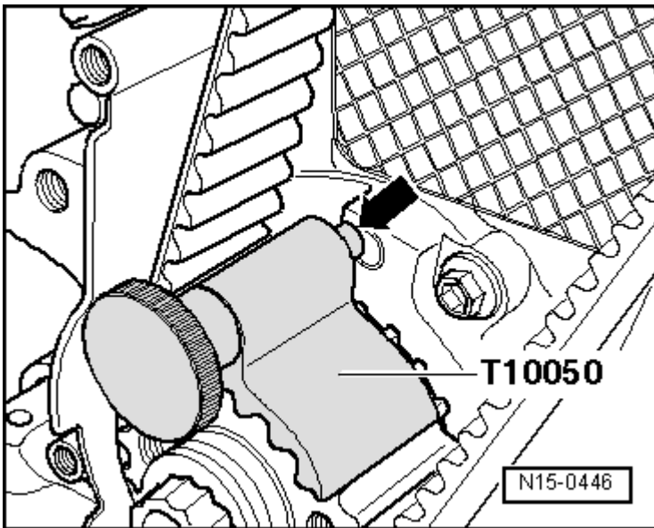
Fig. 46: Identifying Crankshaft Stop T10050
