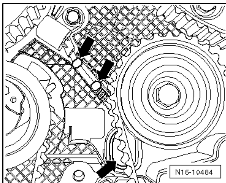
Fig. 20: Identifying Repair Opening -Arrows-
