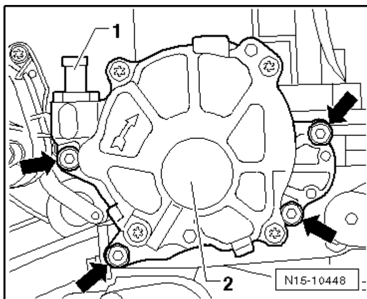
Fig. 68: Identifying Vacuum Pump Bolts
