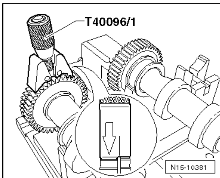
Fig. 77: Identifying Tensioning Tool T40096/1
