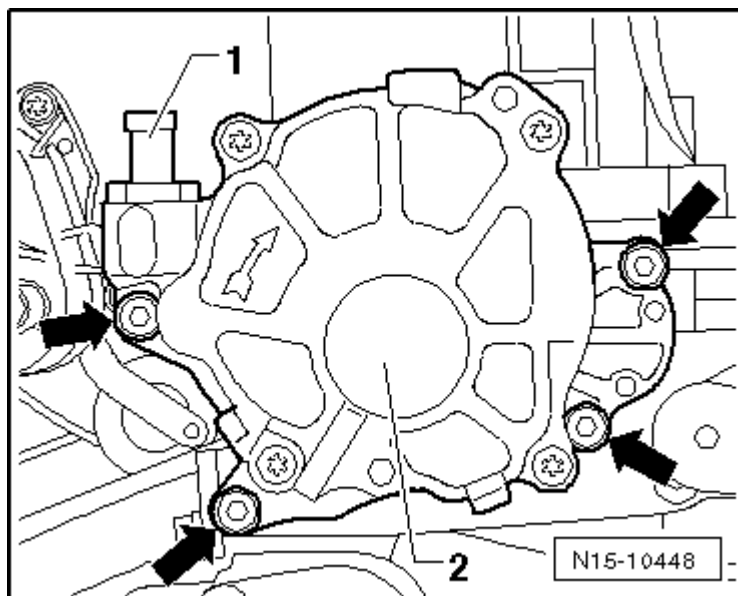
Fig. 67: Identifying Vacuum Pump Bolts
