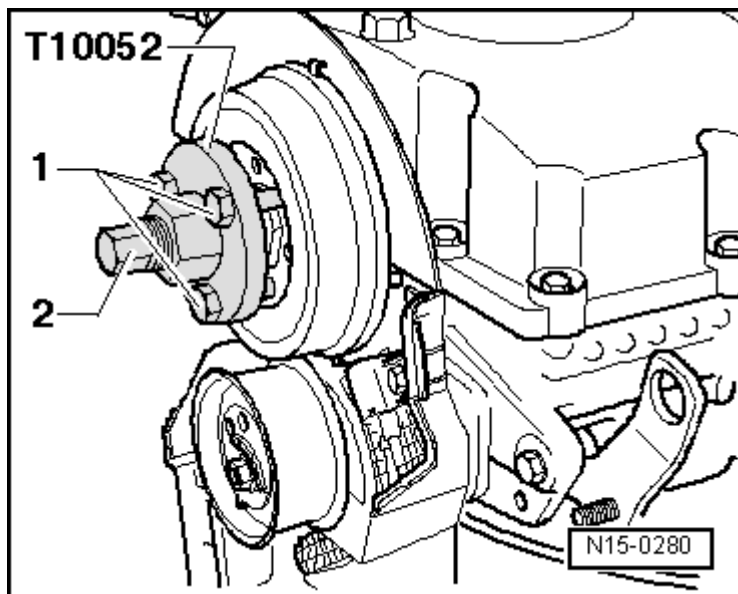
Fig. 71: Identifying Puller T10052
