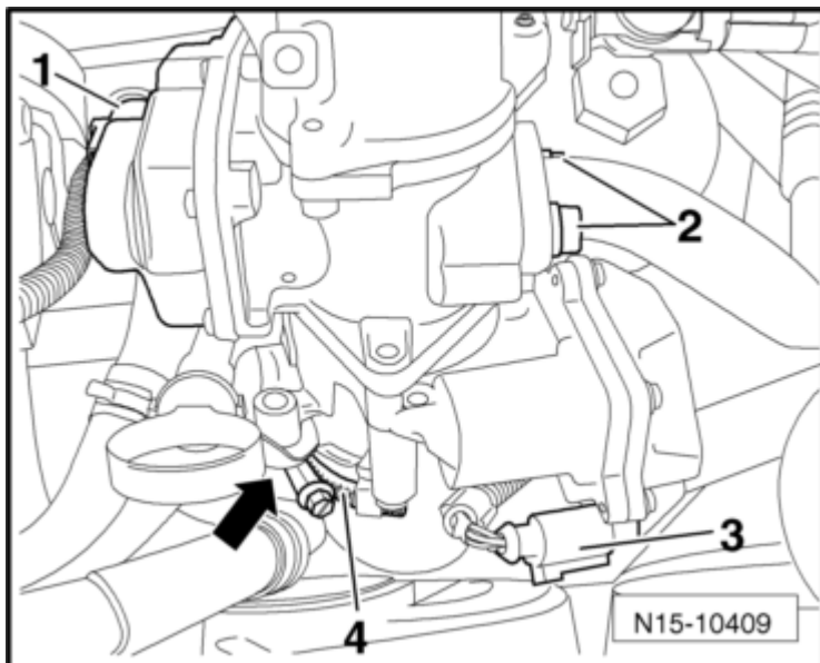
Fig. 49: Identifying Connectors
