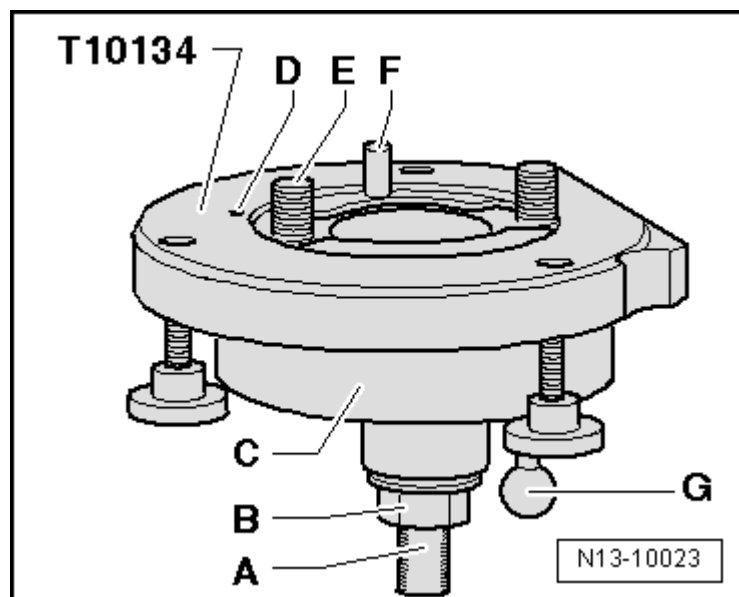
Fig. 45: Identifying Assembly Tool T10134
