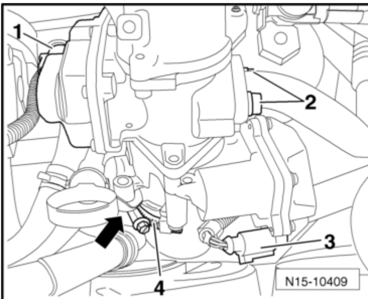
Fig. 48: Identifying Connectors
