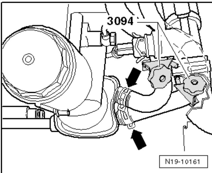
Fig. 75: Identifying Hose Clamps 3094
