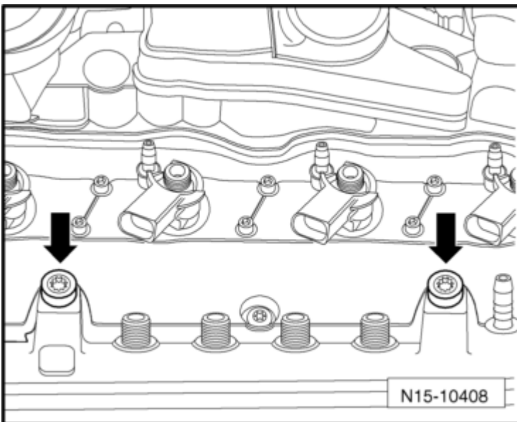
Fig. 28: Identifying Bolts -Arrows- And Fuel Rail
