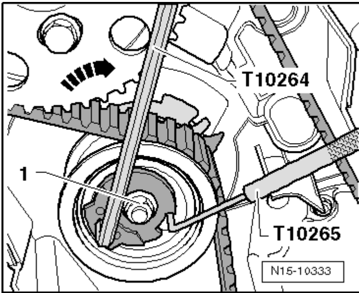
Fig. 37: Identifying Long Reach T10264 And Locking Tool T10265 Courtesy of VOLKSWAGEN GROUP OF AMERICA, INC.
