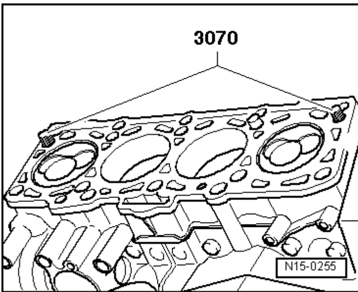
Fig. 64: Identifying Installed Guide Pins
