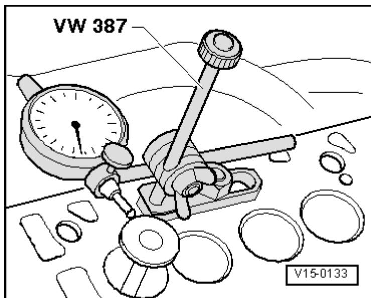
Fig. 32: Determining Valve Rock (Wear Limit)
