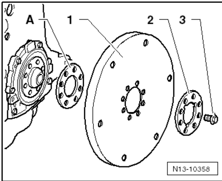
Fig. 56: Identifying Shim -A- And Bolts
