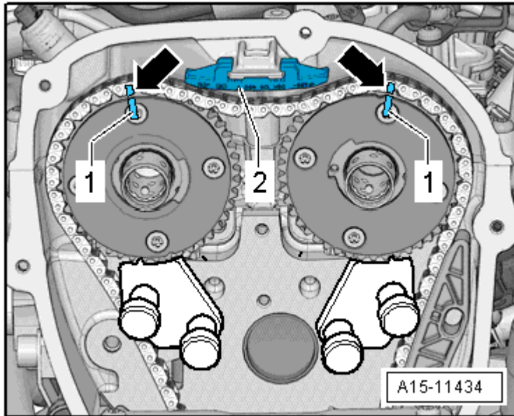
Fig. 92: Position Markings On Chain Links
