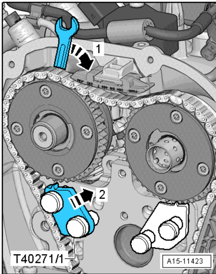
Fig. 118: Attach T40271/1 To Cylinder Head
