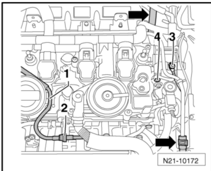
Fig. 99: Identifying Vacuum Line -1-, Ground Wire -3- And Bolt -4-
