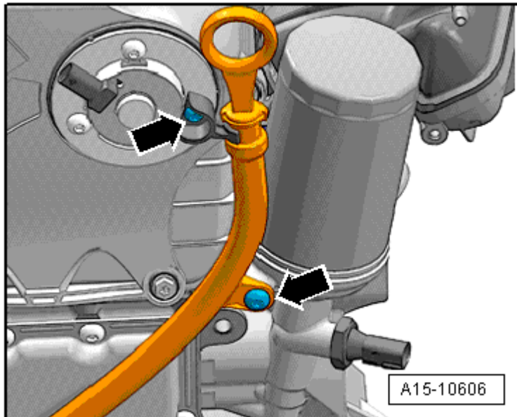
Fig. 176: Identifying Oil Dipstick Guide Tube And Bolts
