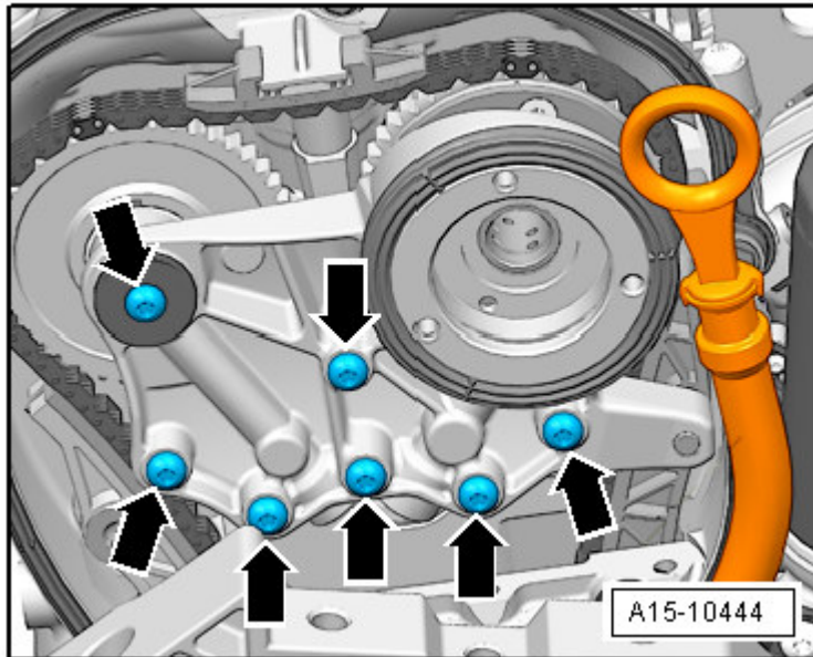
Fig. 200: Bearing Bracket Bolts
