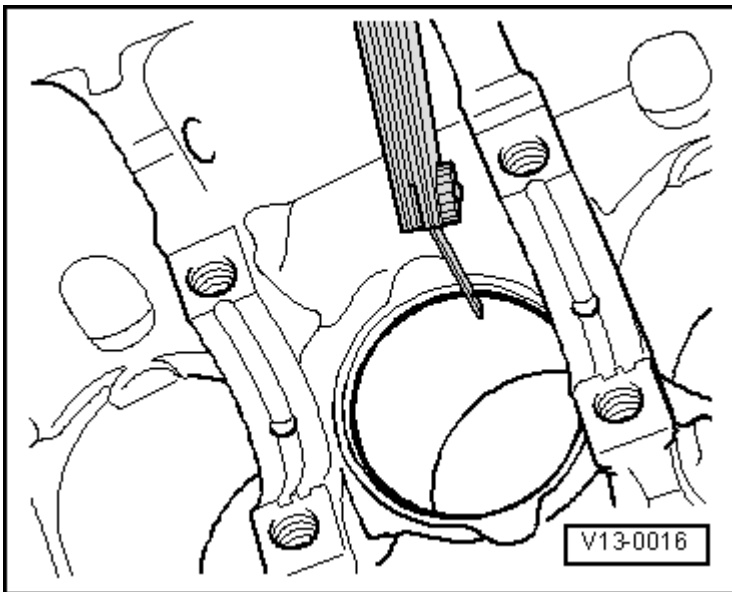
Fig. 20: Checking Piston Ring Gap Courtesy of AUDI OF AMERICA, LLC
