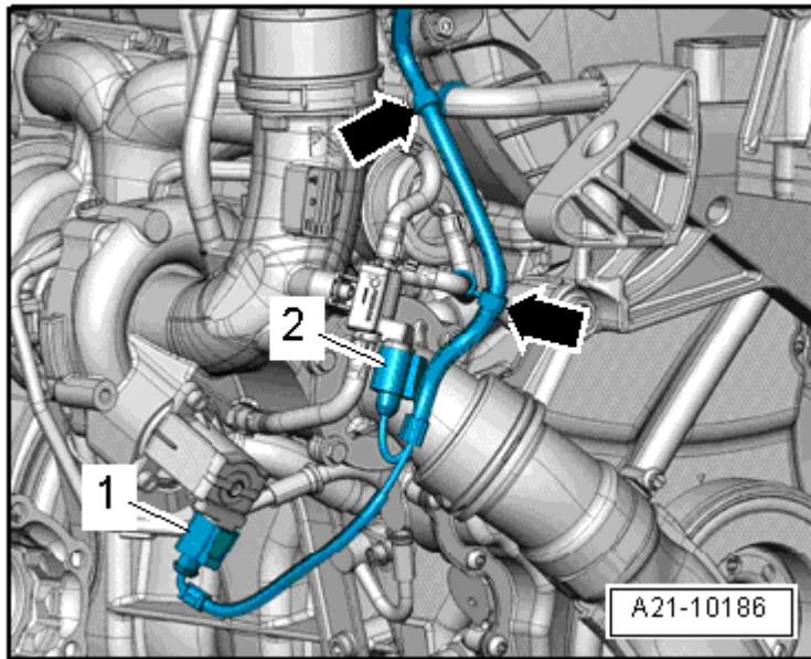
Fig. 39: Identifying Turbocharger Electrical Connectors
