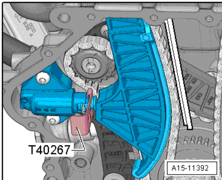
Fig. 206: Securing Chain Tensioner With T40267
