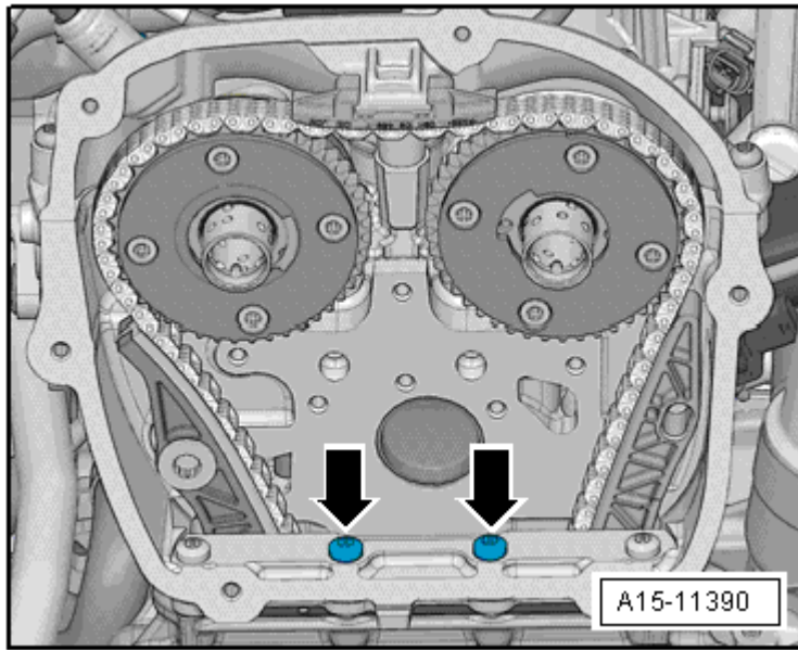
Fig. 68: Identifying Bolts
