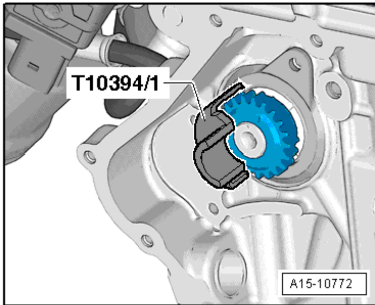
Fig. 237: Identifying Half Shell -T10394/1-
