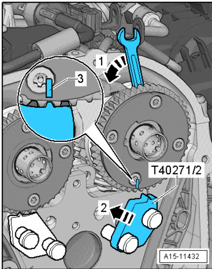
Fig. 135: Attach T40271/2 To Cylinder Head
