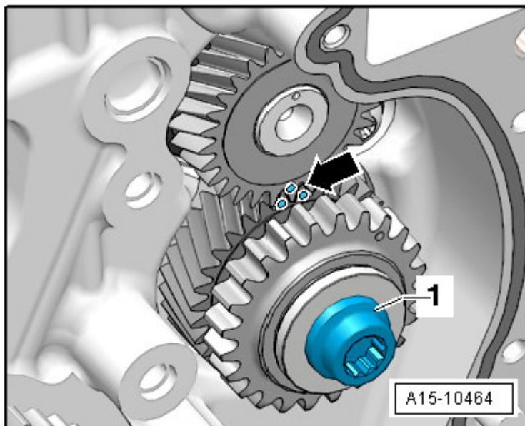
Fig. 235: Identifying Intermediate Shaft Sprocket
