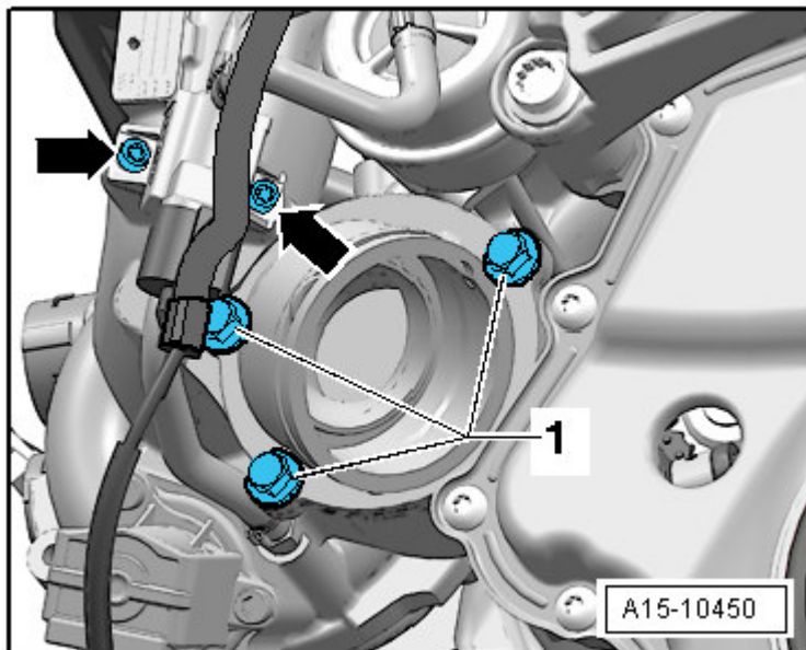
Fig. 177: Identifying Turbocharger And Supports
