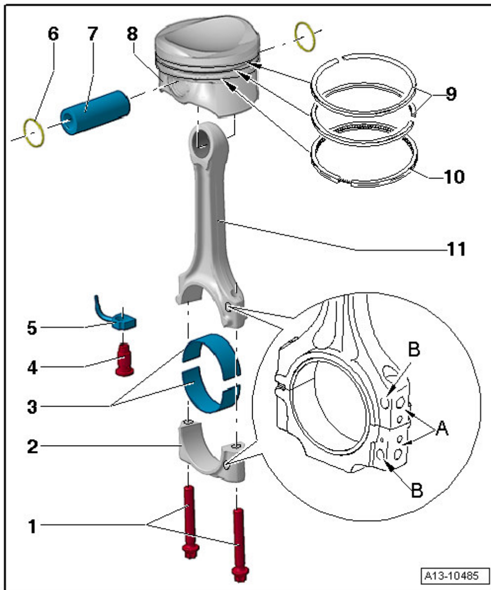
Fig. 14: Identifying Assembly Overview: Pistons And Connecting Rod Courtesy of AUDI OF AMERICA, LLC
