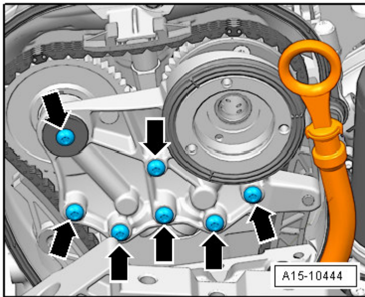
Fig. 144: Bearing Bracket Bolts
