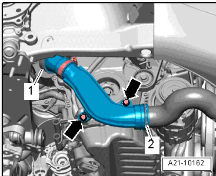
Fig. 45: Air Guide Pipe And Bolts
