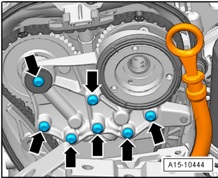
Fig. 64: Bearing Bracket Bolts
