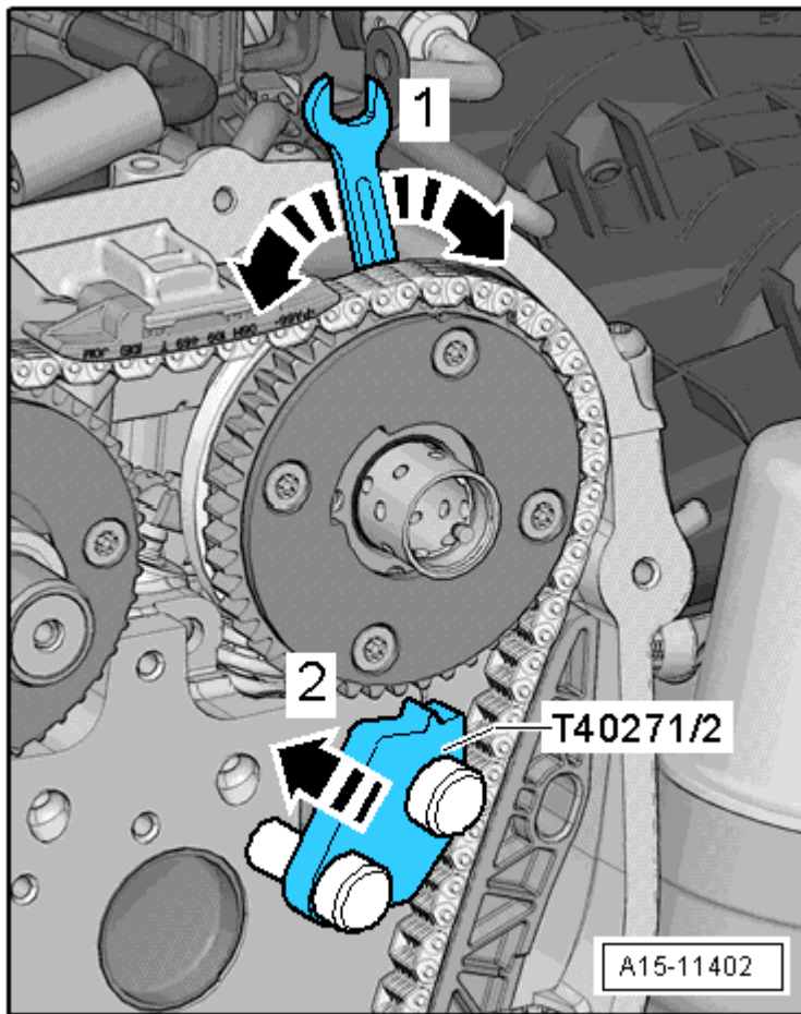
Fig. 116: Bolt Camshaft Locating Tool
