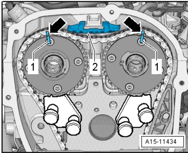
Fig. 139: Position Markings On Chain Links
