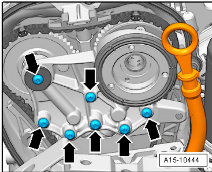
Fig. 189: Bearing Bracket Bolts
