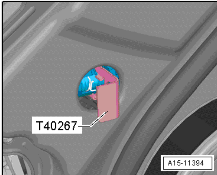
Fig. 115: Securing Chain Tensioner
