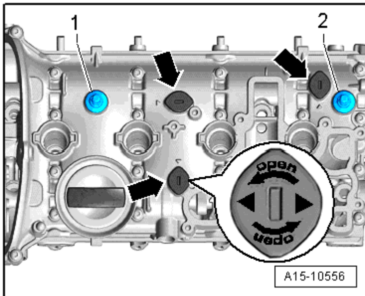
Fig. 78: Ball Head And Sealing Plug
