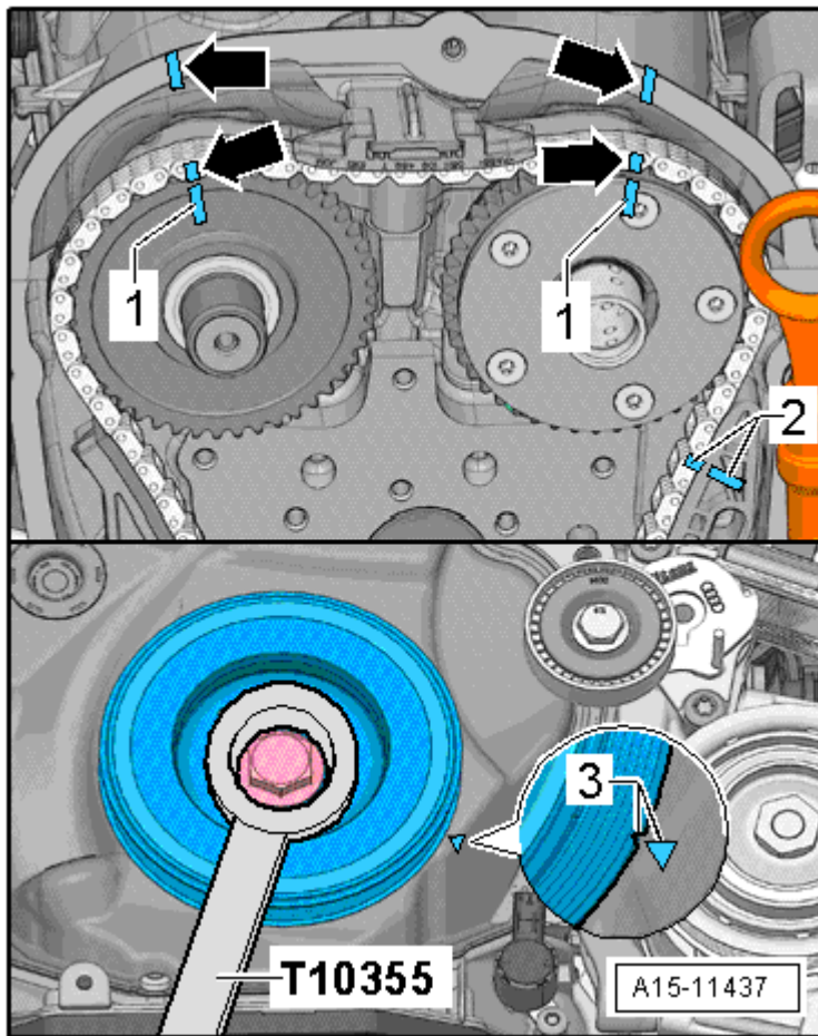
Fig. 143: Check Valve Timing
