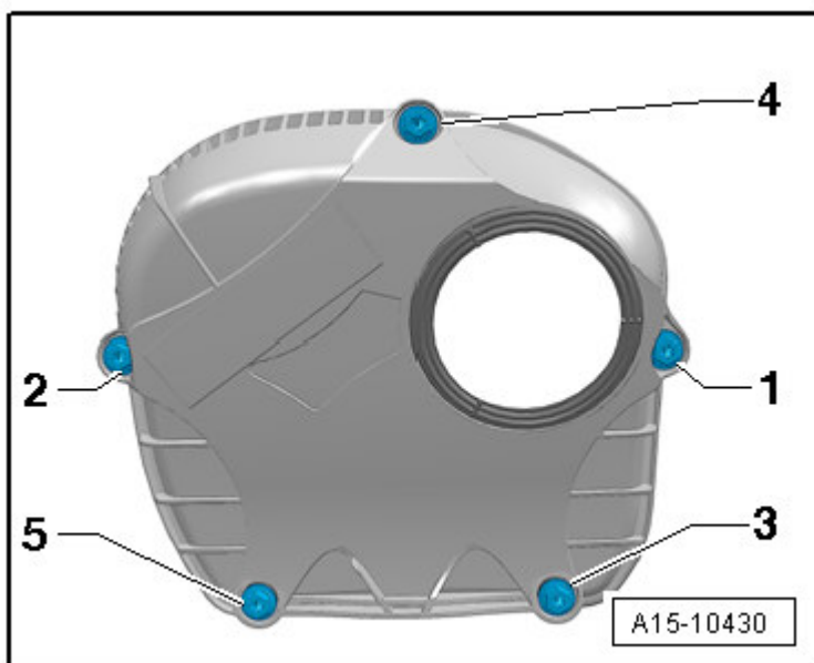
Fig. 161: Identifying Upper Timing Chain Cover - Tightening Sequence
