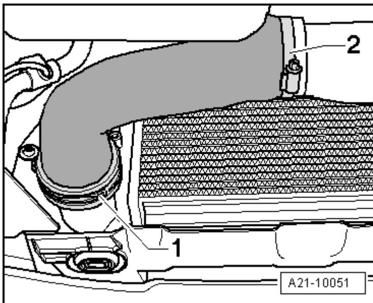
Fig. 36: Air Cooler Air Duct
