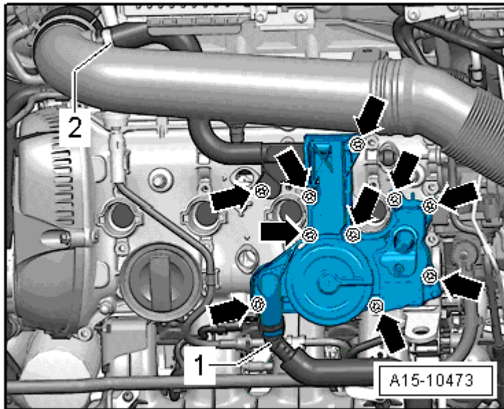
Fig. 45: Crankcase Ventilation, Tightening Sequence
